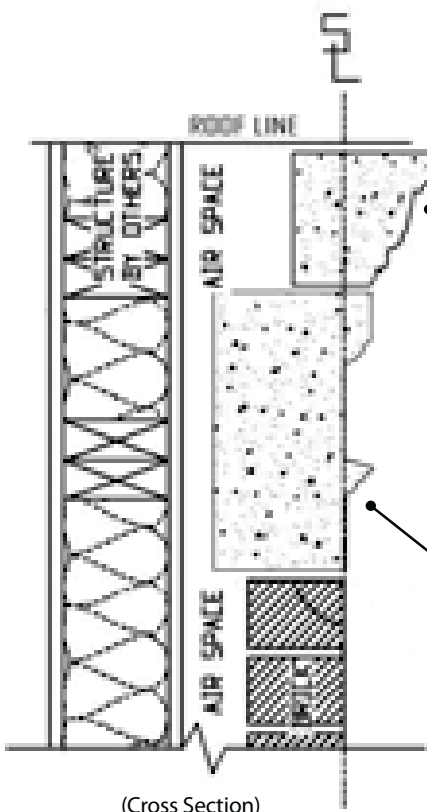
(Cross Section)
