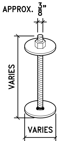
2 BISCUIT ANCHOR DETAIL GALV. OR BETTER
