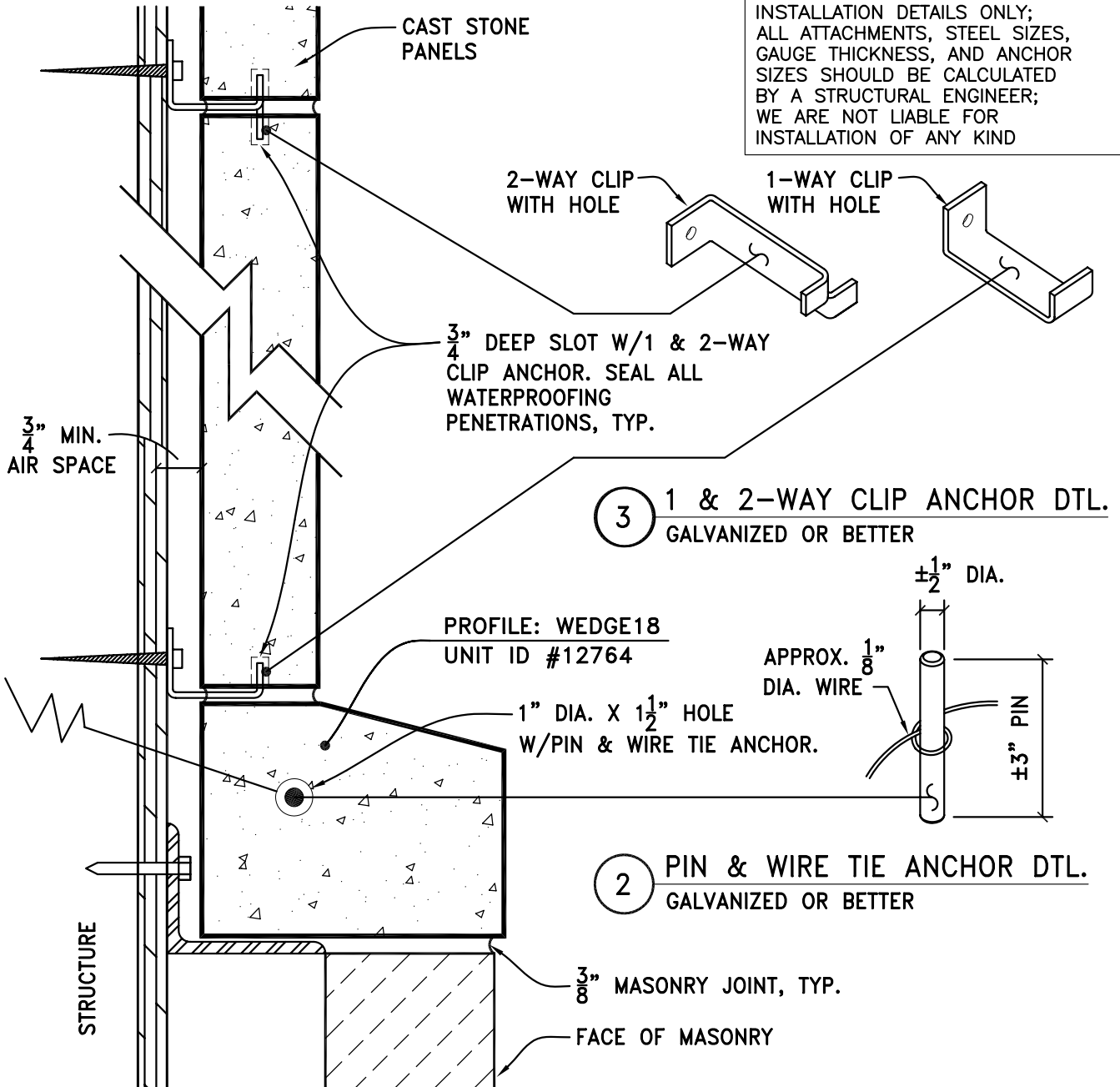
1 CAST STONE PANEL & WATER TABLE ATTACHMENT TO MASONRY VENEER WITH 1 & 2-WAY CLIP ANCHOR AND PIN & WIRE TIE ANCHOR
