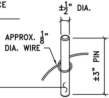
2 PIN & WIRE TIE DETAIL GALVANIZED OR BETTER
