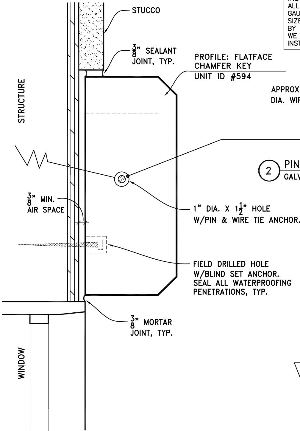
1 CAST STONE LINTEL ATTACHMENT AT STUCCO WITH PIN & WIRE TIE AND BLIND SET ANCHORS
