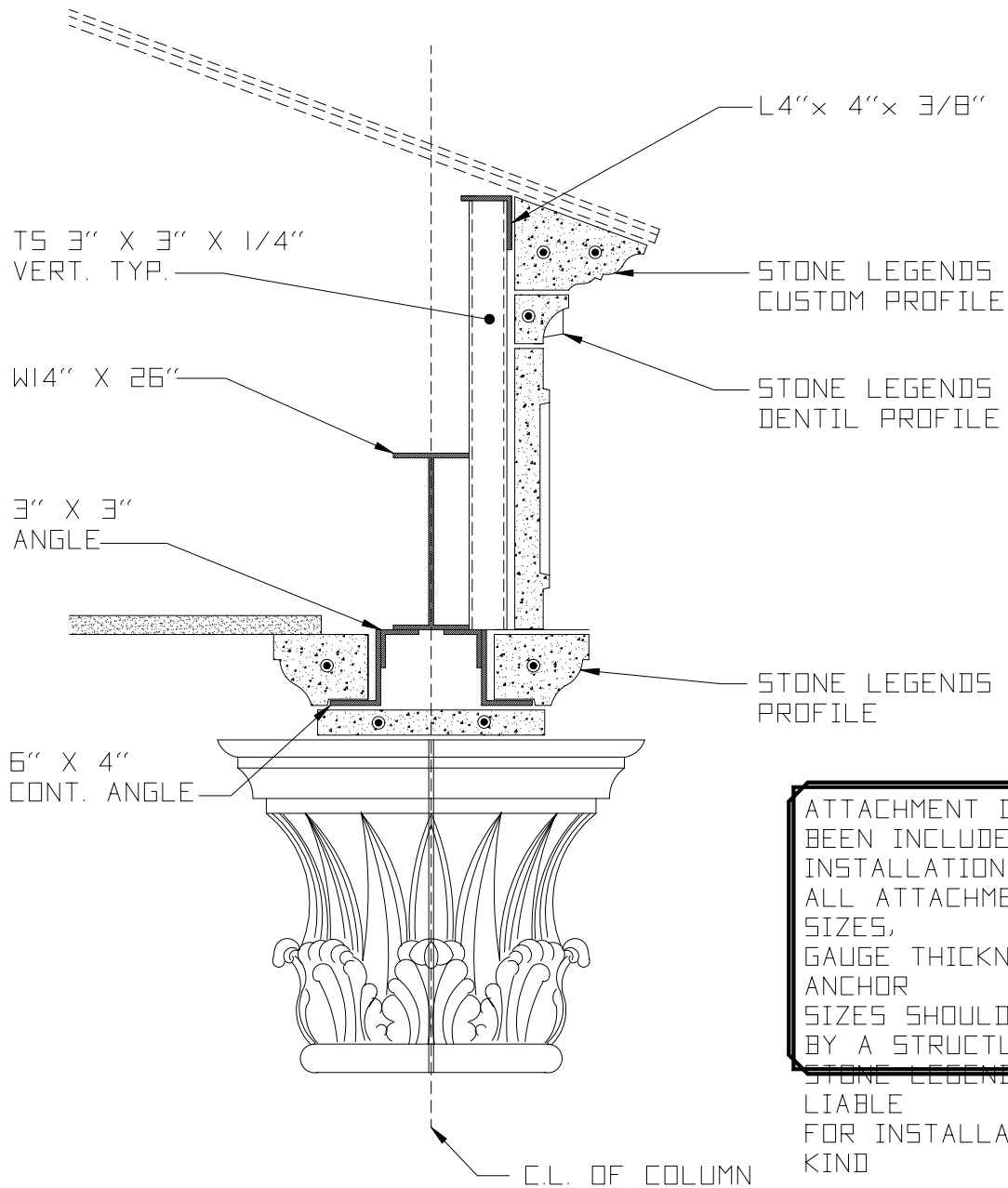
① ATTACHMENT OF ENTABLATURE & SOFFIT TO STRUCTURAL STEEL WITH LINTEL & STRAP & WIRE
