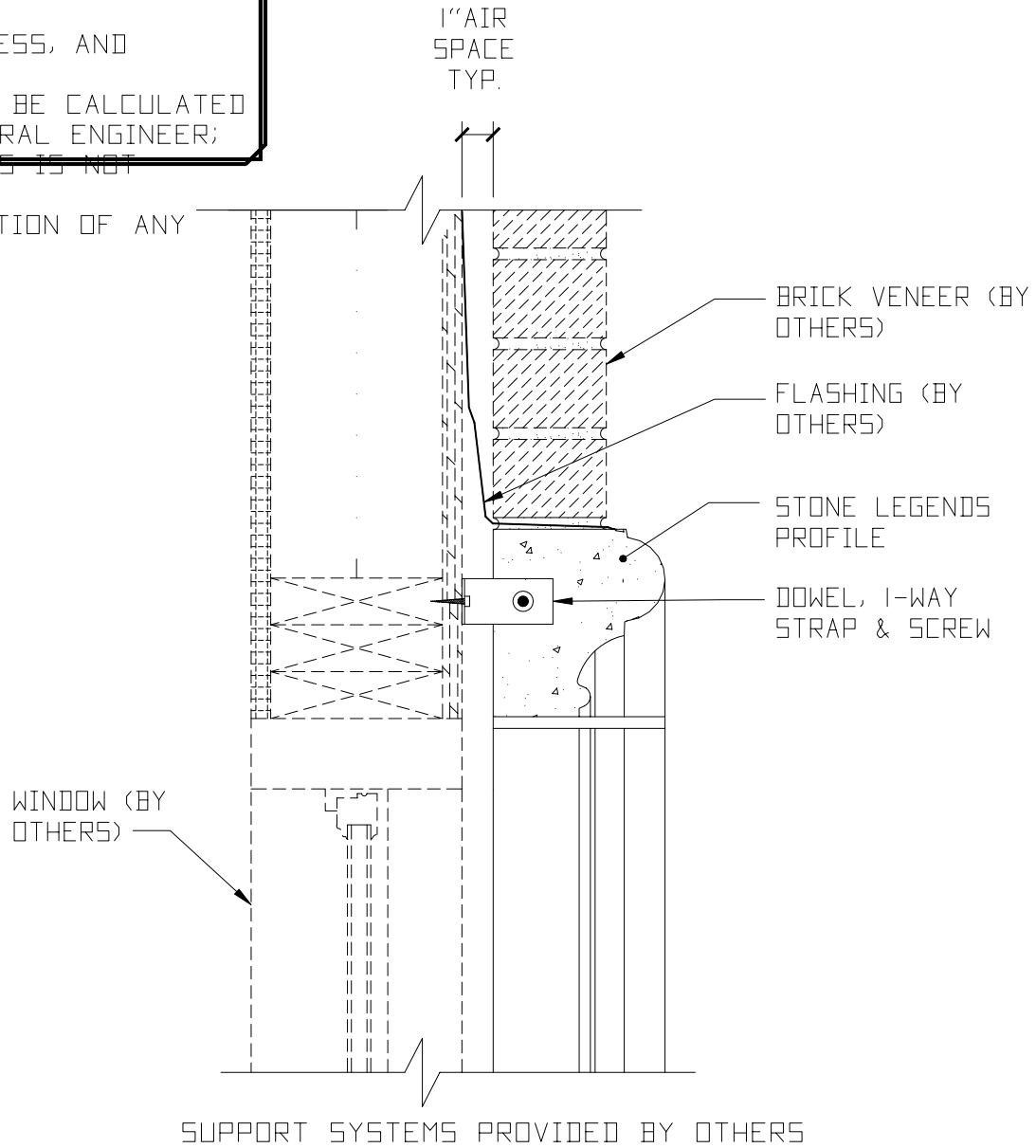
① ATTACHMENT OF HEADER TO BRICK VENEER WITH FLASHING & DOWEL & 1-WAY STRAP & SCREW
