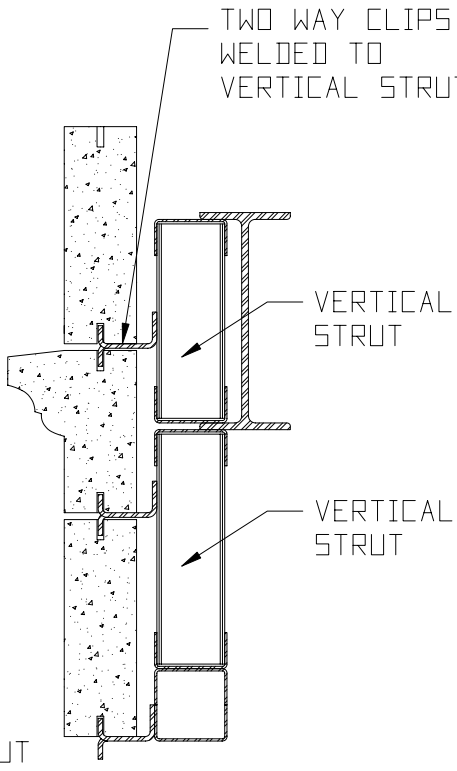
CROSS SECTION THROUGH STRUCTURE
