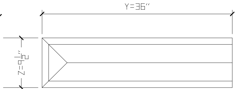
2 TOP VIEW FINISHED END QTY: _____
