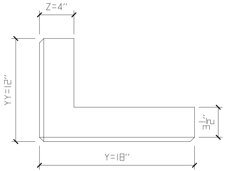
③ TOP VIEW
