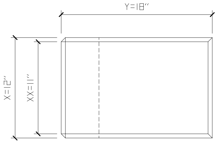
① FRONT VIEW CHAMFER1
