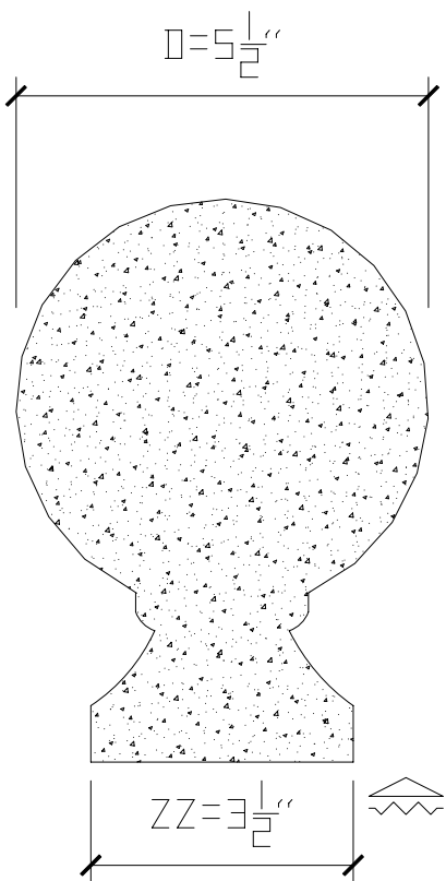
② VERTICAL SECTION
