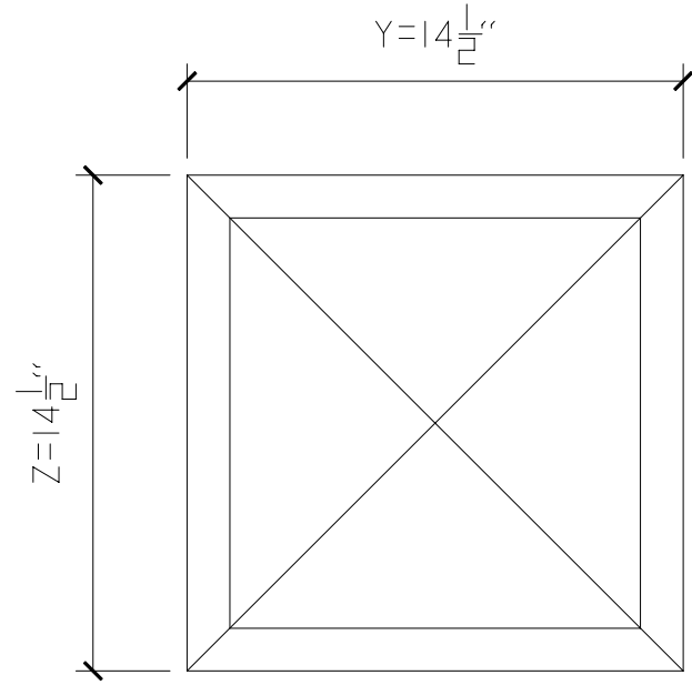
3 TOP VIEW
