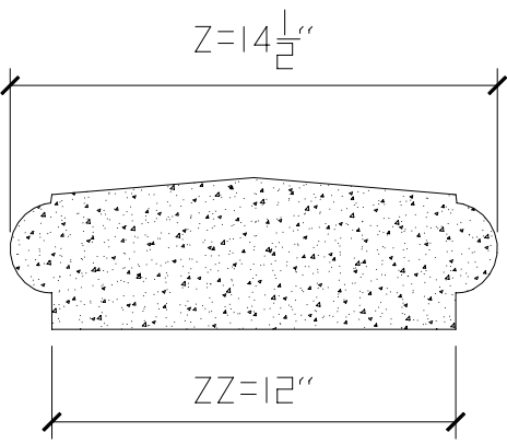
2 VERTICAL SECTION
