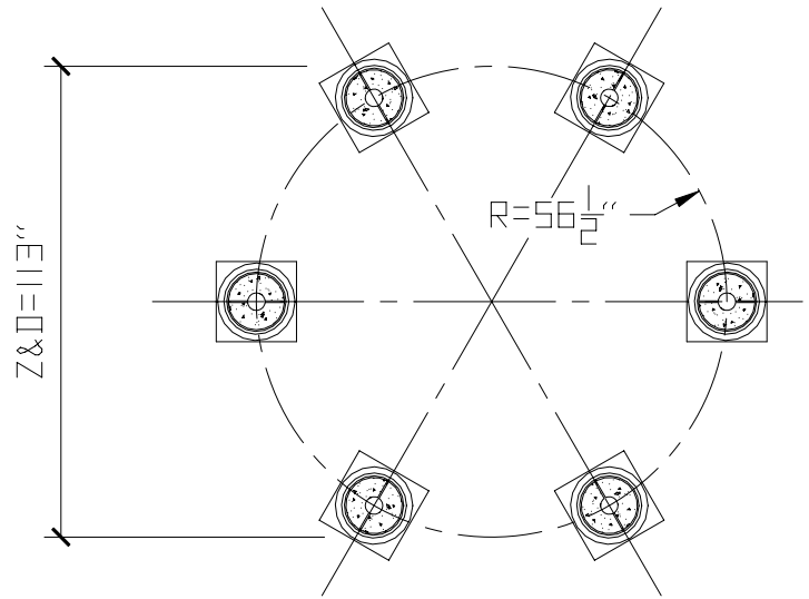
3 HORIZONTAL SECTION
