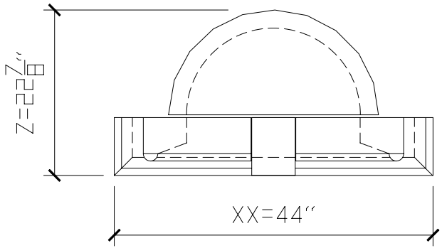
3 TOP VIEW
