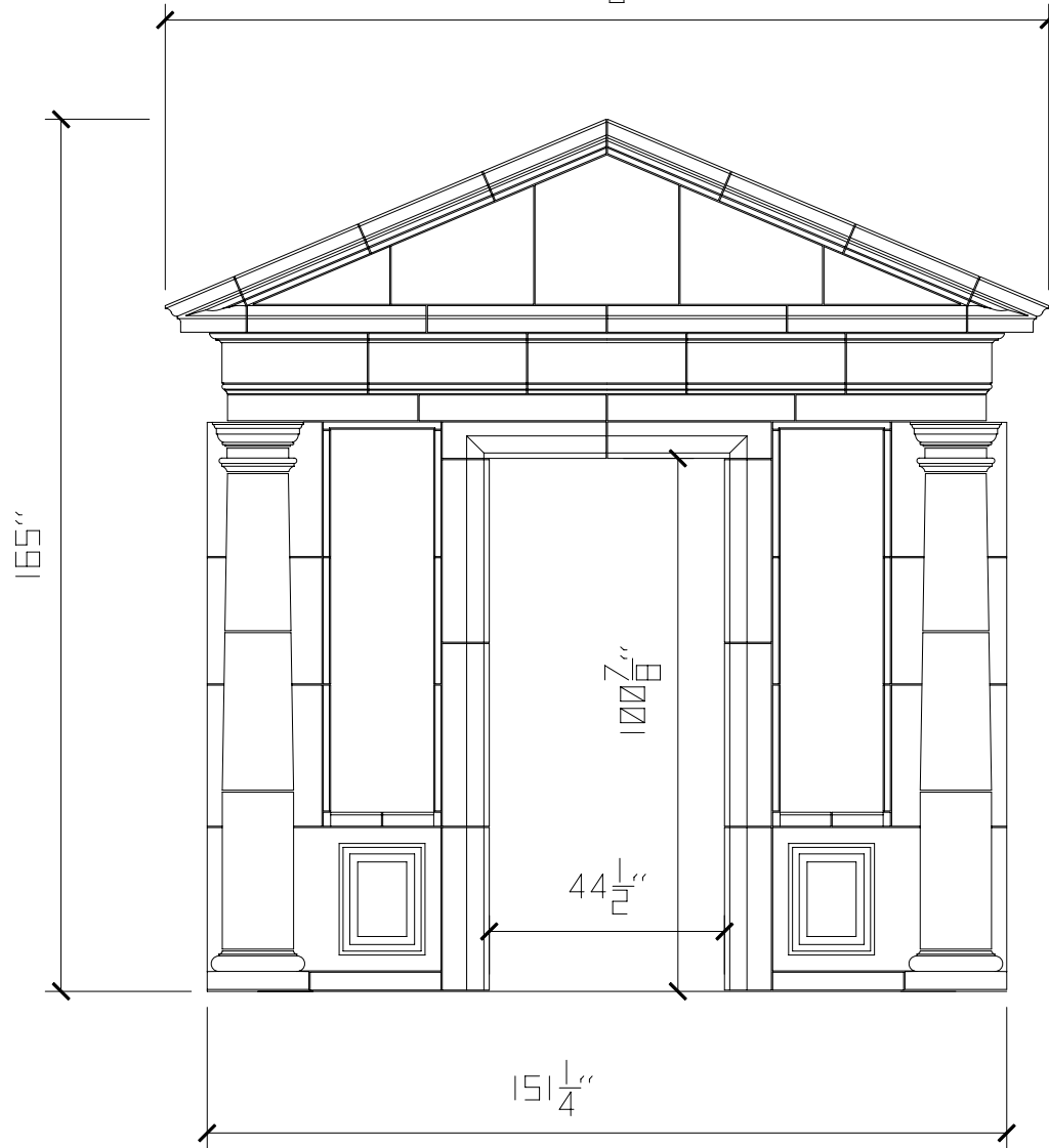
① FRONT VIEW
