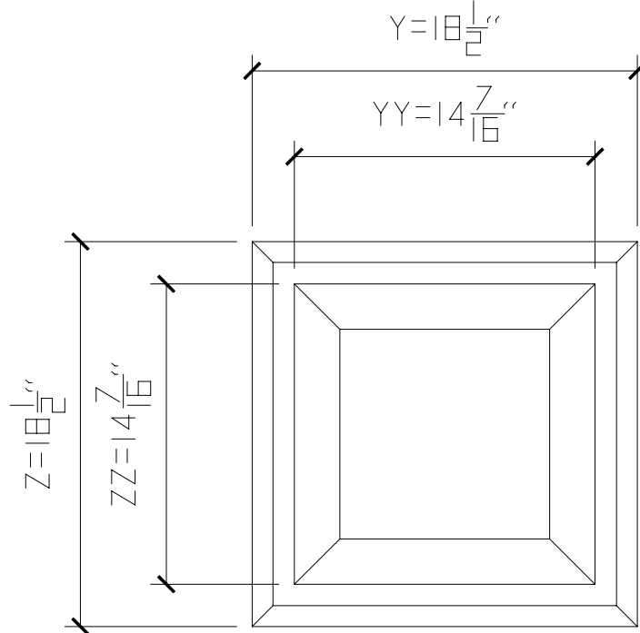
③ TOP VIEW
