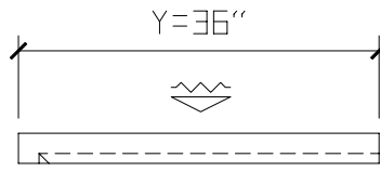
④ TOP VIEW QTY COPE INSIDE LEFT
