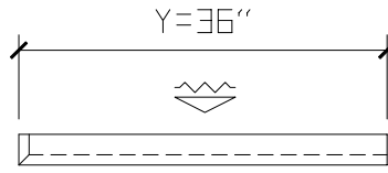
② TOP VIEW QTY COPE OUTSIDE LEFT
