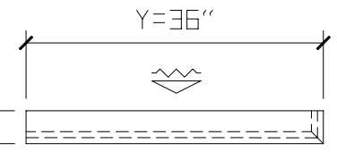
3 TOP VIEW QTY COPE OUTSIDE RIGHT
