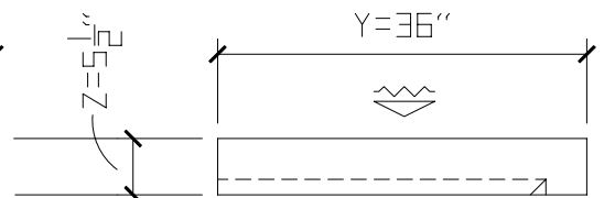
5 TOP VIEW QTY COPE INSIDE RIGHT
