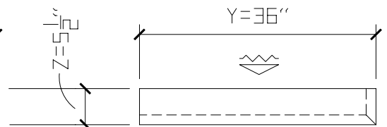
3 TOP VIEW QTY COPE OUTSIDE RIGHT
