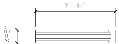
⑦ FRONT VIEW COPE INSIDE RIGHT
