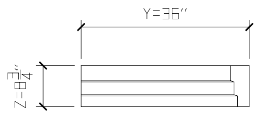
7 FRONT VIEW COPE INSIDE RIGHT
