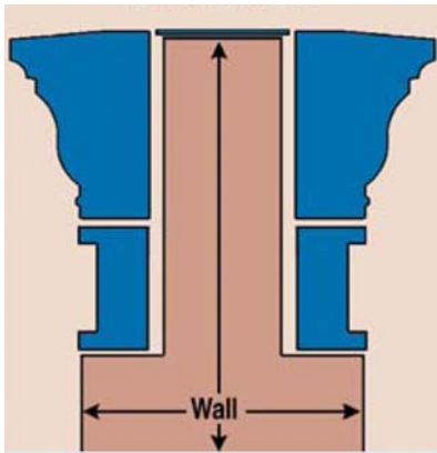
Mortar Filled
