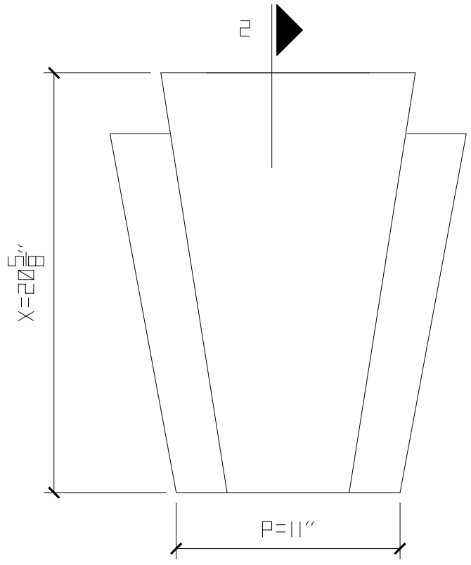
① FRONT VIEW
