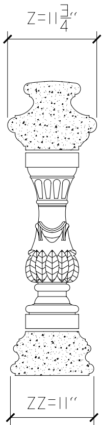
2 VERTICAL SECTION
