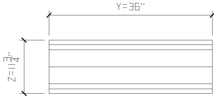
3 TOP VIEW
