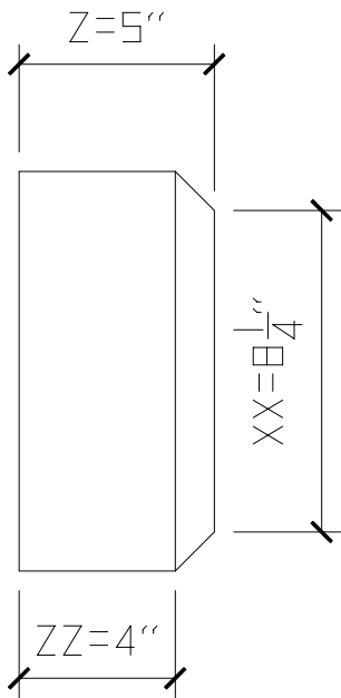
2 SIDE VIEW
