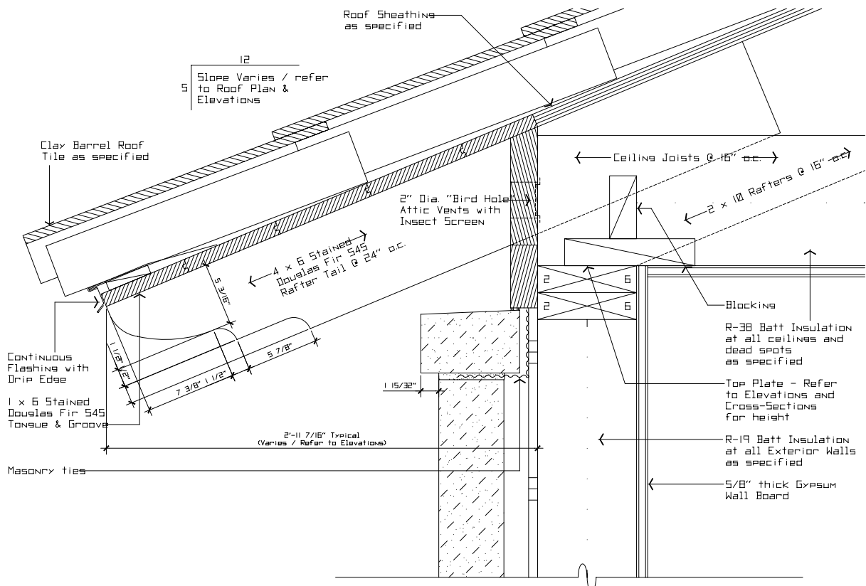
2 Typical Eave Detail with Stone Veneer
