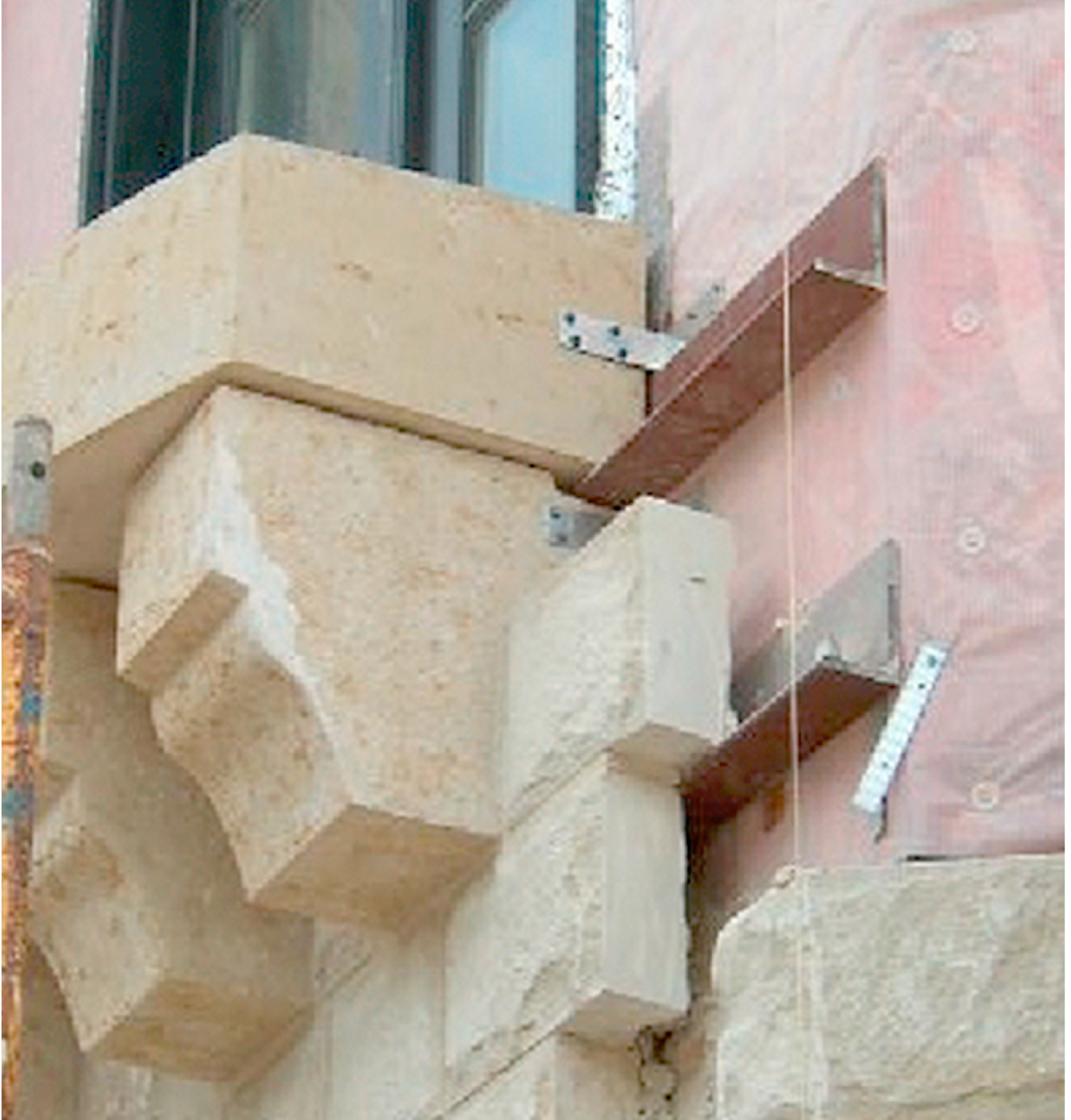
L-clips & tapcon screws secure the stone in position. Steel beams support & distribute the weight.
