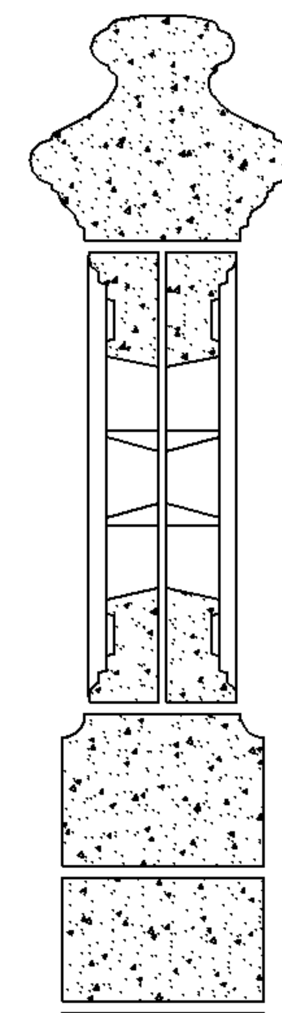
Cove2 Baserail
