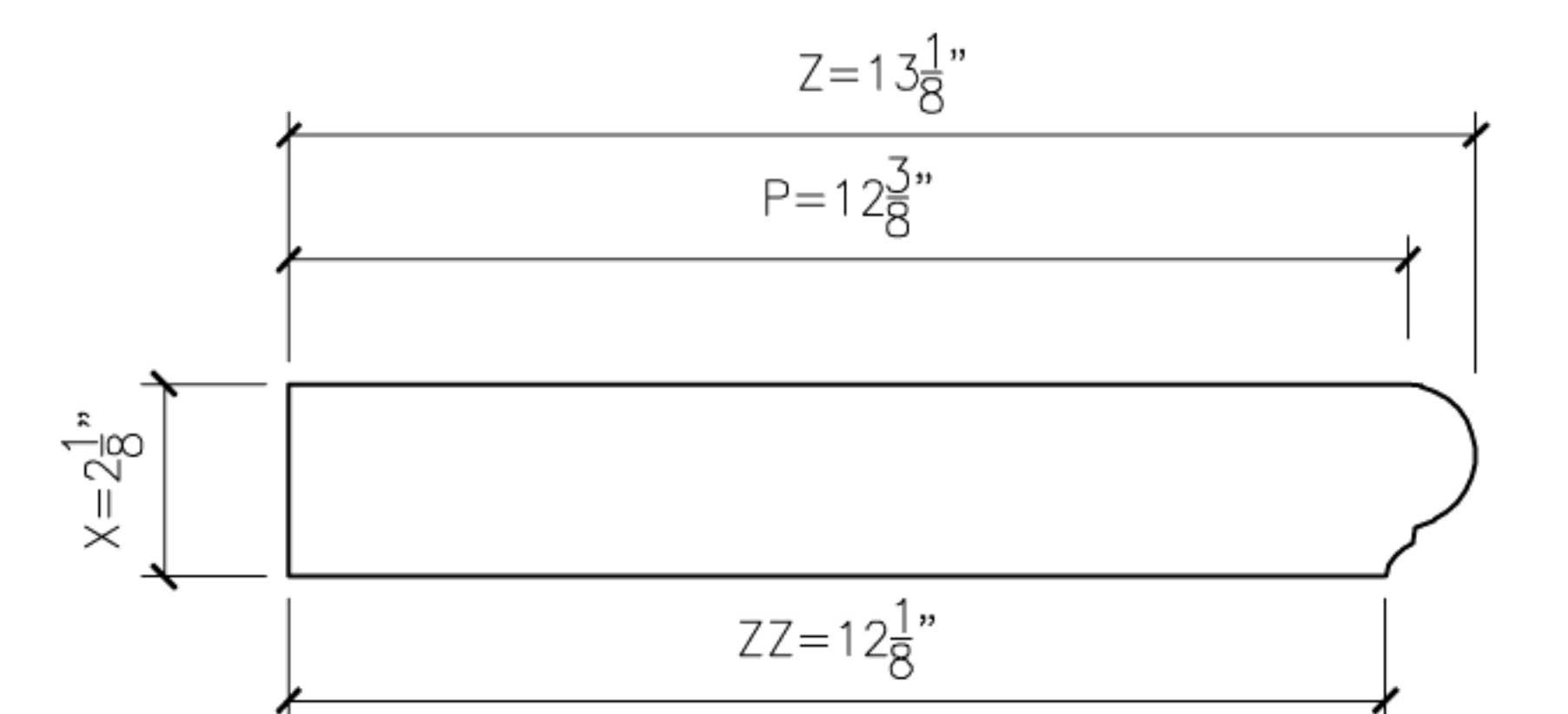
13 BOLSON13 PROFILE SECTION
