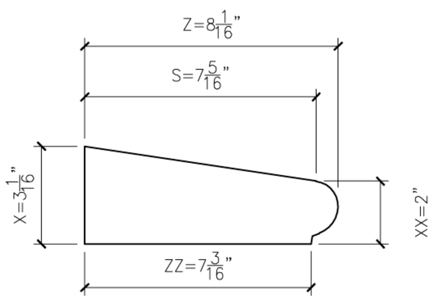
11 BULLNOSE RISE5 PROFILE SECTION
