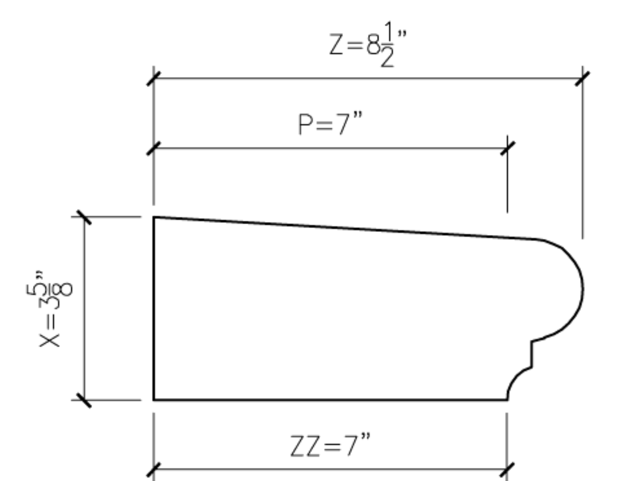
6 BOLSON6 PROFILE SECTION
