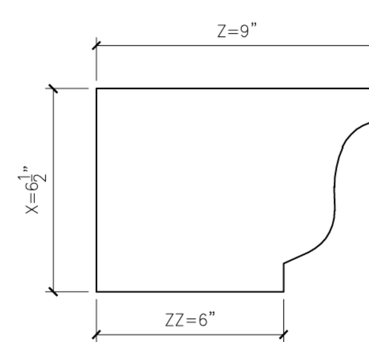
16A OGEE16A PROFILE SECTION
