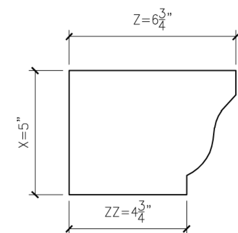
14A OGEE14A PROFILE SECTION
