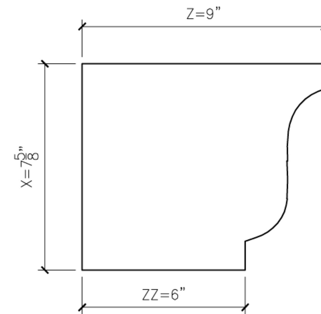
2 OGEE2 PROFILE SECTION
