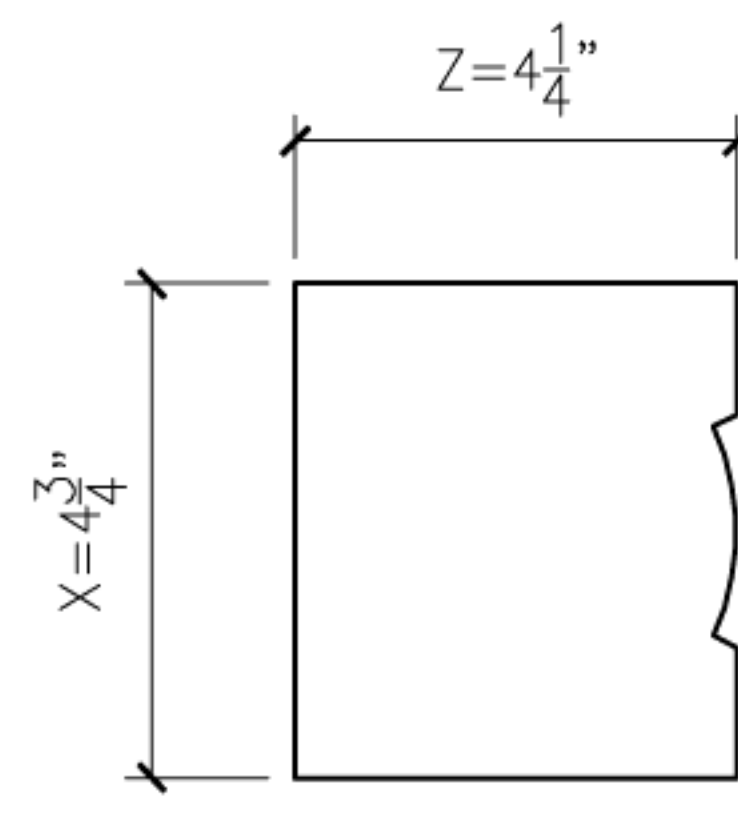
5 NAVARRO5 PROFILE SECTION
