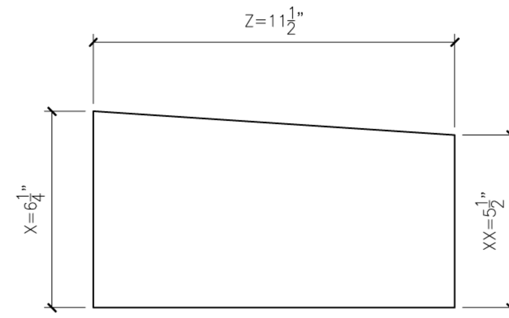
3 FLATFACE SLOPE4 PROFILE SECTION
