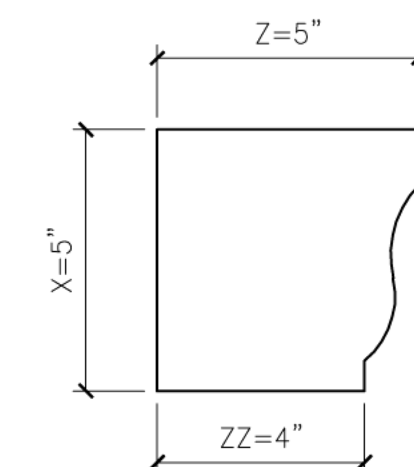
13 OGEE13 PROFILE SECTION
