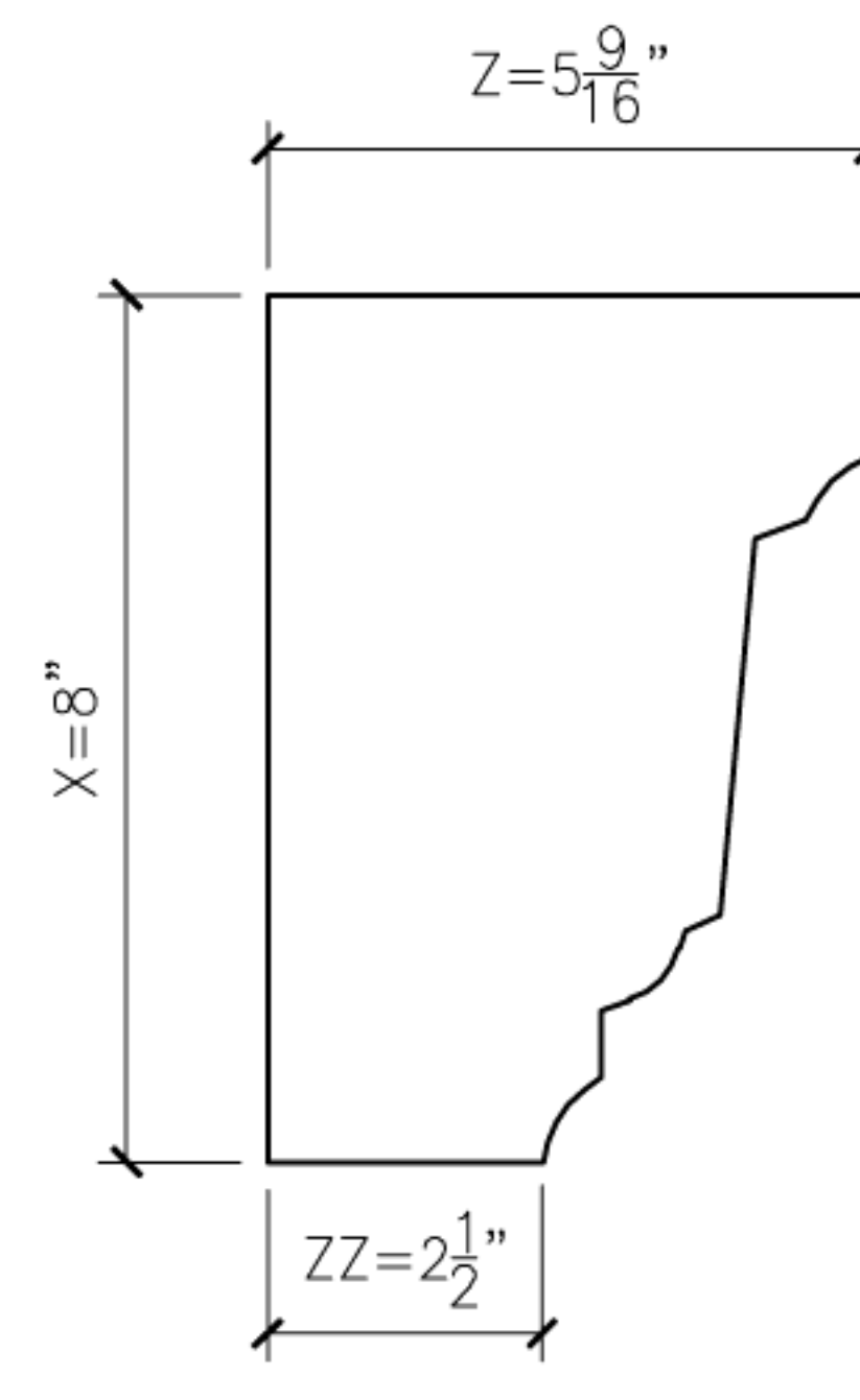
10 JAMISON10 PROFILE SECTION
