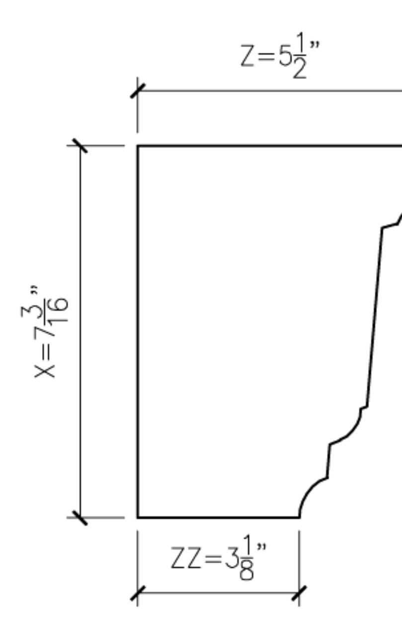
17 JAMISON17 PROFILE SECTION
