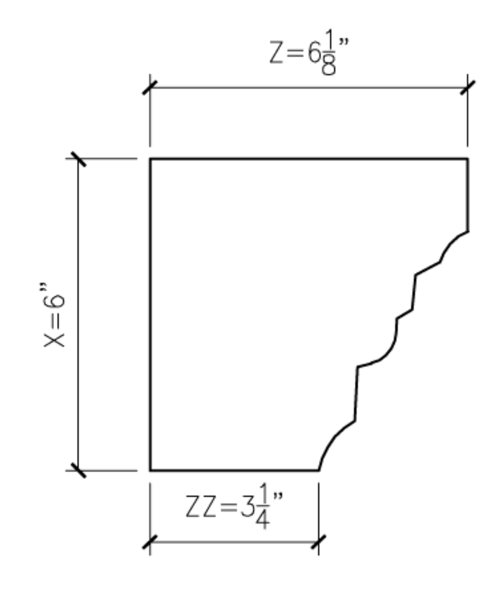
15 JAMISON15 PROFILE SECTION
