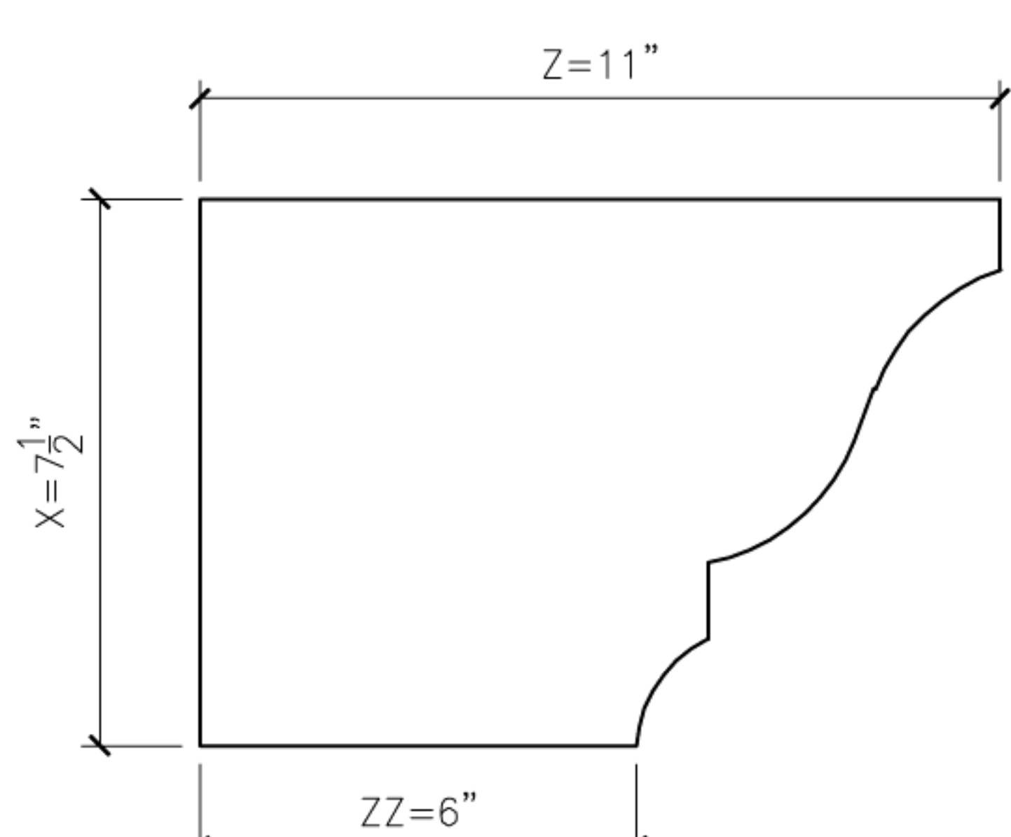
20 ORIEL20 PROFILE SECTION
