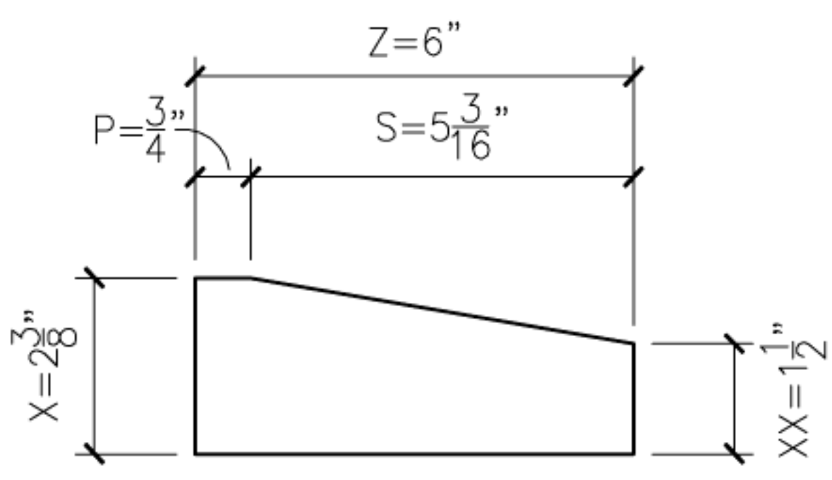
5 WEDGE5 PROFILE SECTION
