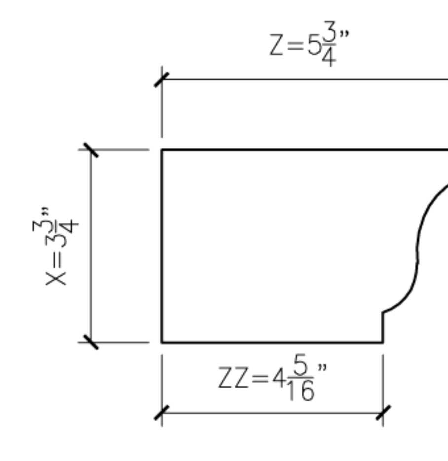
5 OGEE5 PROFILE SECTION
