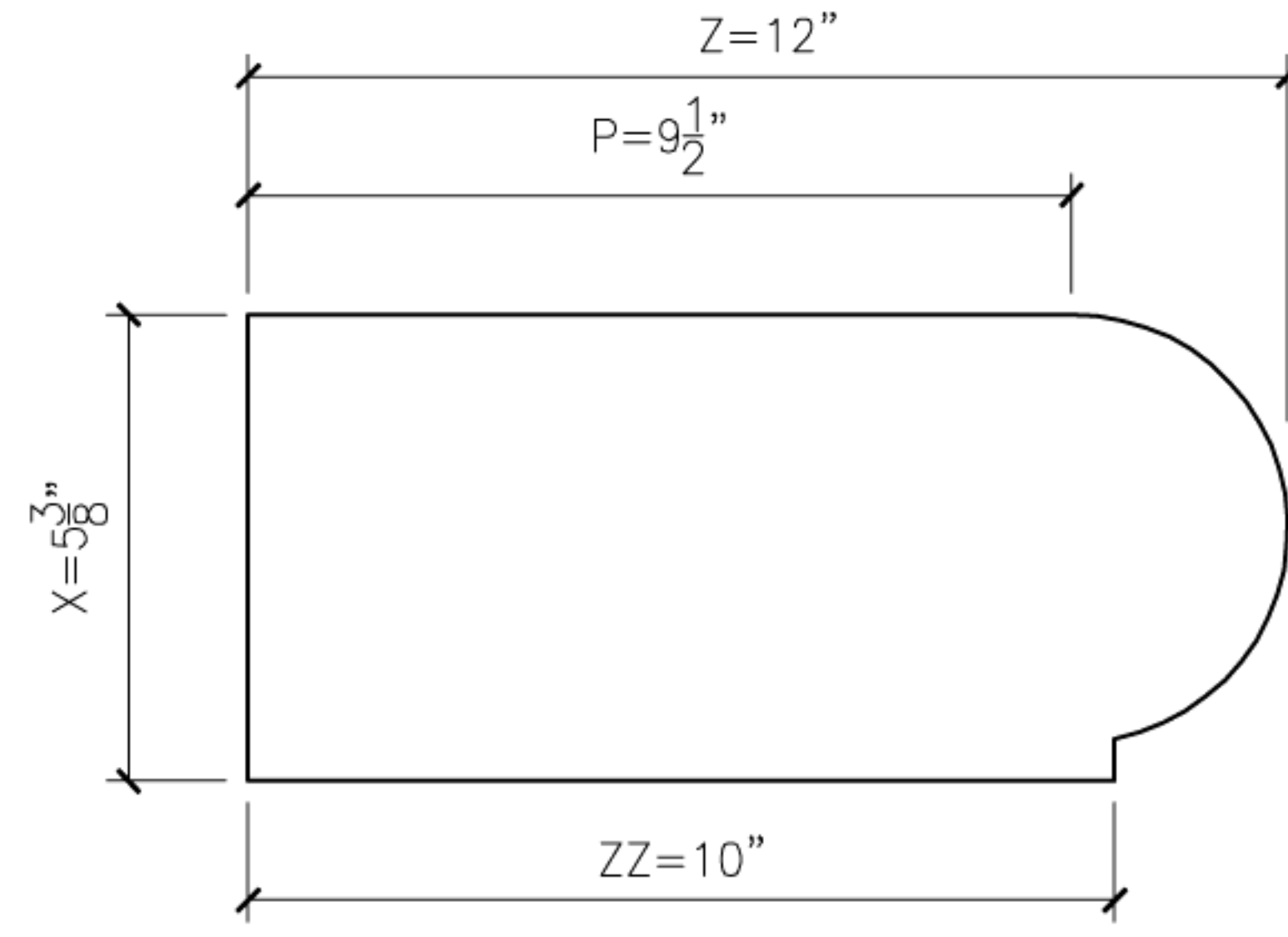
4B BULLNOSE10B PROFILE SECTION
