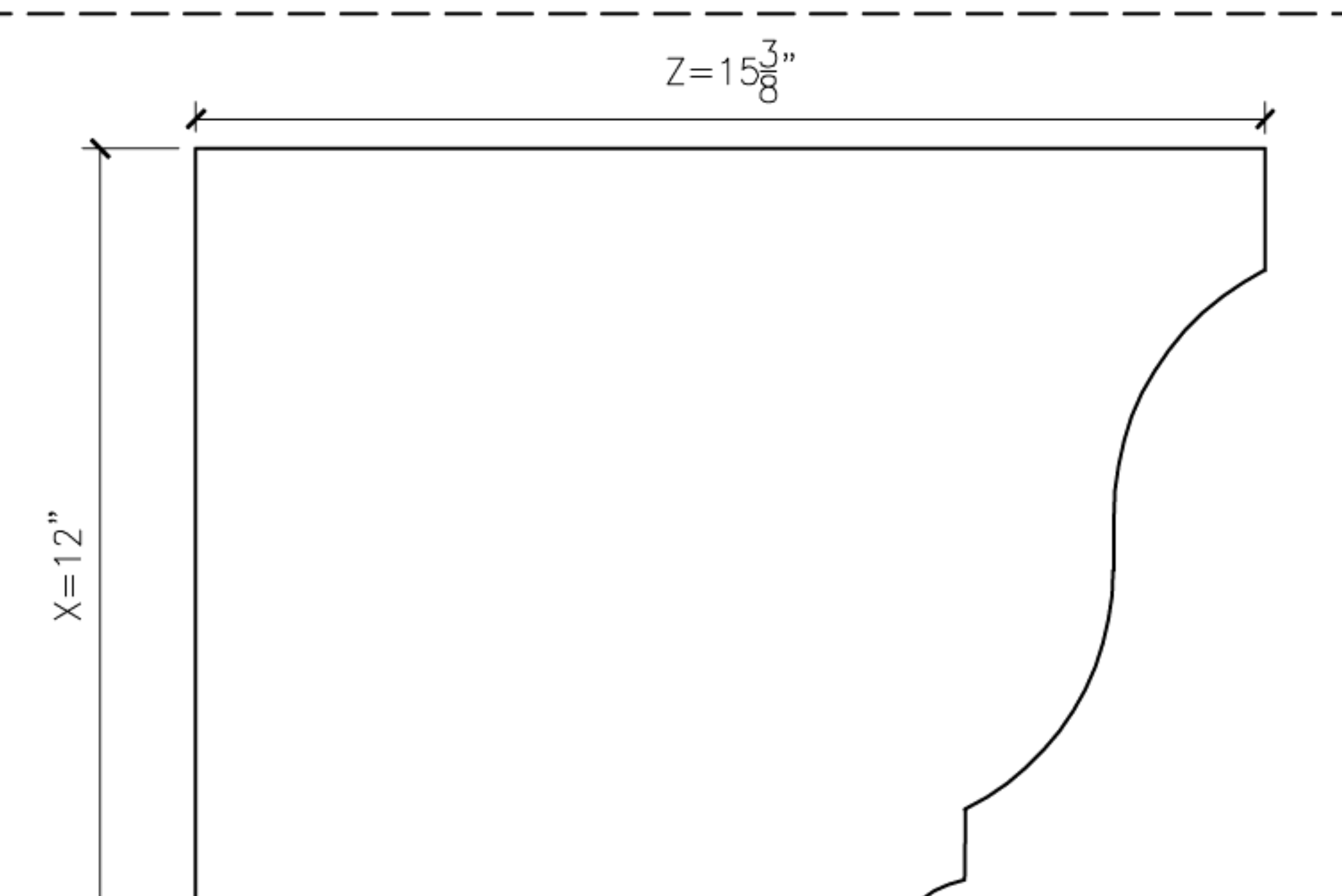
9 ORIEL9 PROFILE SECTION
