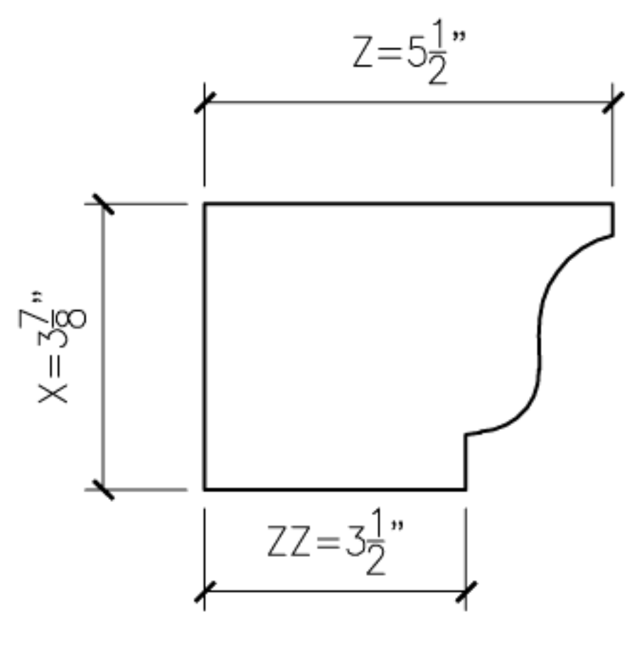
7 OGEE7 PROFILE SECTION
