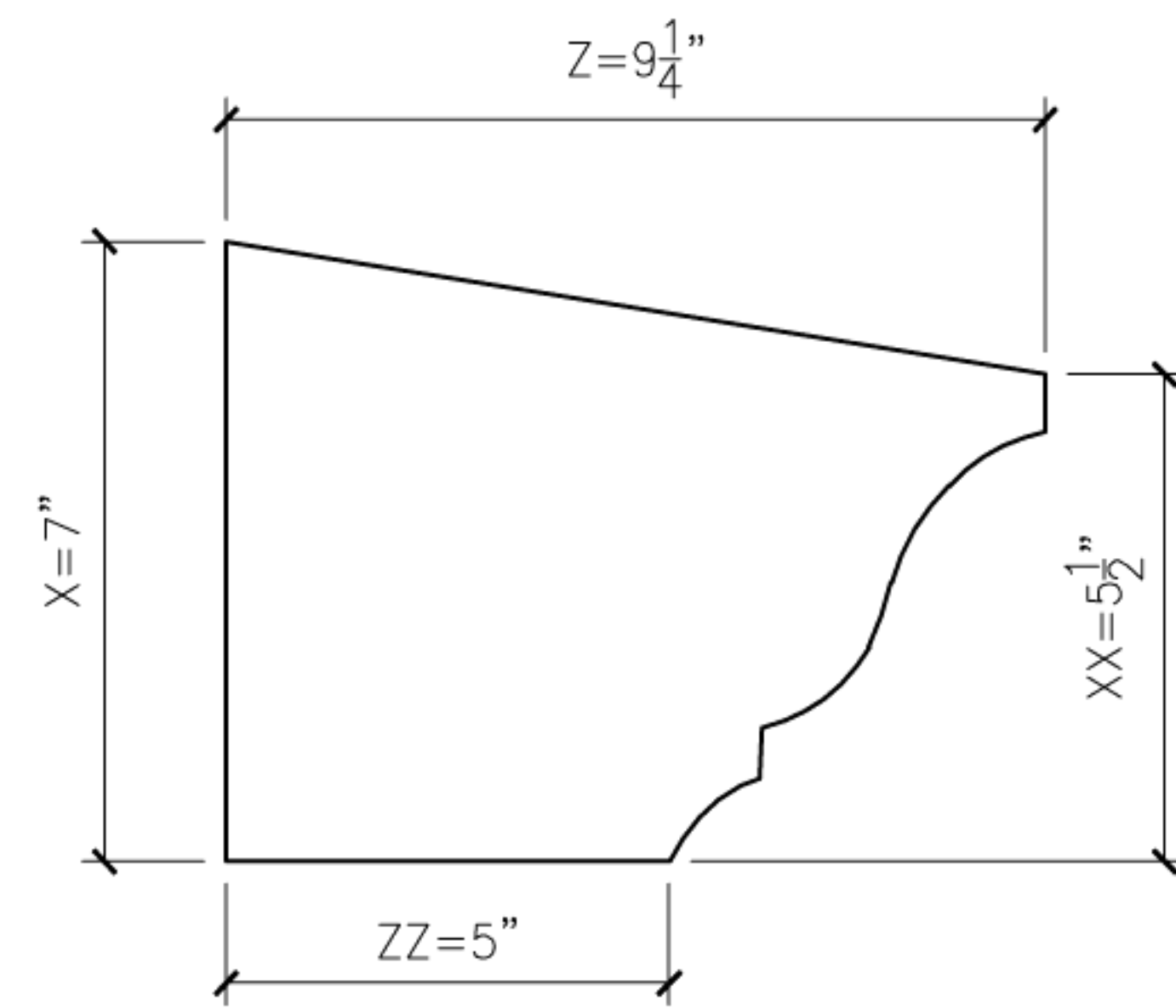
7 ORIEL7 PROFILE SECTION
