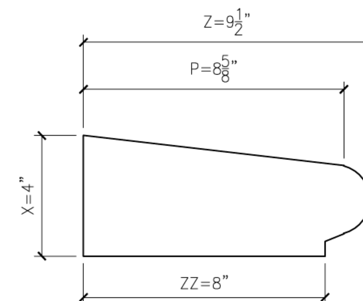
9 BULLNOSE18 PROFILE SECTION
