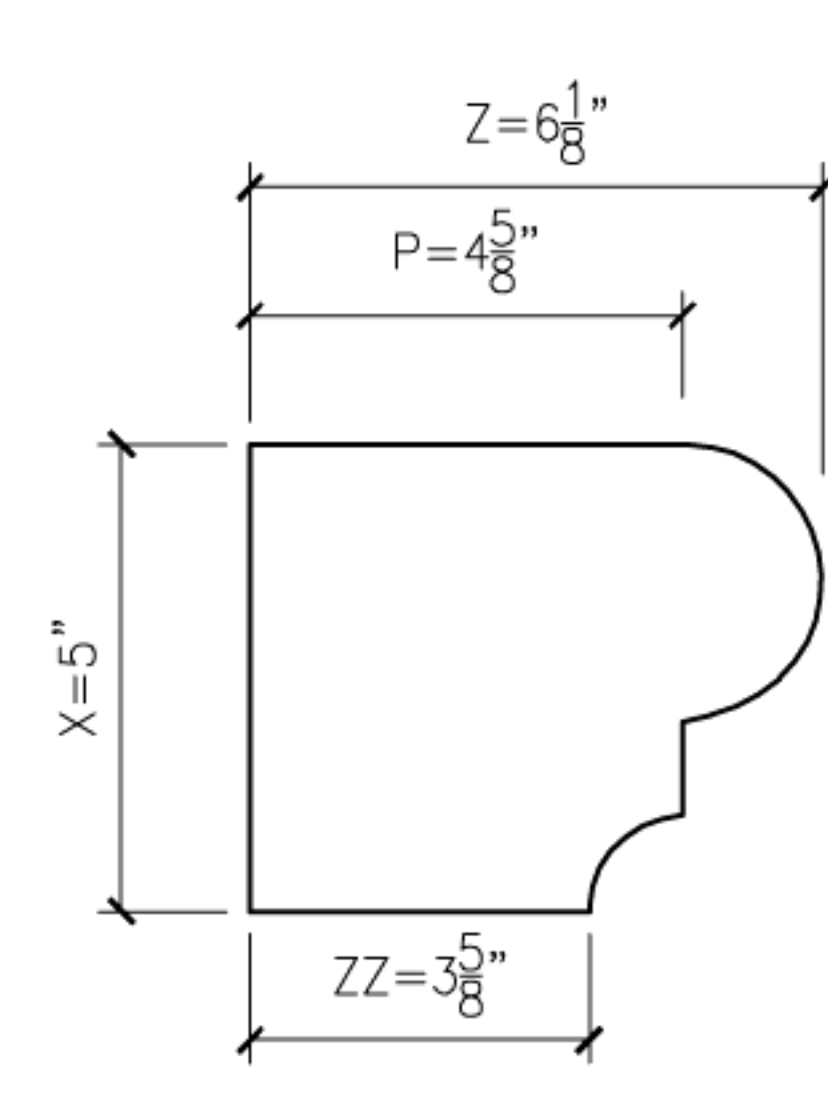
1A BOLSON1A PROFILE SECTION
