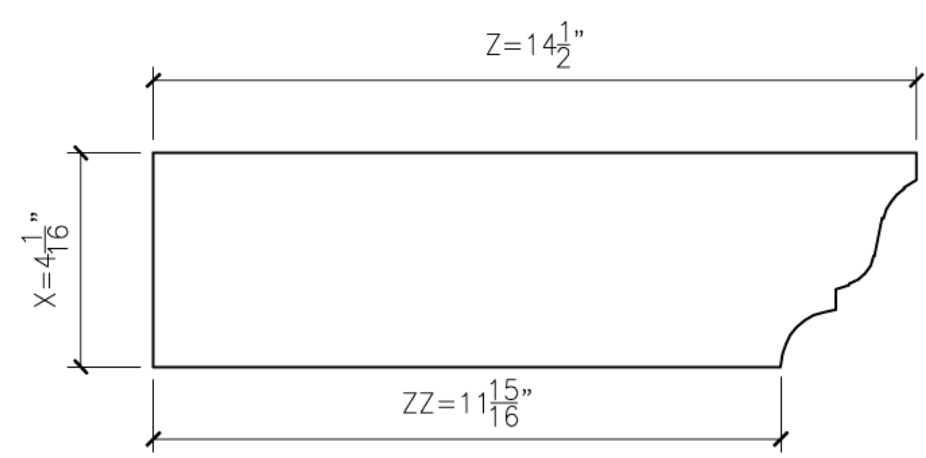
1A ORIEL1A PROFILE SECTION
