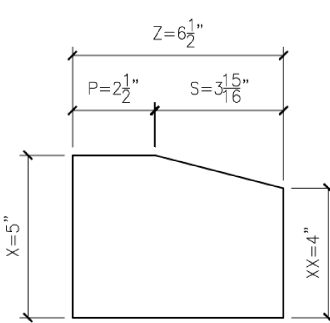
18 WEDGE18 PROFILE SECTION
