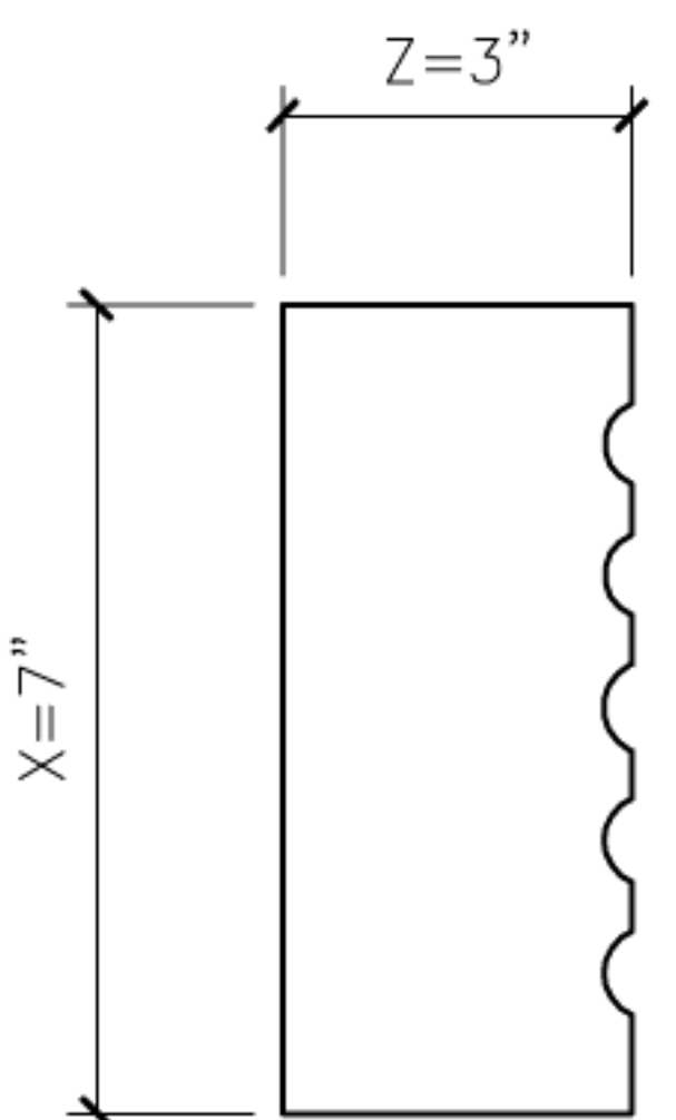
17 GEORGIAN17 PROFILE SECTION
