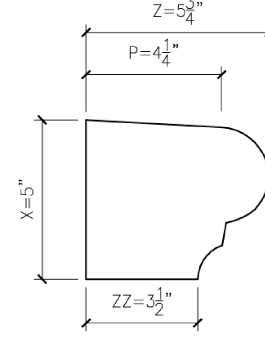
2 BOLSON2 PROFILE SECTION
