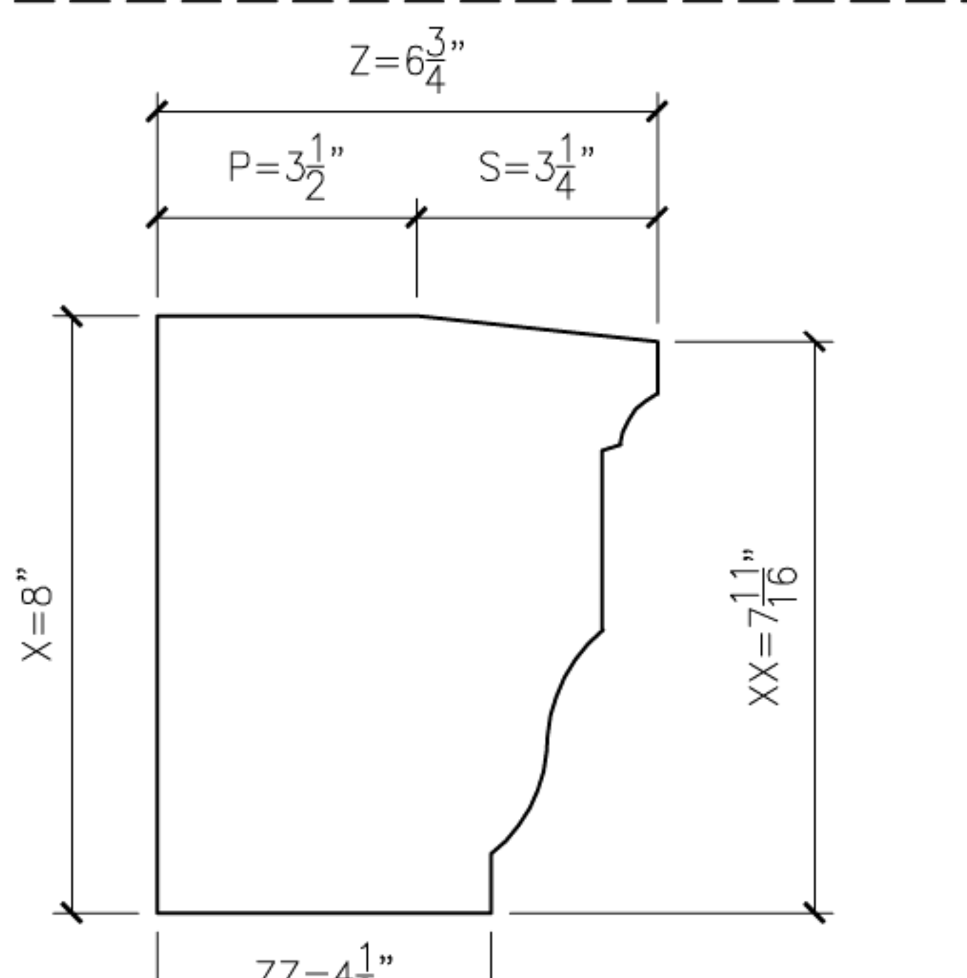
17 JUSTIN18 PROFILE SECTION
