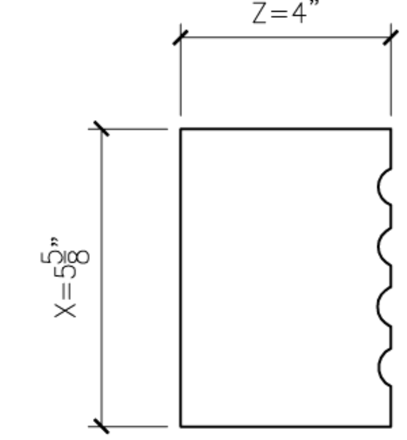
9 GEORGIAN9 PROFILE SECTION
