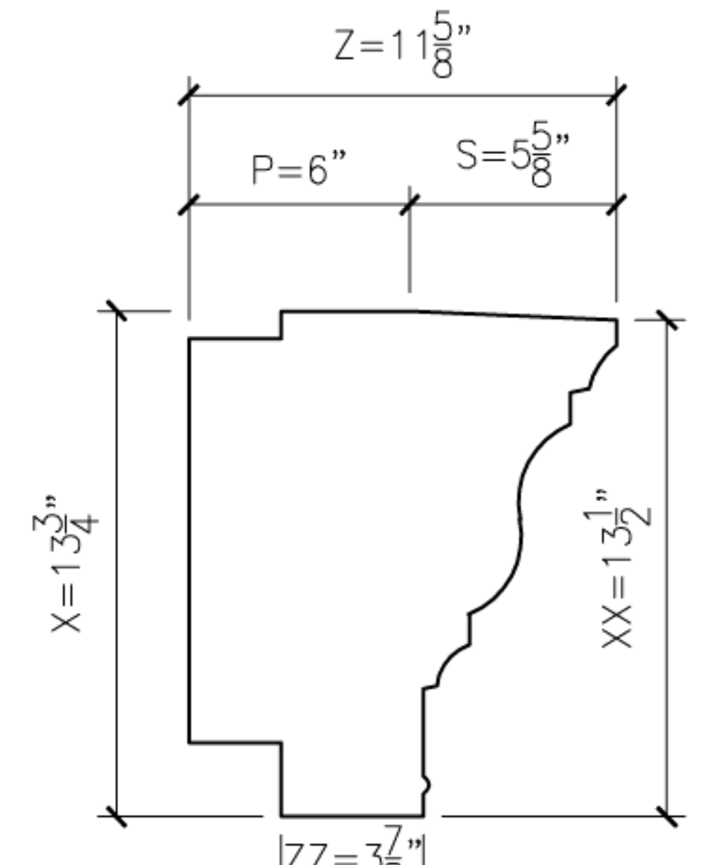
19 JUSTIN20 PROFILE SECTION
