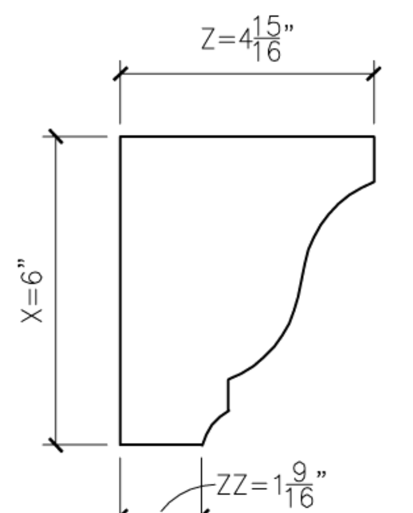
3 ORIEL3 PROFILE SECTION
