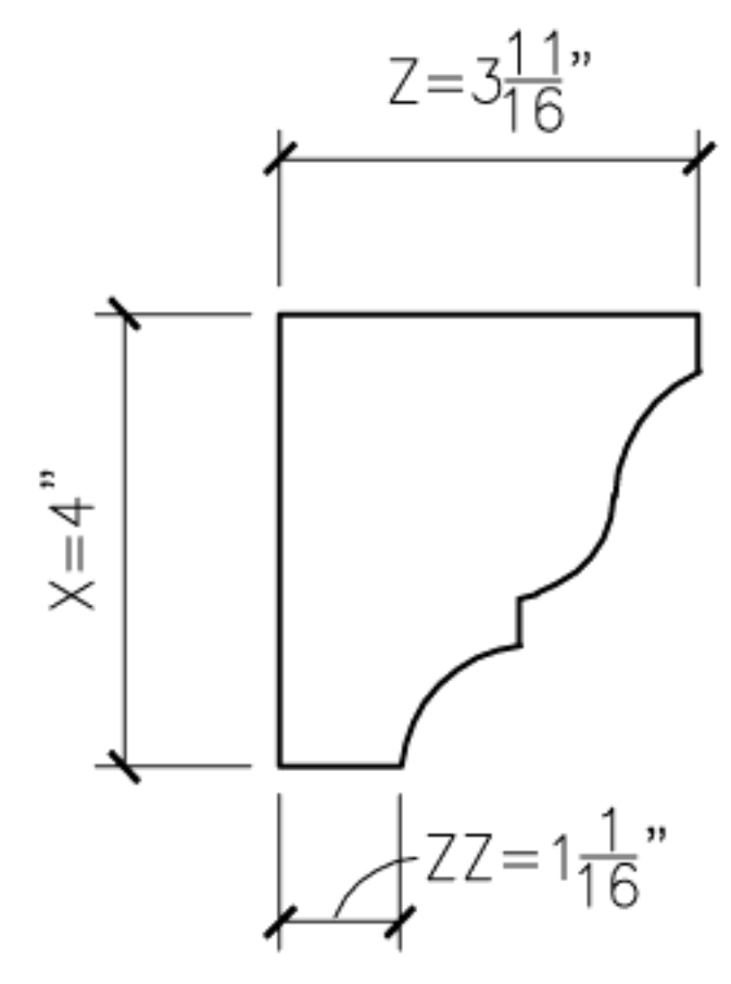
1 ORIEL1 PROFILE SECTION
