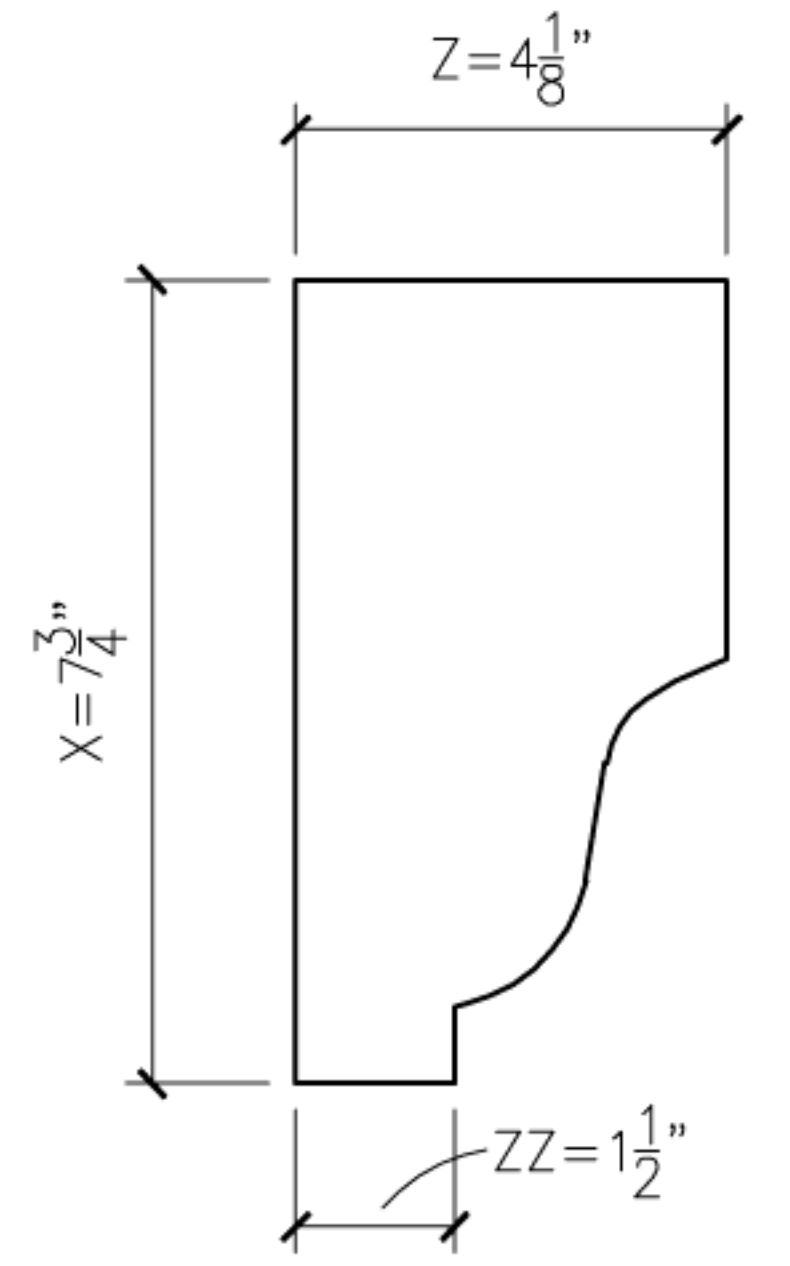
25 OGEE25 PROFILE SECTION
