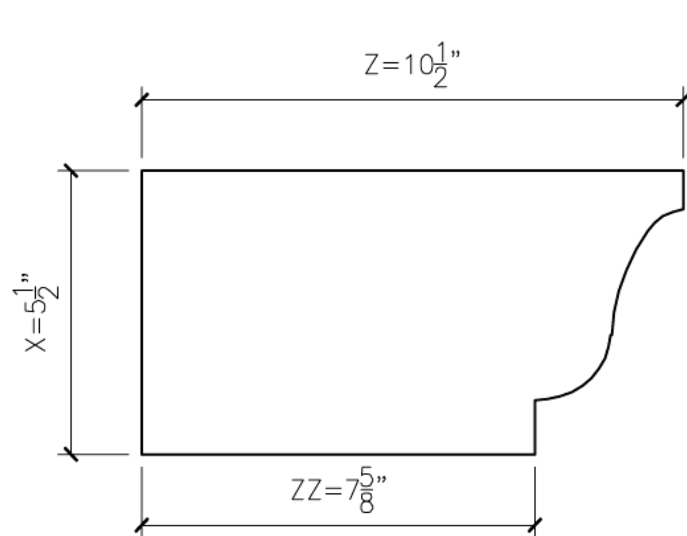
15A OGEE15A PROFILE SECTION
