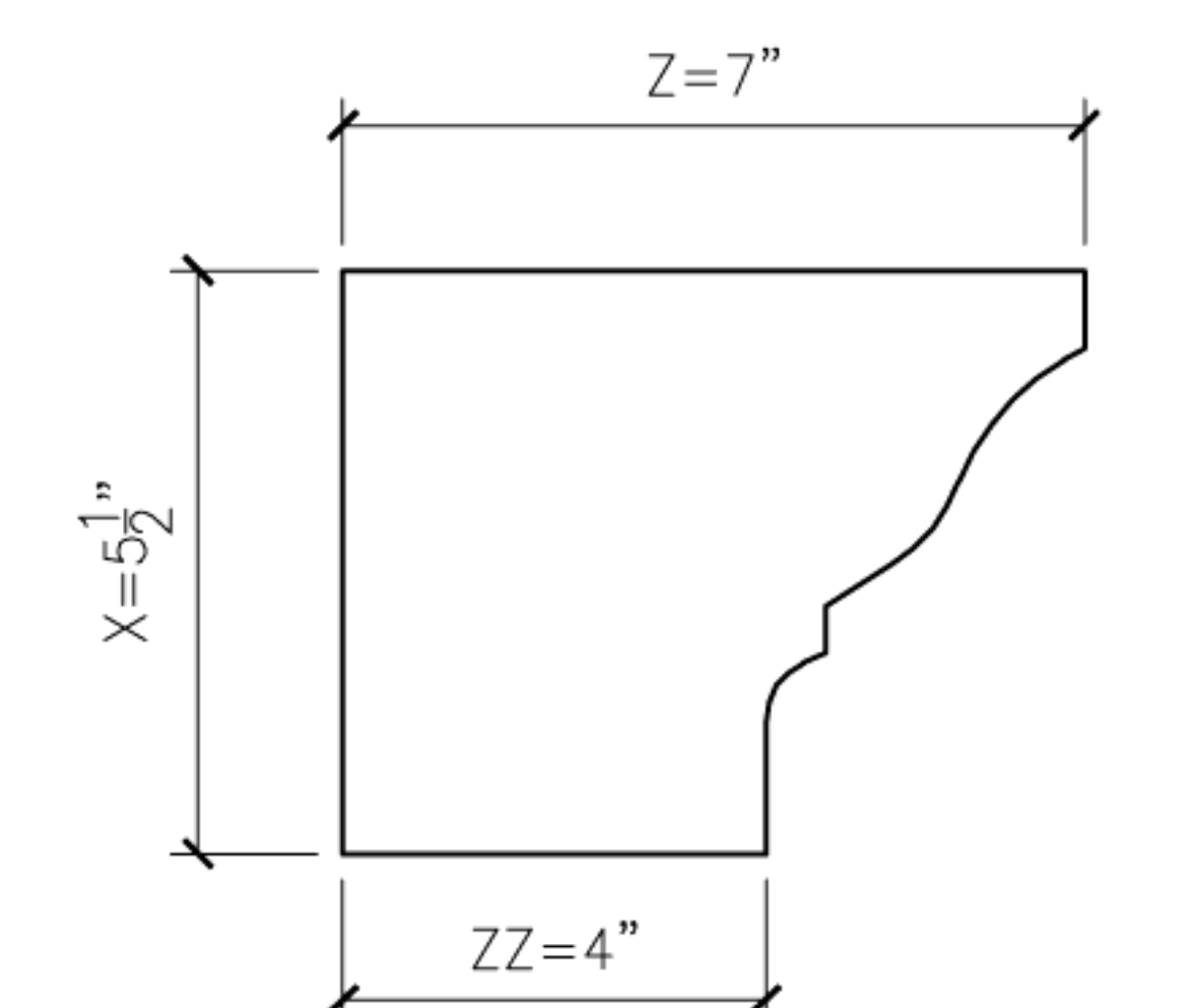
16 ORIEL16 PROFILE SECTION
