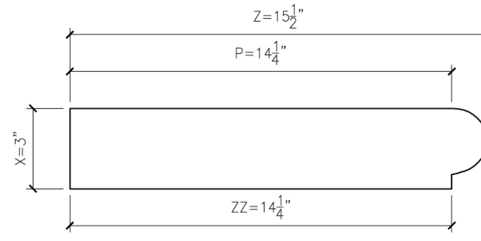
3 BULLNOSE8 PROFILE SECTION
