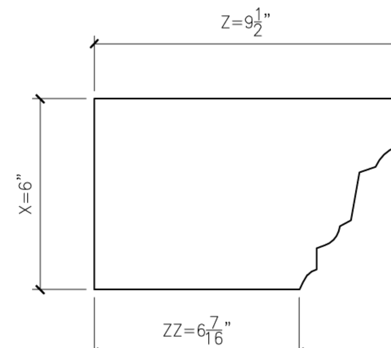
3A JAMISON3A PROFILE SECTION
