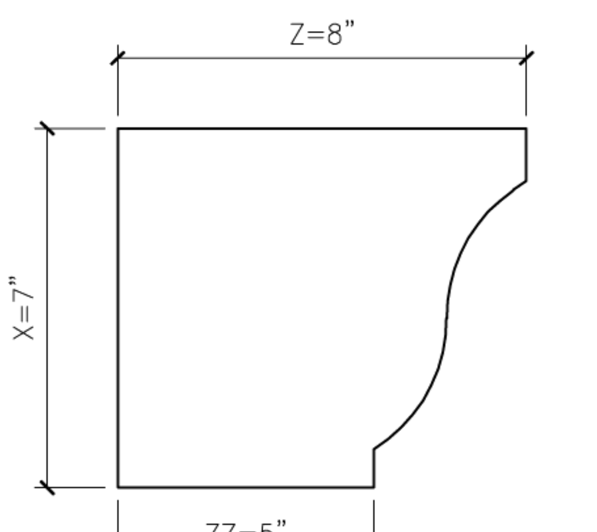
17 OGEE17 PROFILE SECTION
