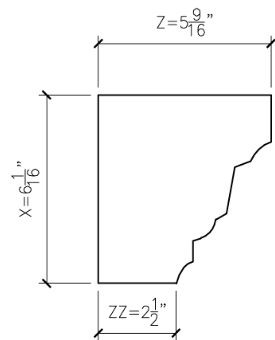
3 JAMISON3 PROFILE SECTION
