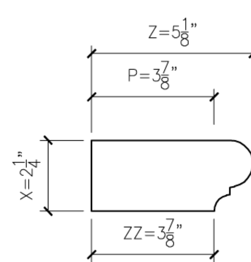
5 BOLSON5 PROFILE SECTION
