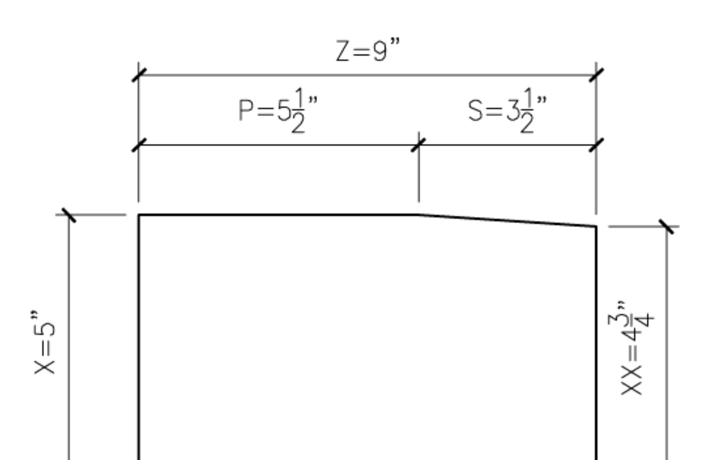
24 WEDGE24 PROFILE SECTION
