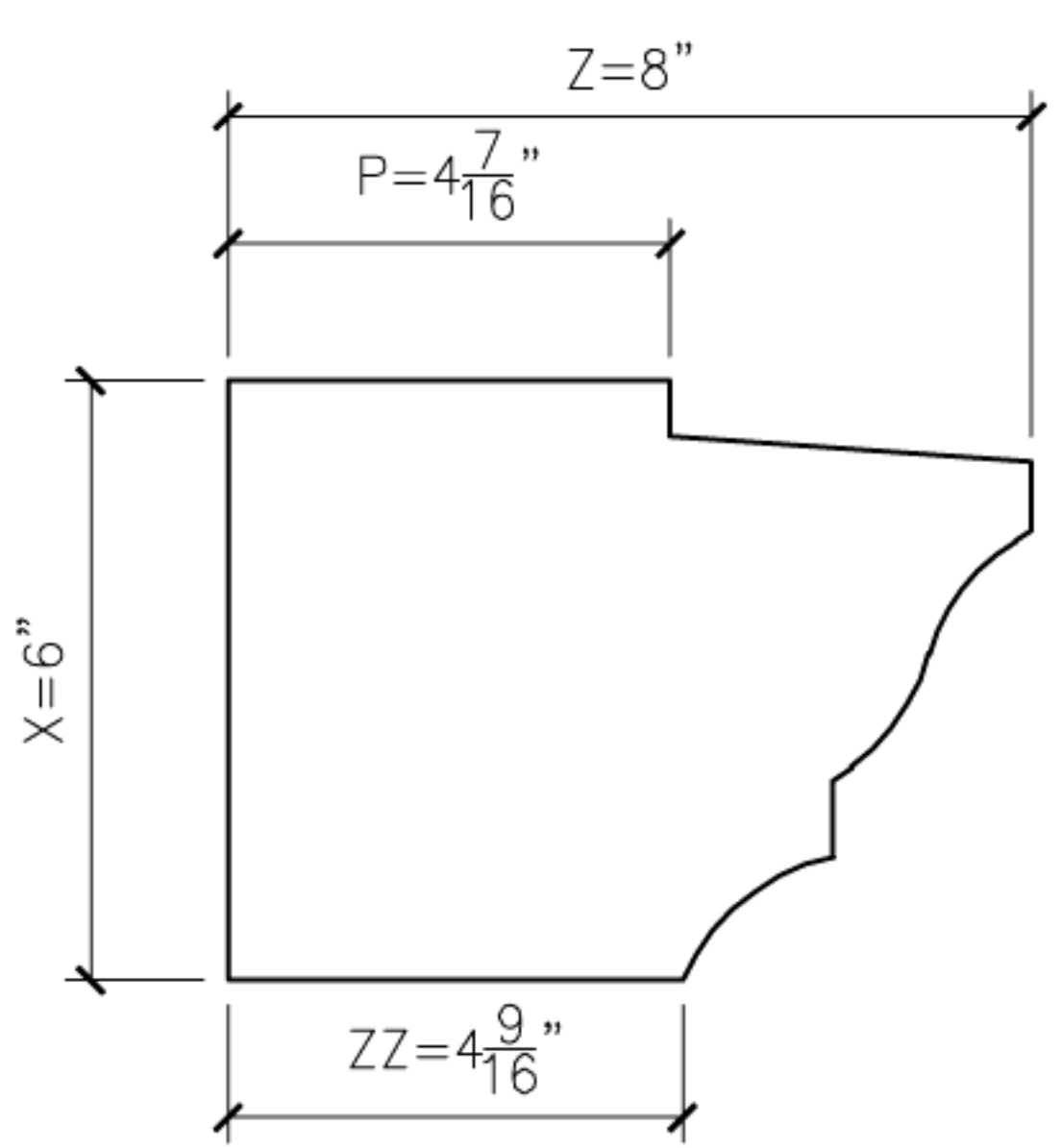
4 ORIEL4 PROFILE SECTION
