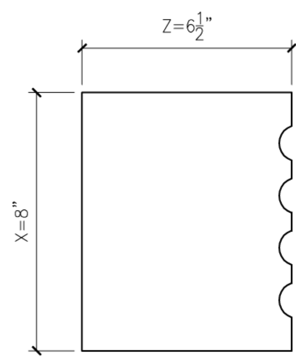
1A GEORGIAN1A PROFILE SECTION
