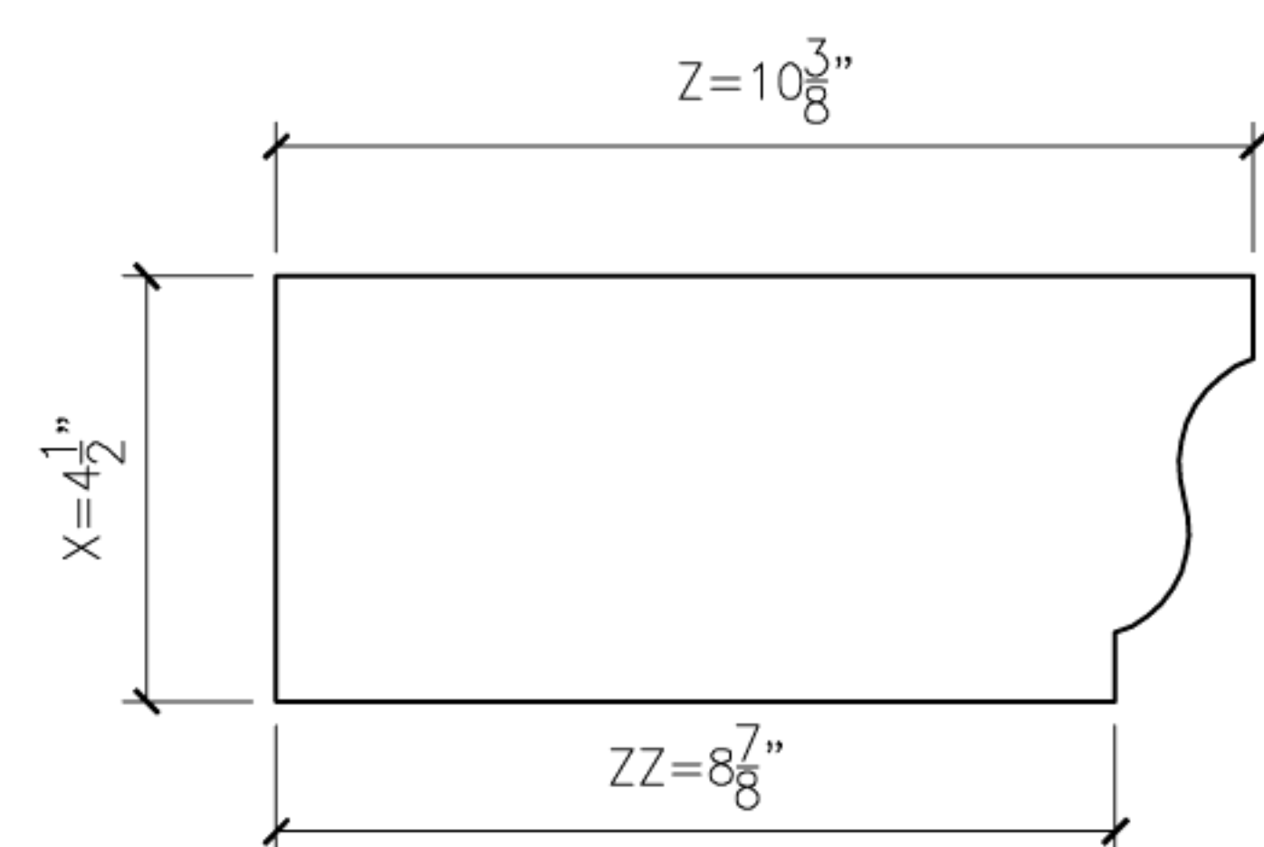
12 OGEE12 PROFILE SECTION
