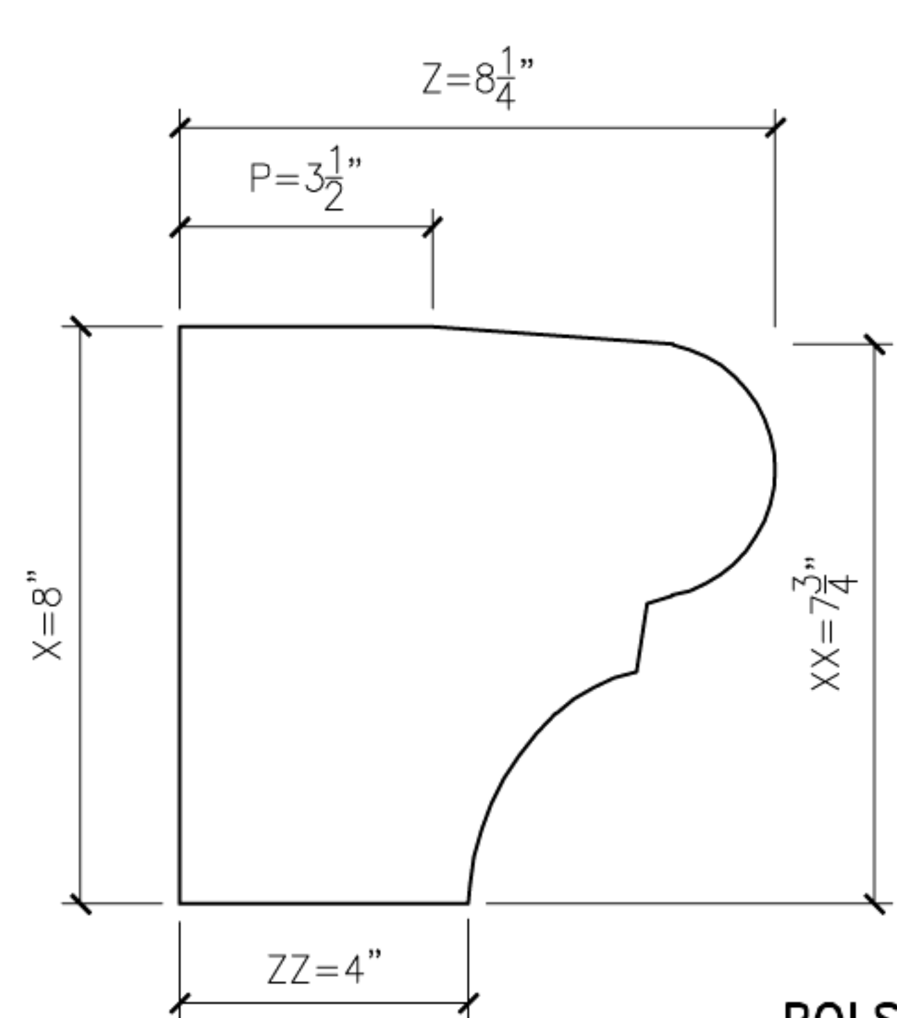
14 BOLSON14 PROFILE SECTION
