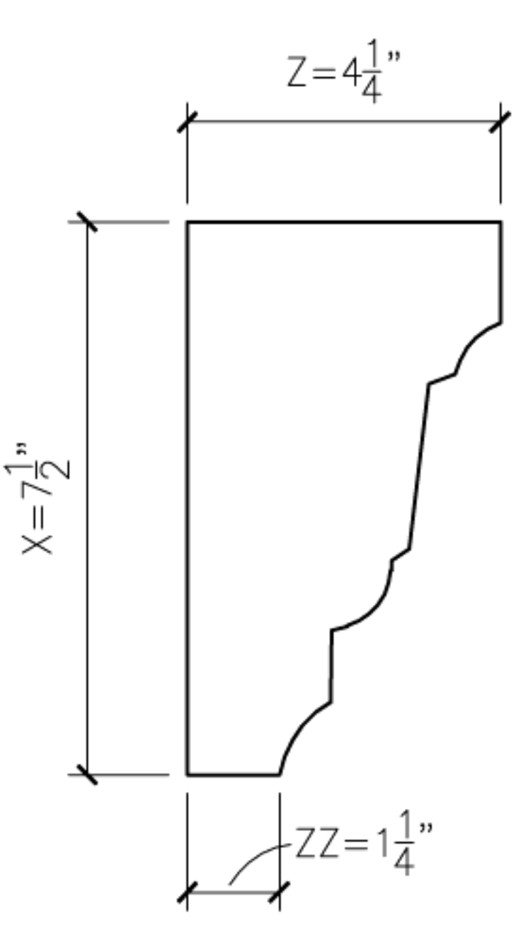
8 JAMISON8 PROFILE SECTION
