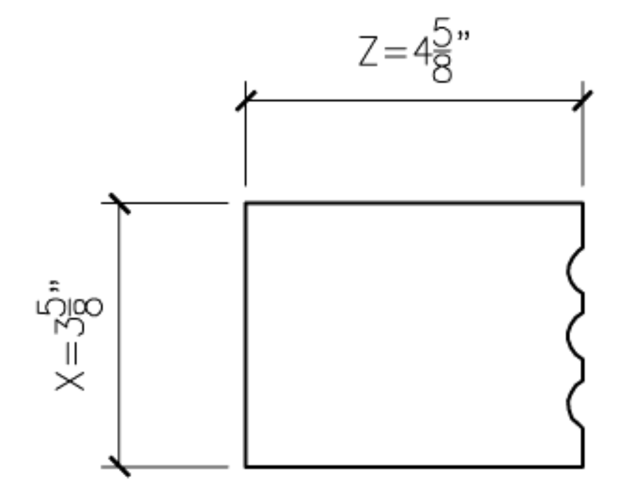
10 GEORGIAN10 PROFILE SECTION
