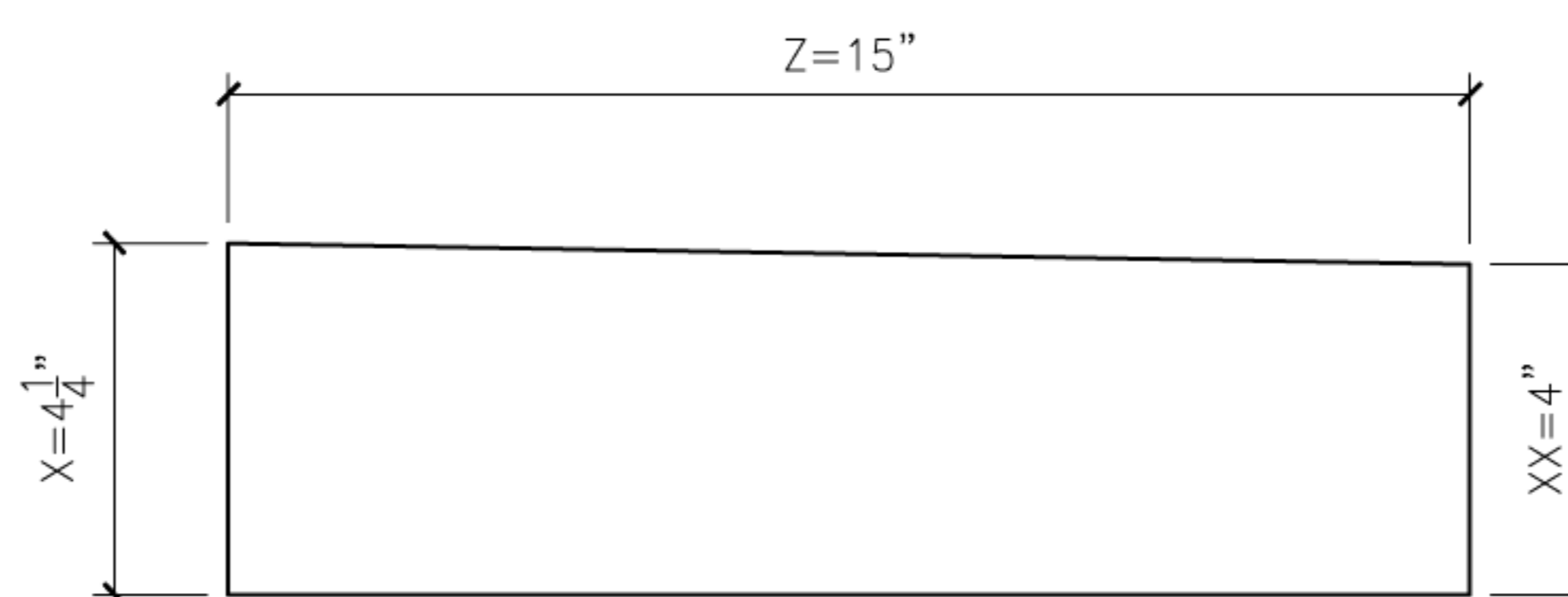
15 FLATFACE SLOPE16 PROFILE SECTION
