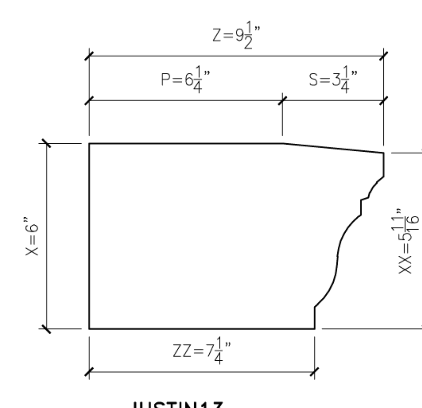
12 JUSTIN13 PROFILE SECTION
