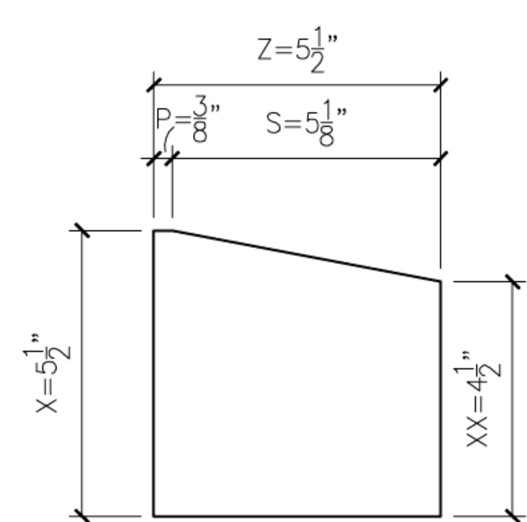
21 WEDGE21 PROFILE SECTION
