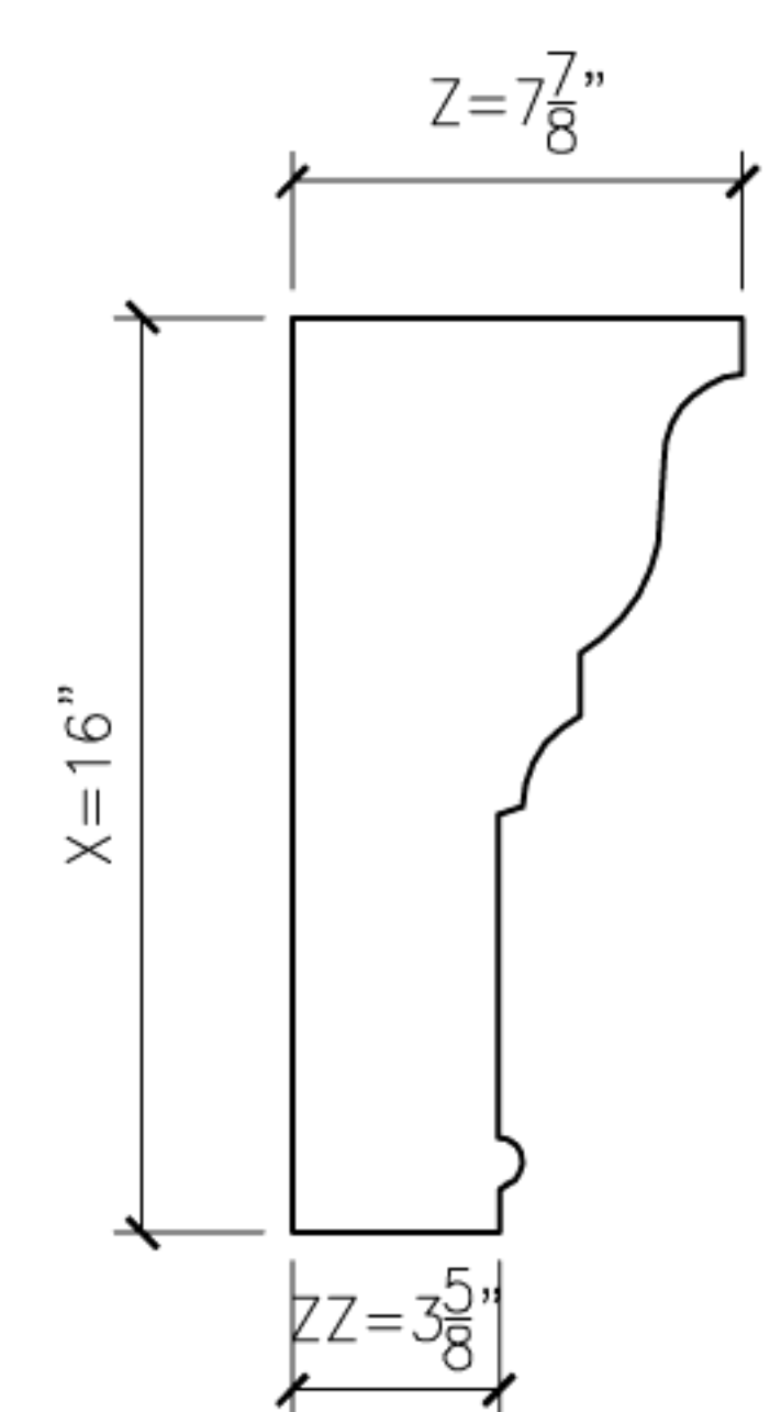
14 ORIEL14 PROFILE SECTION
