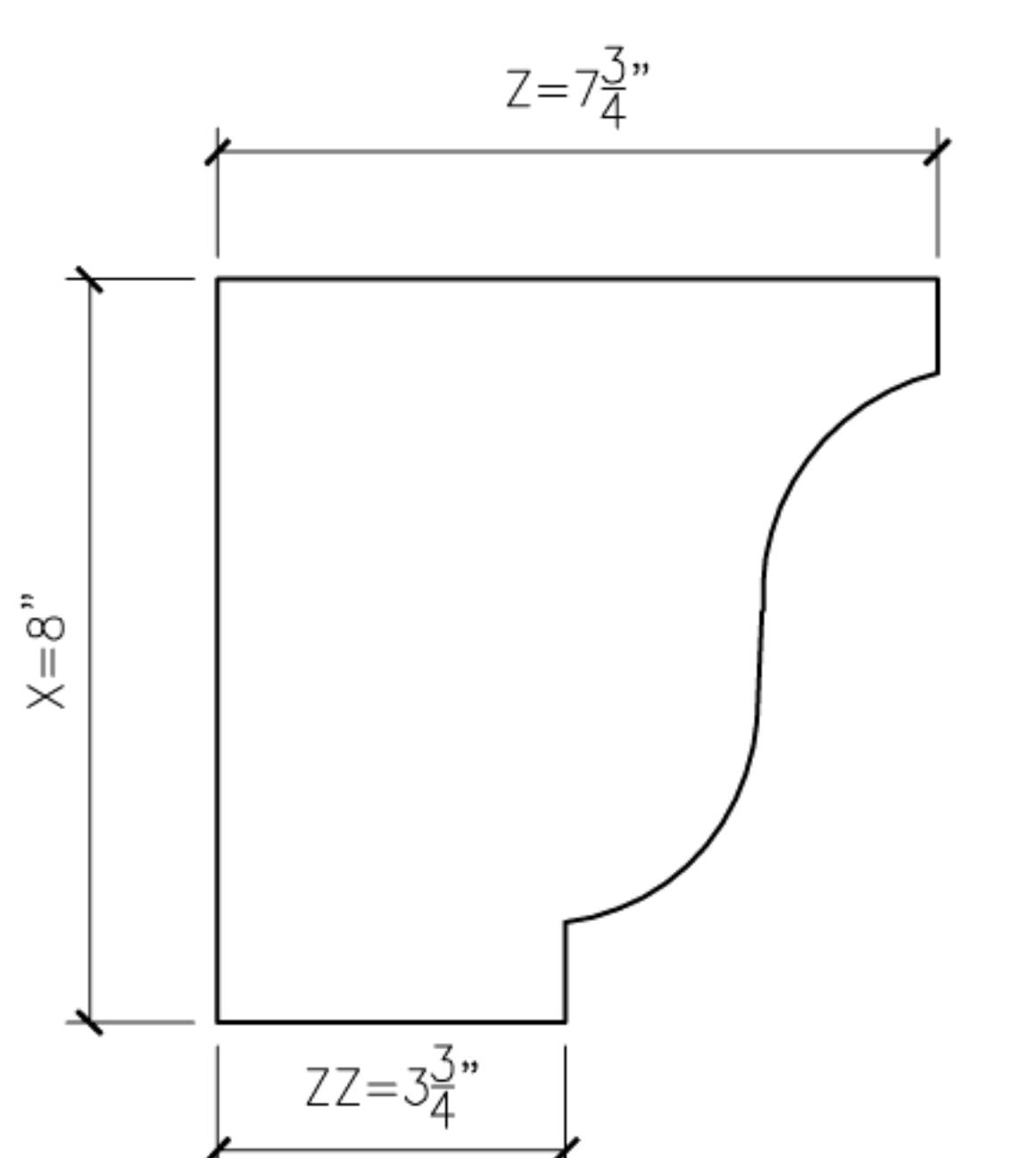
10 OGEE10 PROFILE SECTION
