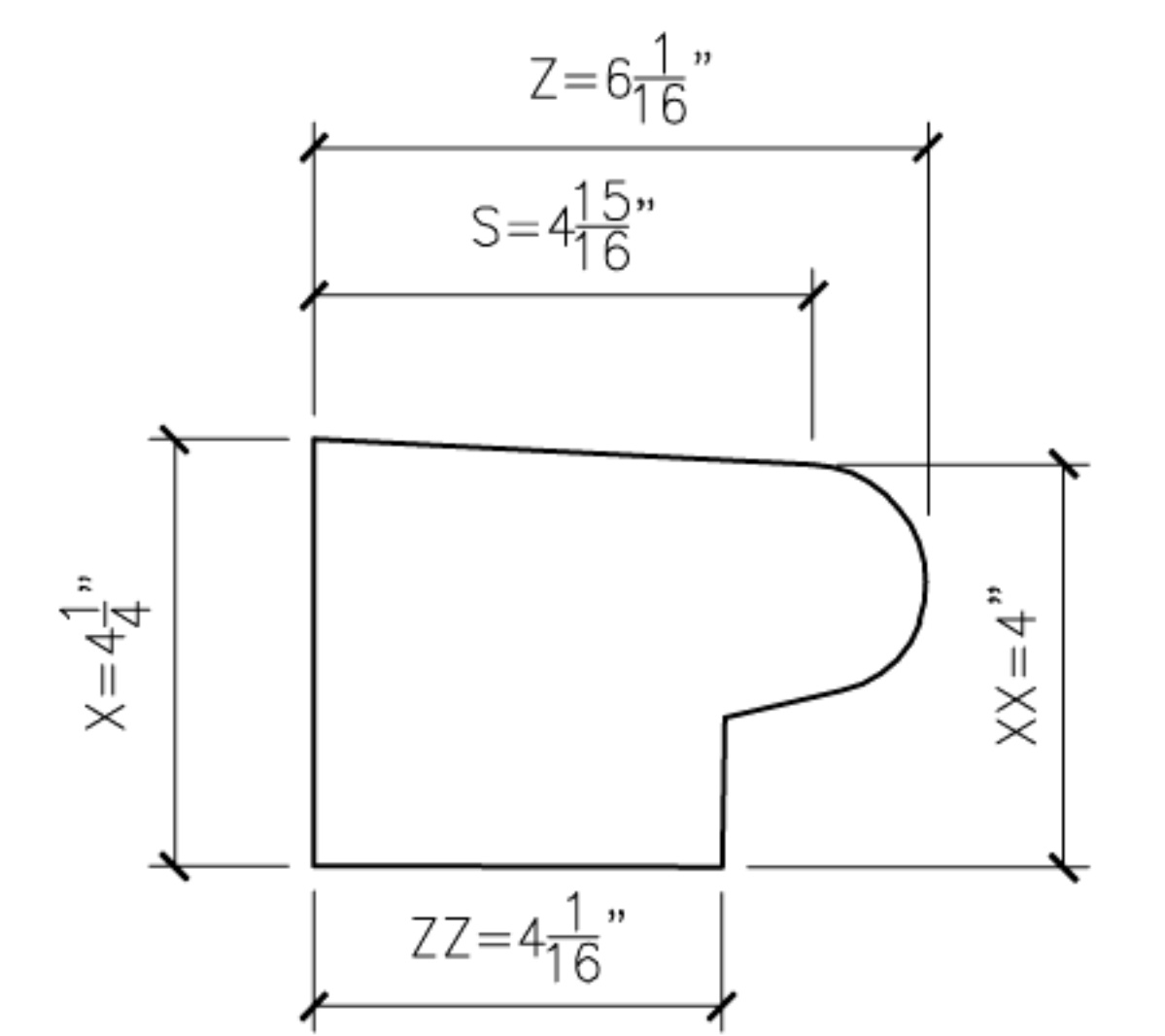
10 BULLNOSE RISE2 PROFILE SECTION
