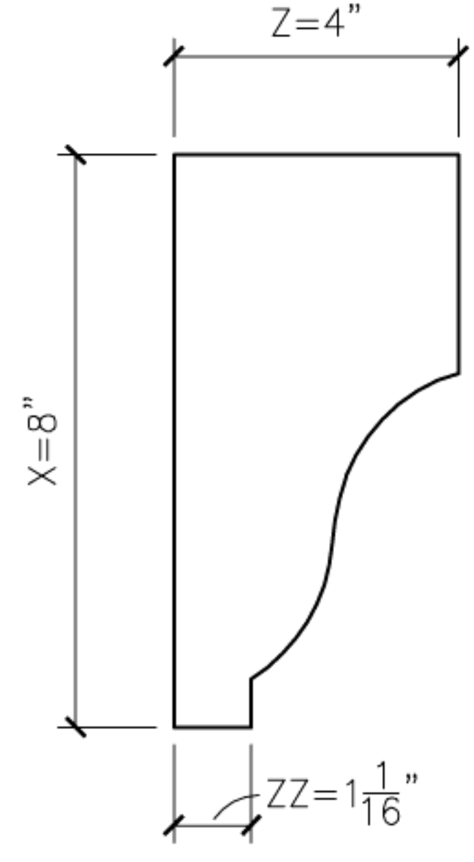
26 OGEE26 PROFILE SECTION
