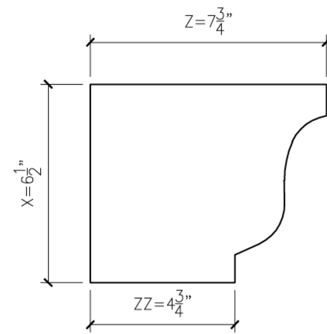
16 OGEE16 PROFILE SECTION
