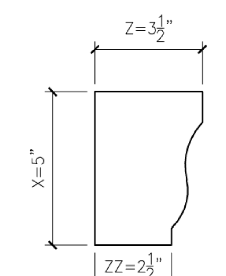
13A OGEE13A PROFILE SECTION
