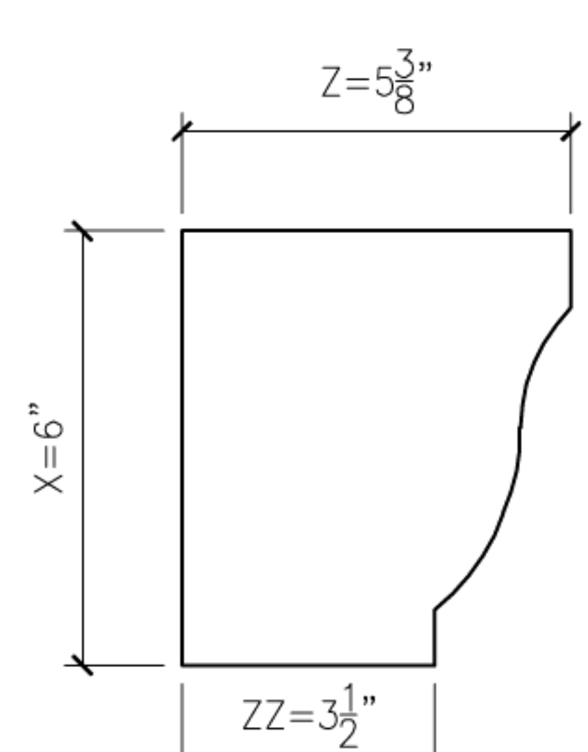
18 OGEE18 PROFILE SECTION
