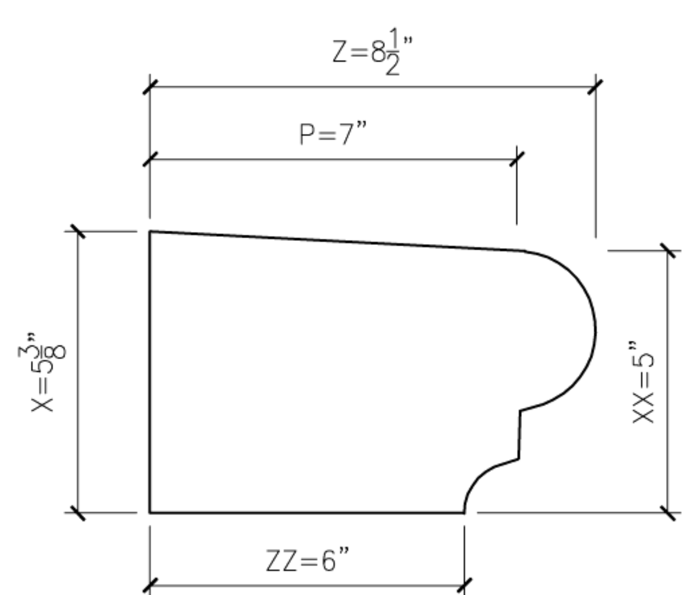
7 BOLSON7 PROFILE SECTION
