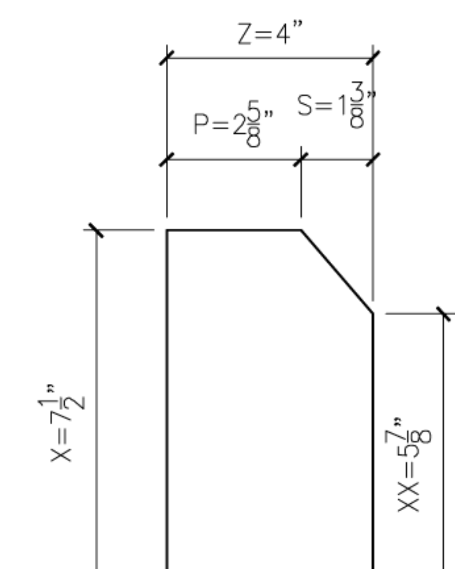
14 WEDGE14 PROFILE SECTION
