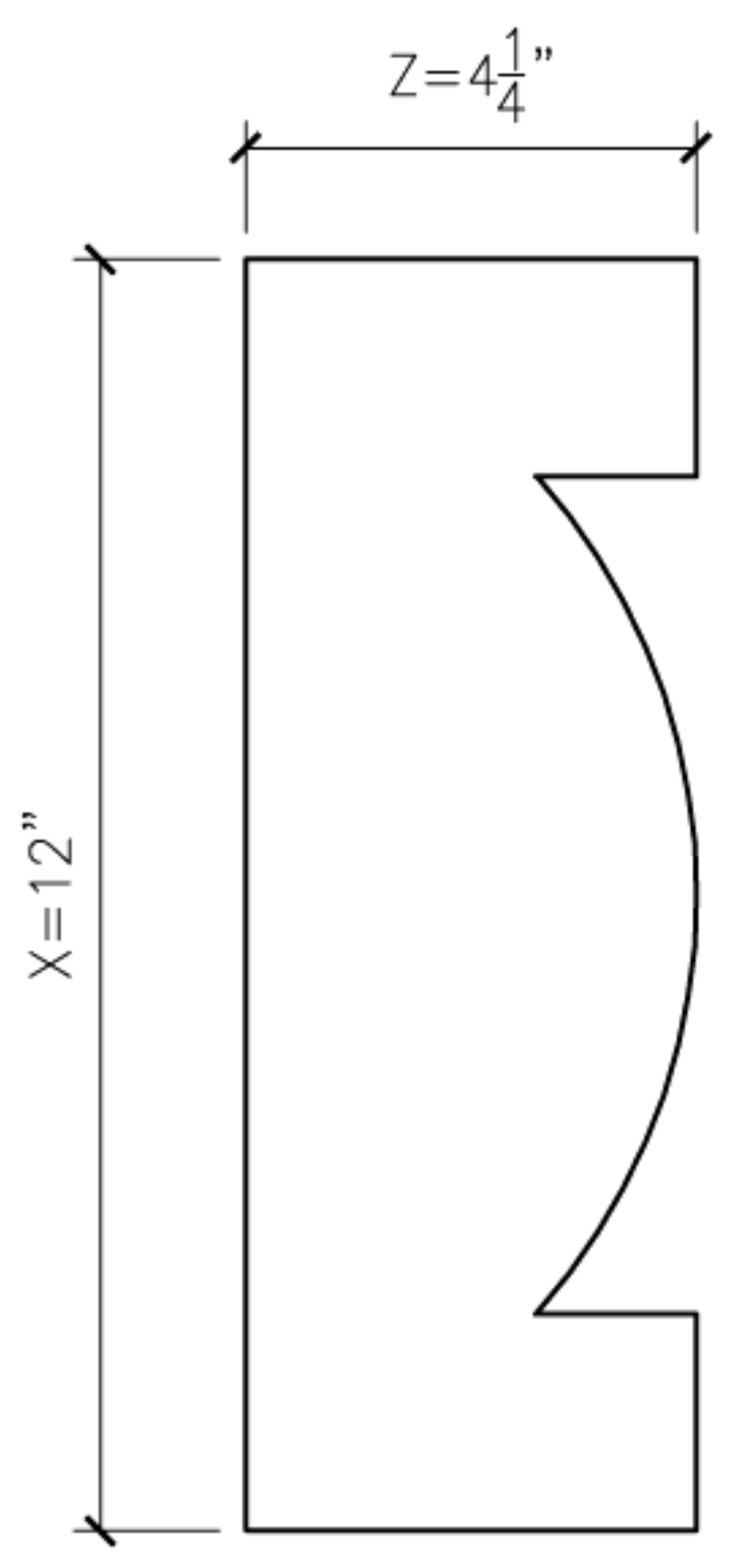
1 NAVARRO1 PROFILE SECTION
