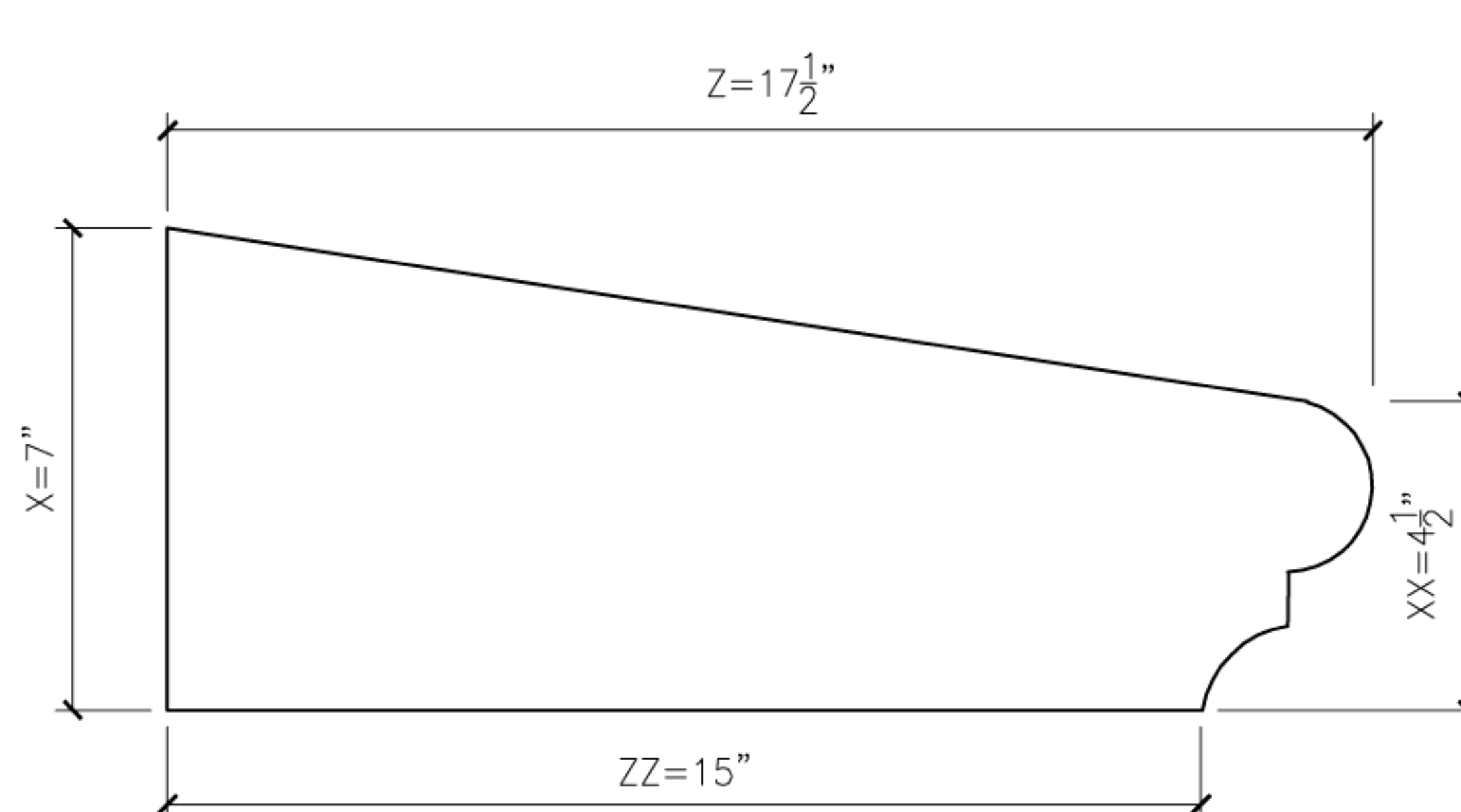
15 BOLSON15 PROFILE SECTION
