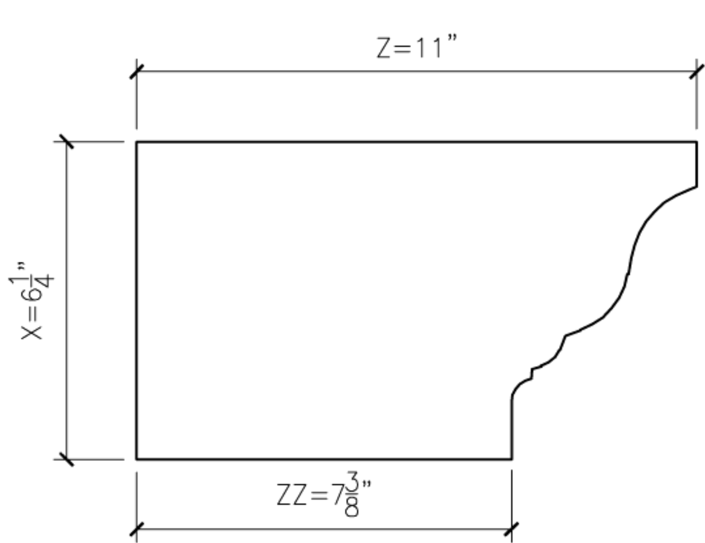
17 ORIEL17 PROFILE SECTION
