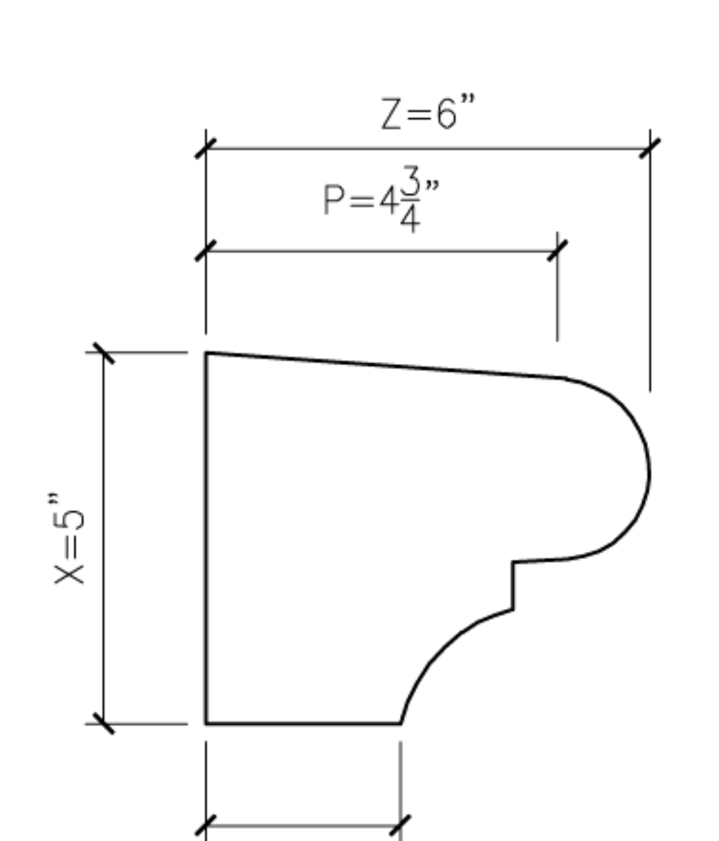
9 BOLSON9 PROFILE SECTION
