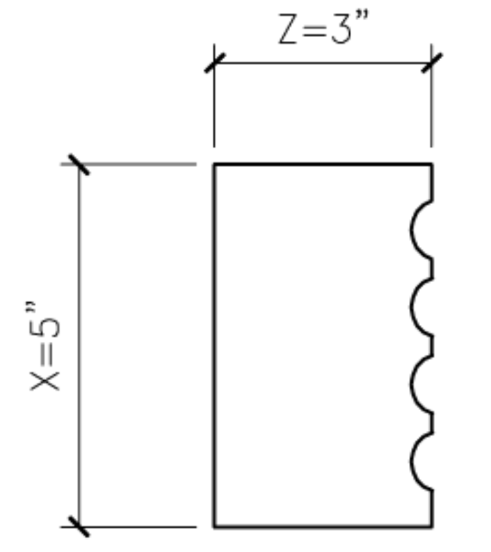
2A GEORGIAN2A PROFILE SECTION
