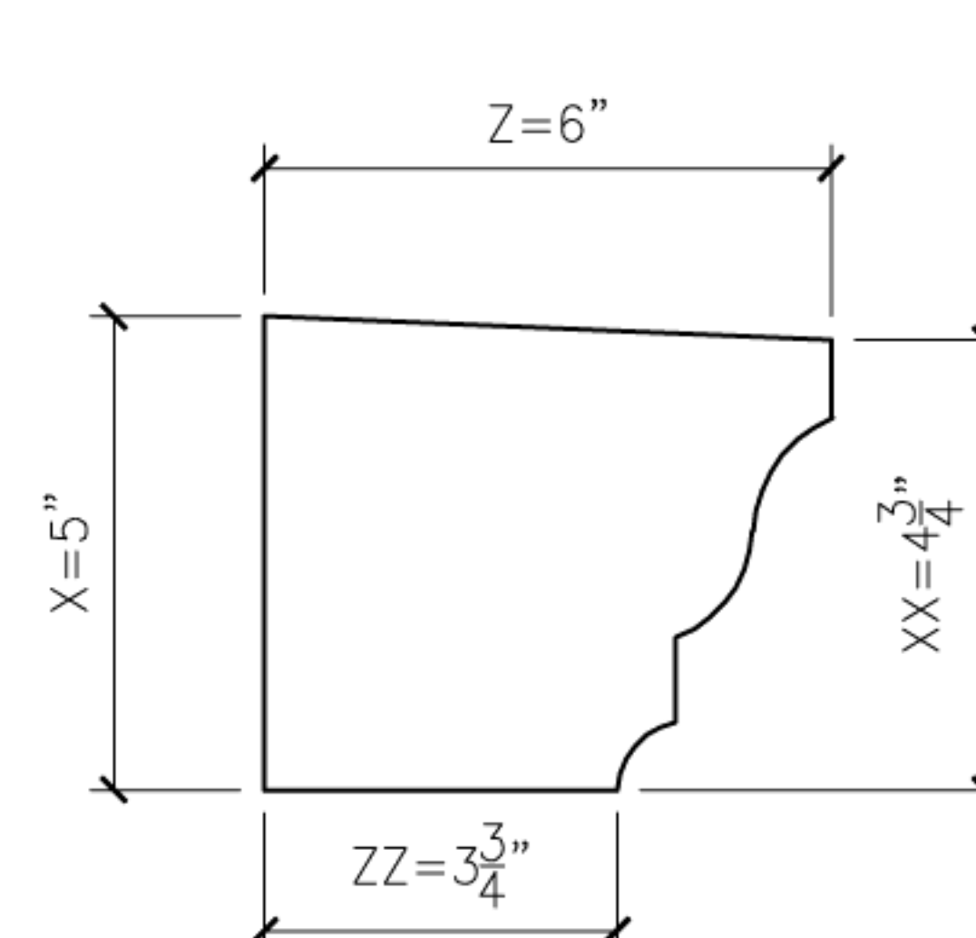
18 ORIEL18 PROFILE SECTION
