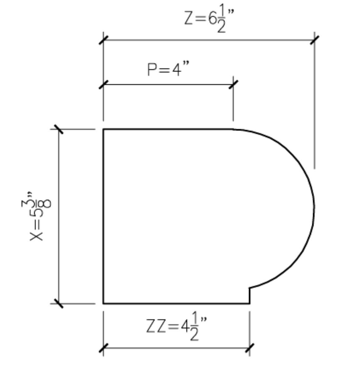
4 BULLNOSE10 PROFILE SECTION
