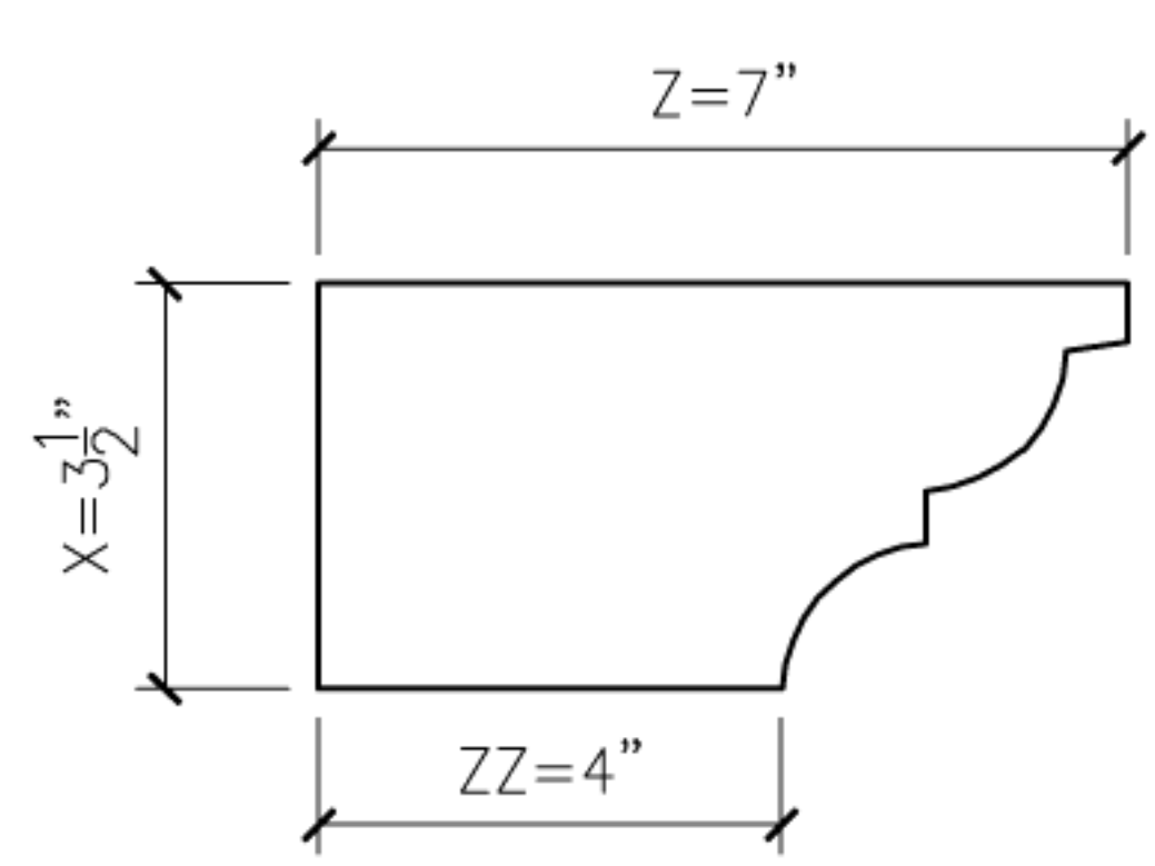
13 ORIEL13 PROFILE SECTION
