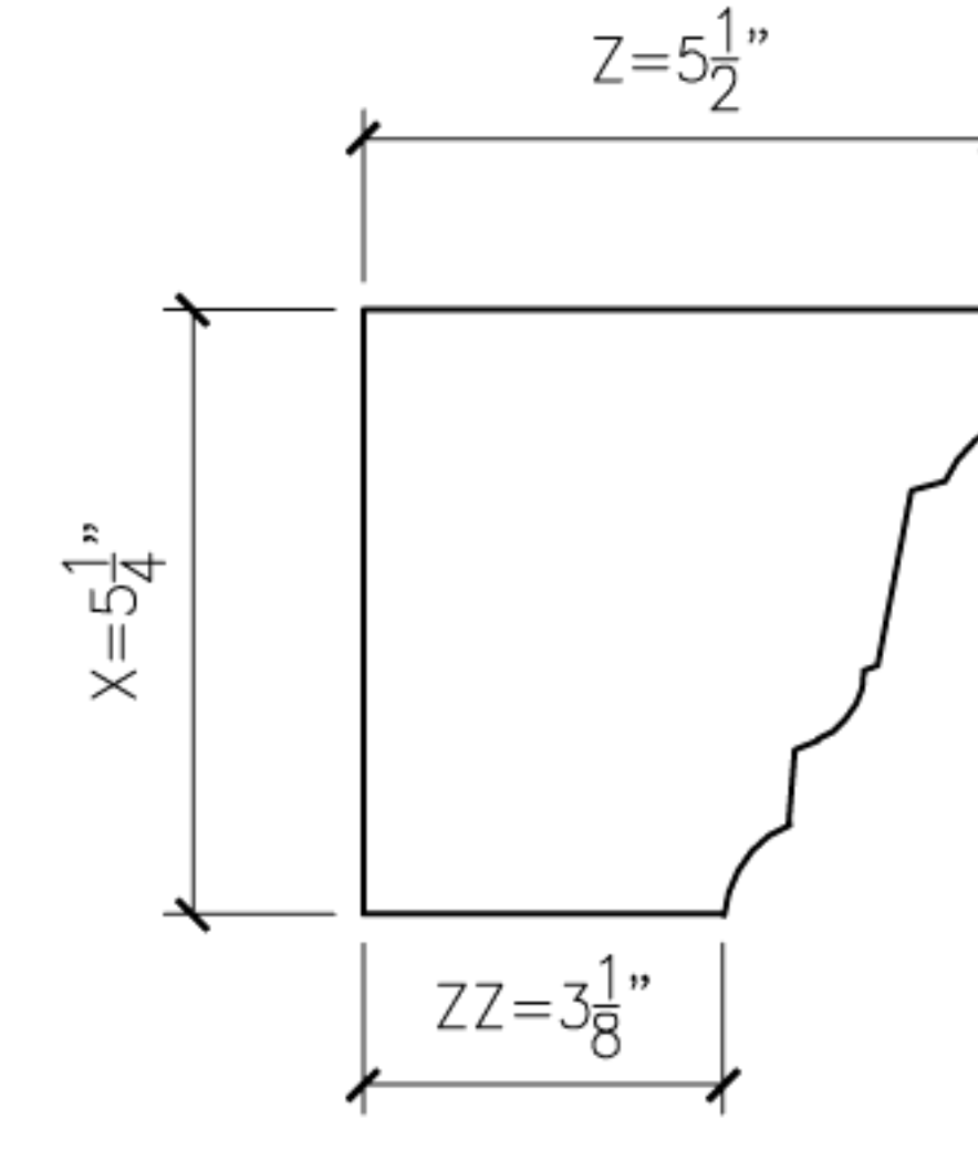
2 JAMISON2 PROFILE SECTION
