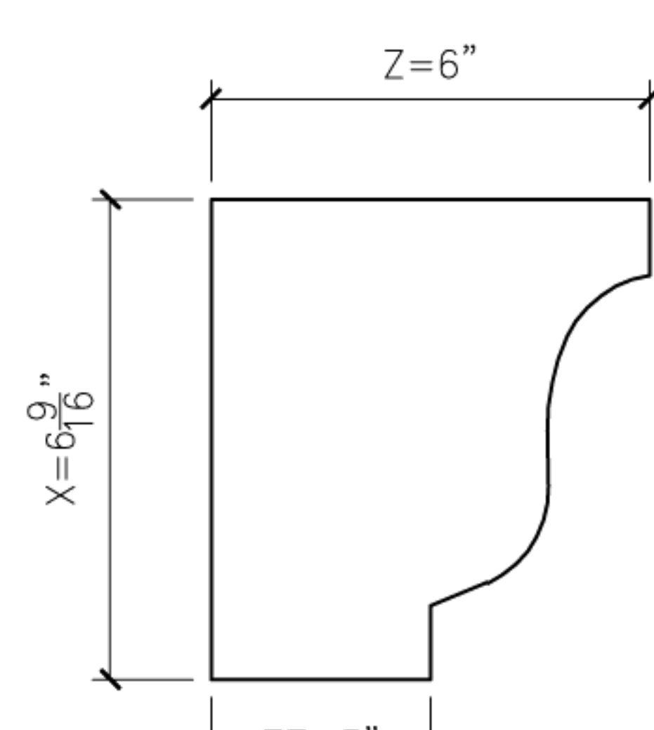
19 OGEE19 PROFILE SECTION
