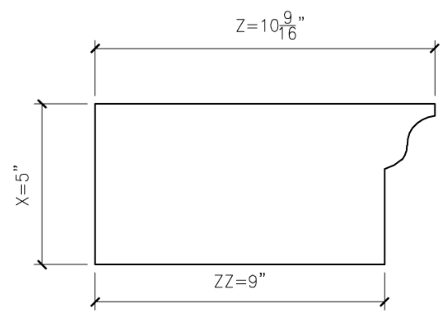
23 OGEE23 PROFILE SECTION
