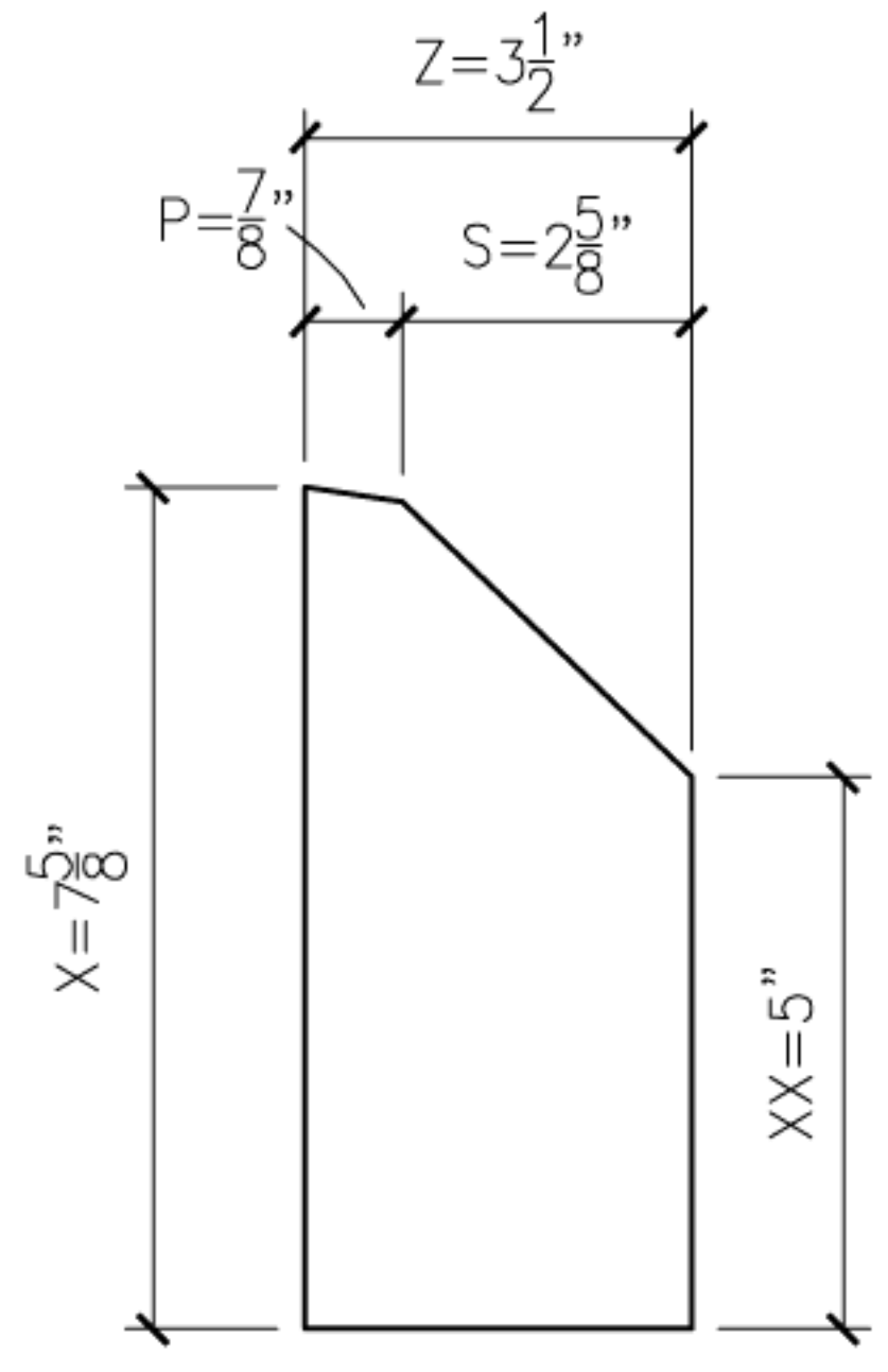
33 WEDGE33 PROFILE SECTION
