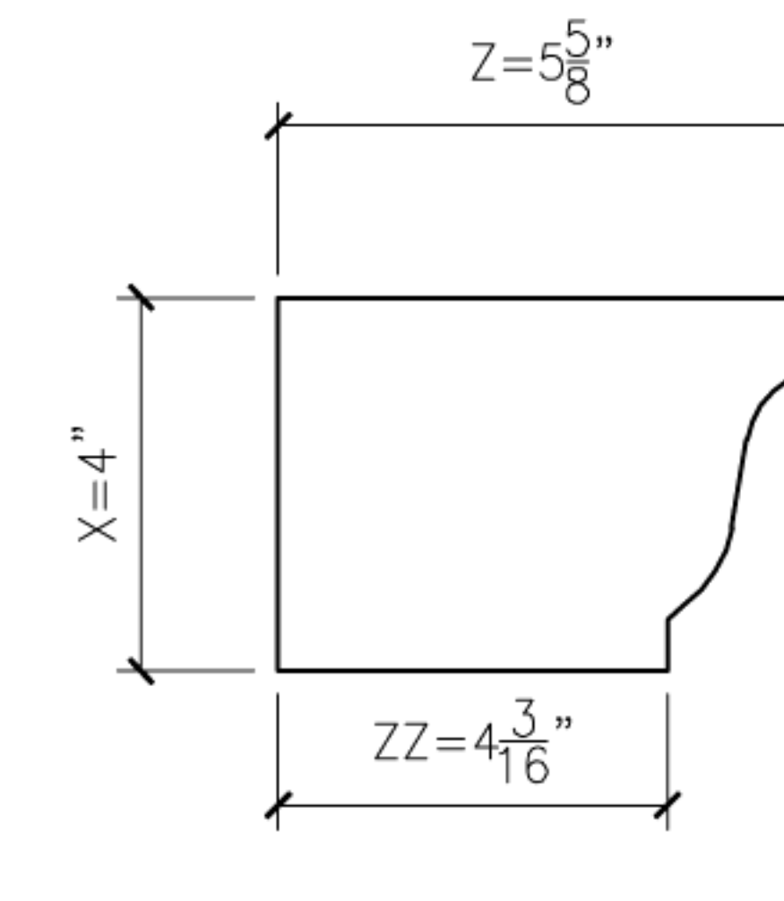
9 OGEE9 PROFILE SECTION
