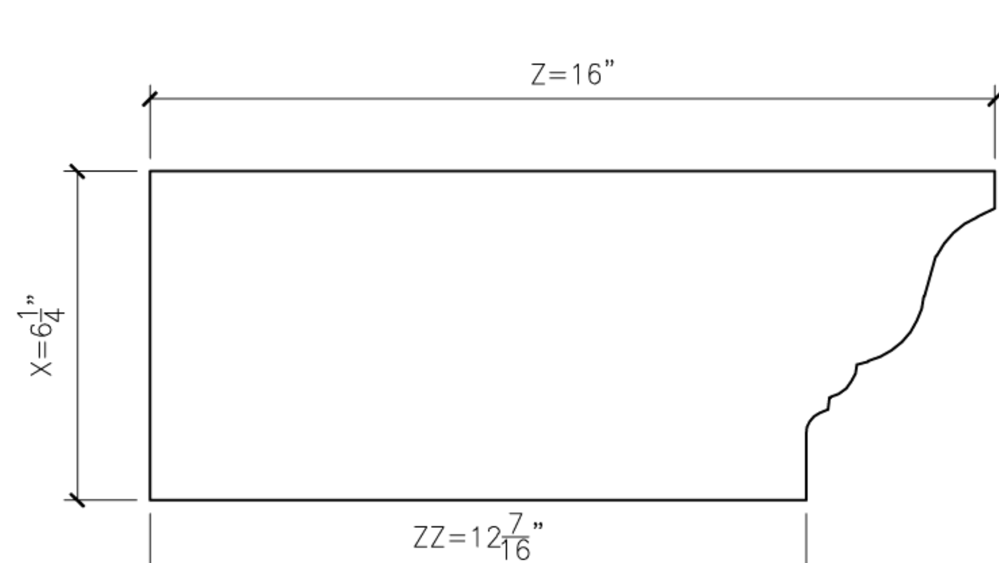
17A ORIEL17A PROFILE SECTION
