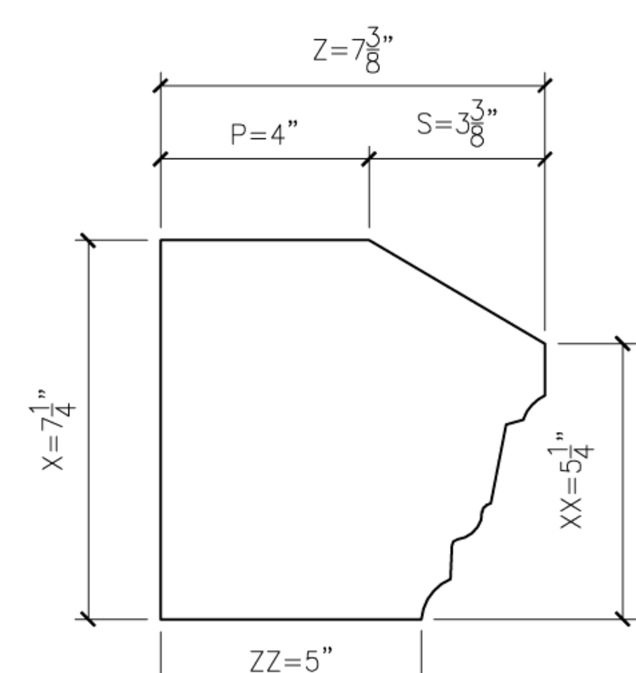
9 JAMISON9 PROFILE SECTION
