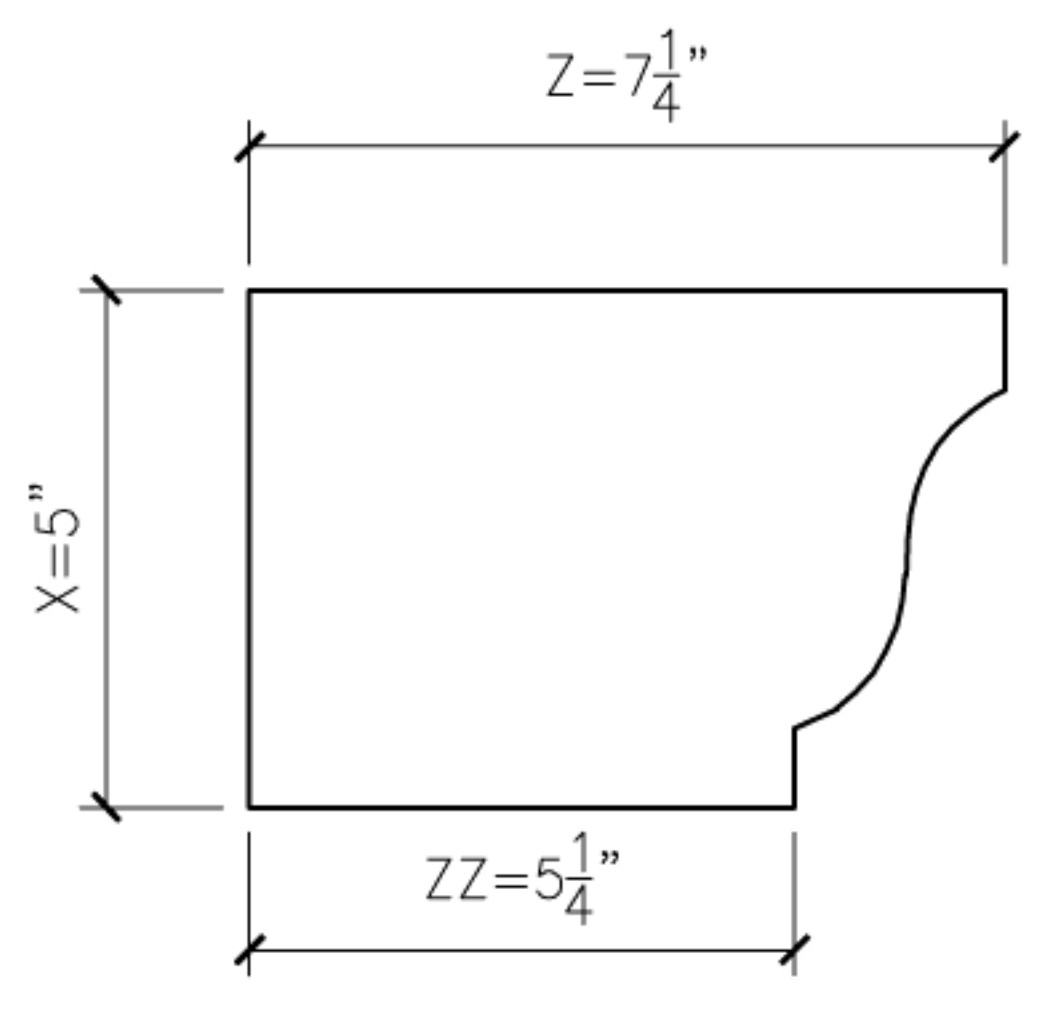
22 OGEE22 PROFILE SECTION
