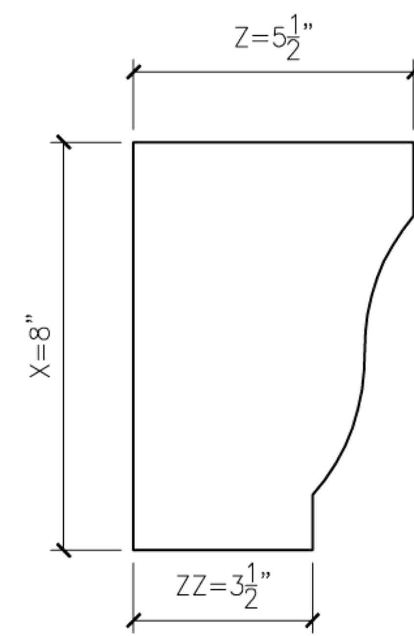
8 OGEE8 PROFILE SECTION
