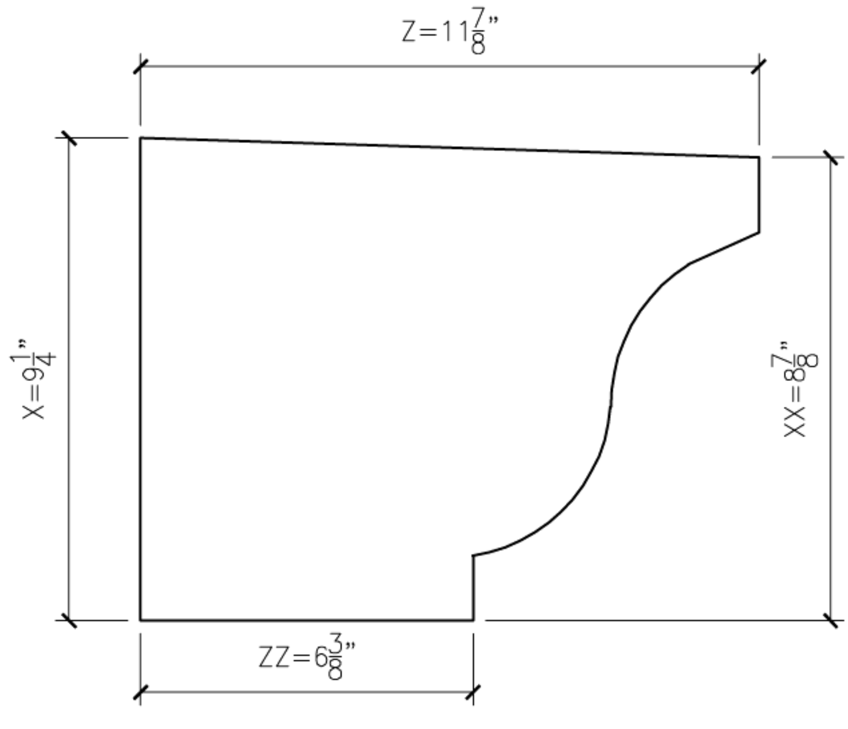
1 OGEE1 PROFILE SECTION
