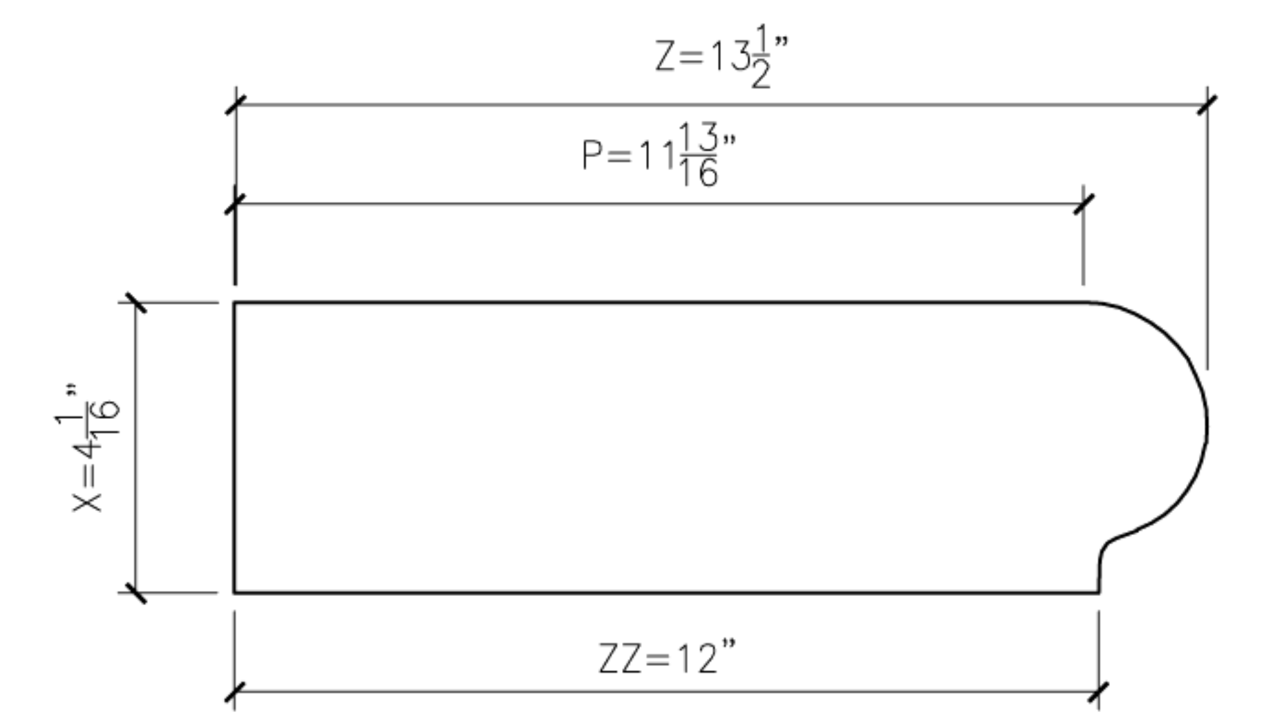
6 BULLNOSE14 PROFILE SECTION
