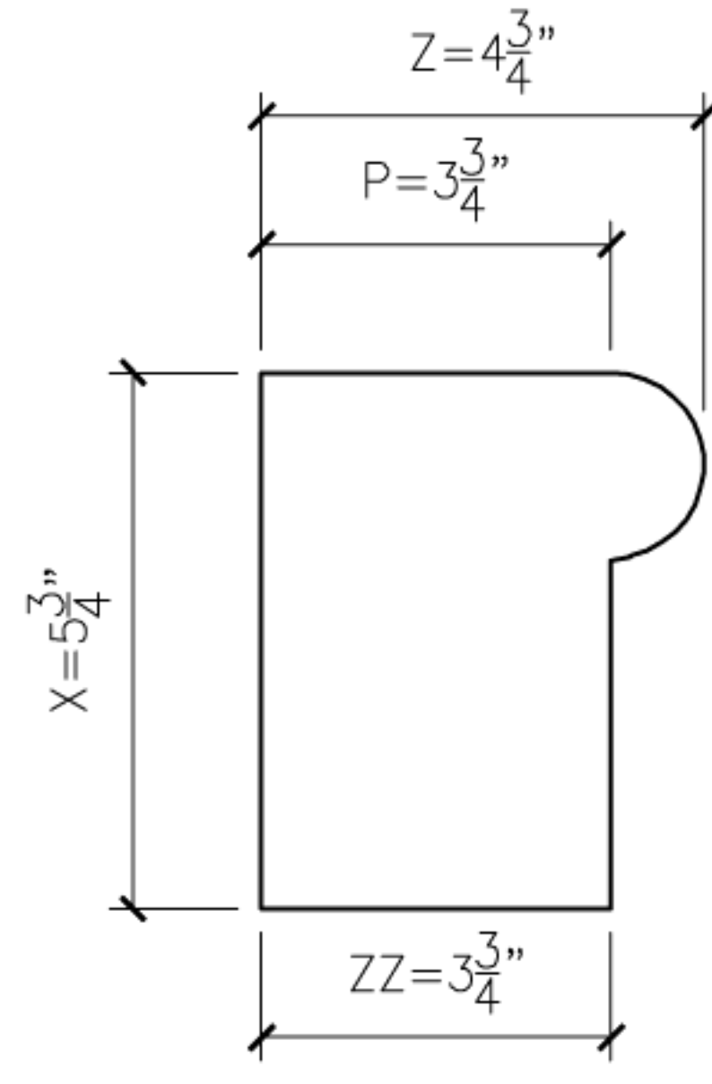
2 BULLNOSE3 PROFILE SECTION
