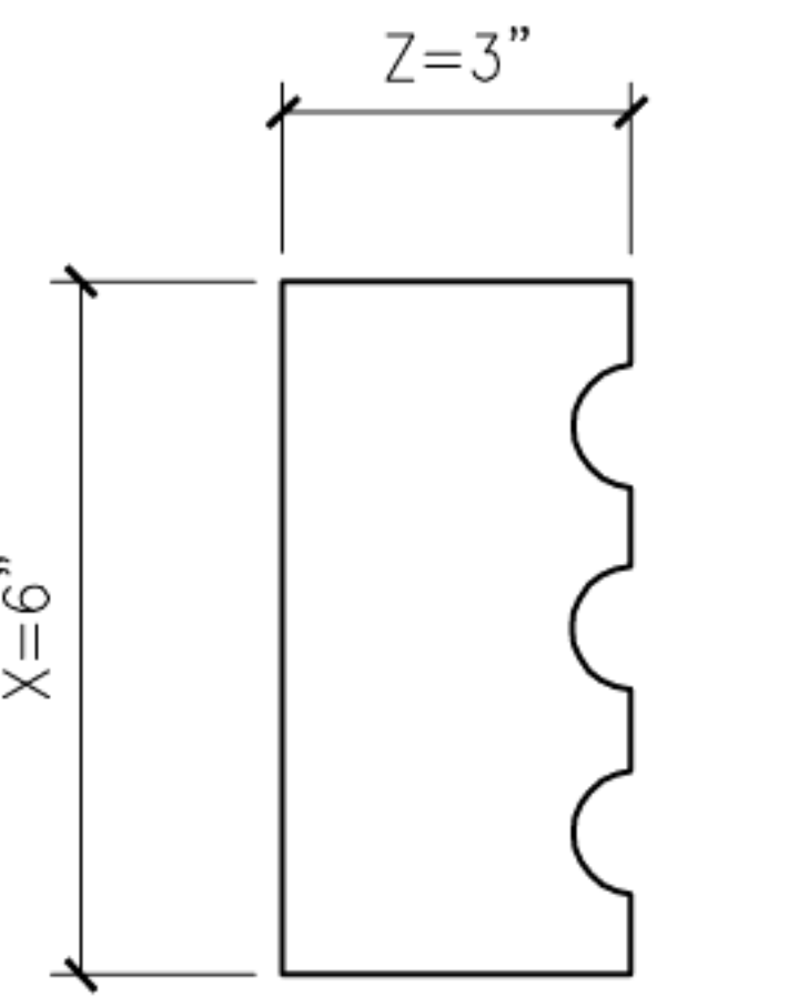
7 GEORGIAN7 PROFILE SECTION
