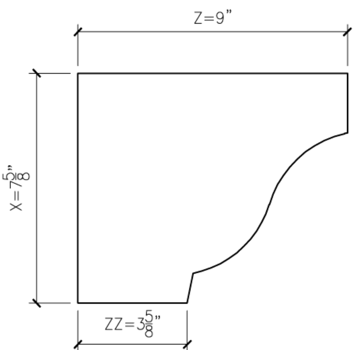
30 OGEE30 PROFILE SECTION
