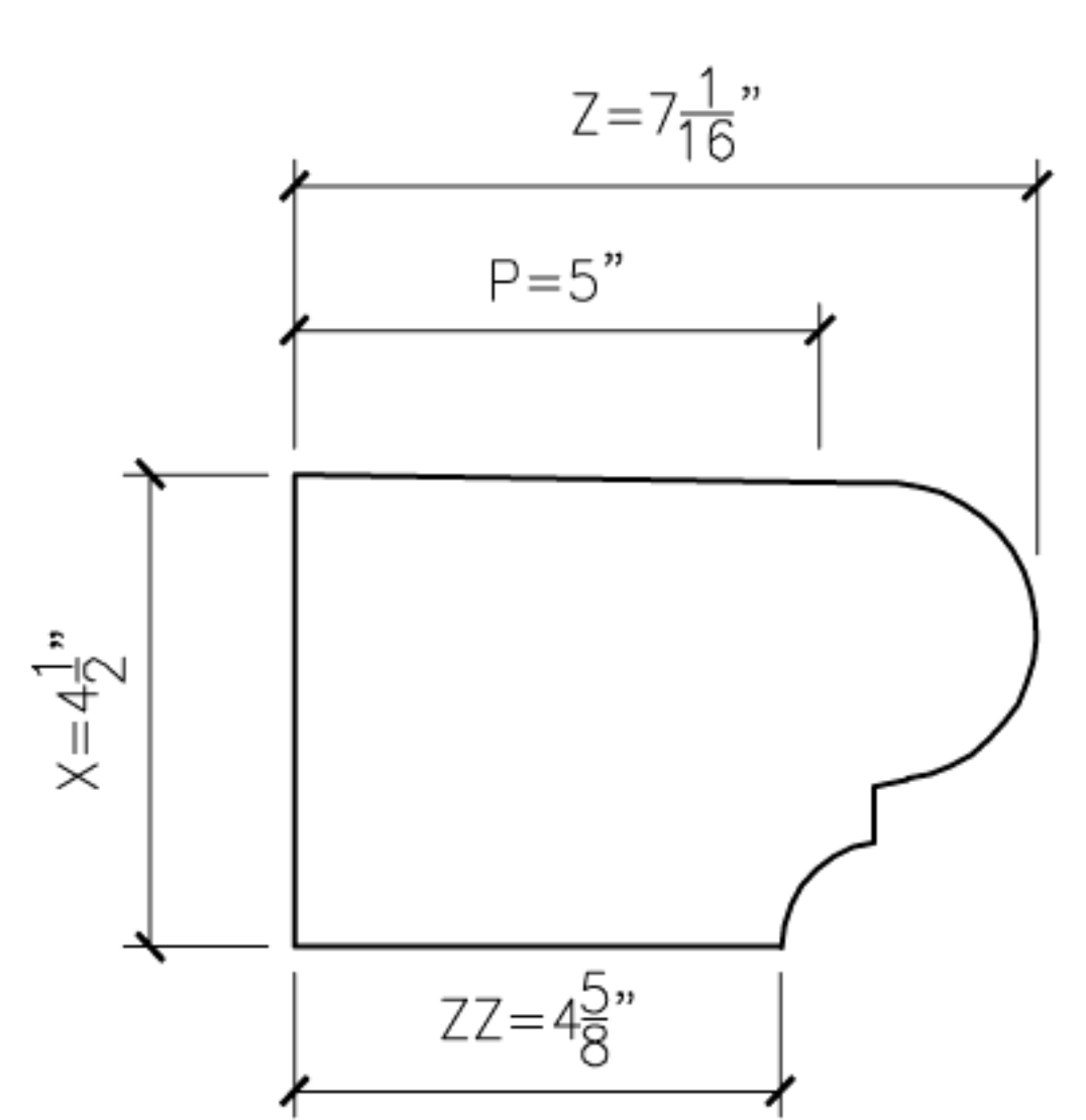
17A BOLSON17A PROFILE SECTION
