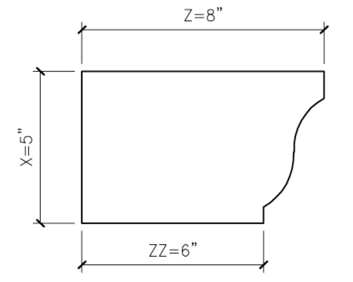
3 OGEE3 PROFILE SECTION
