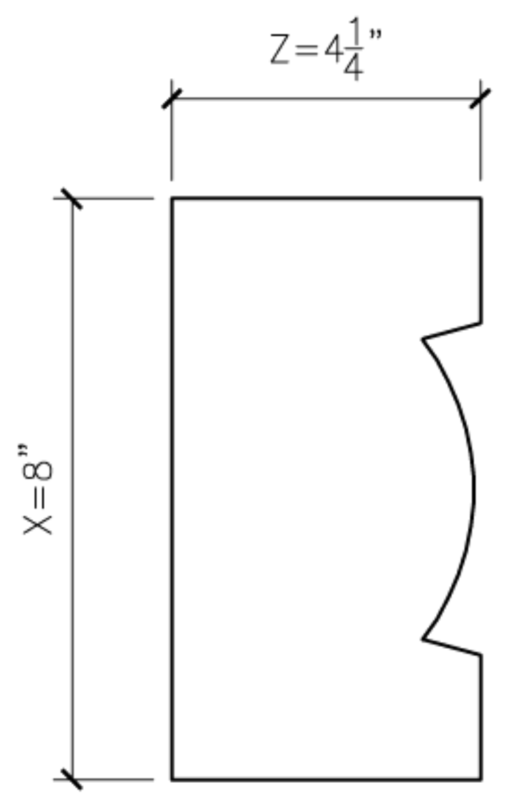
7 NAVARRO7 PROFILE SECTION
