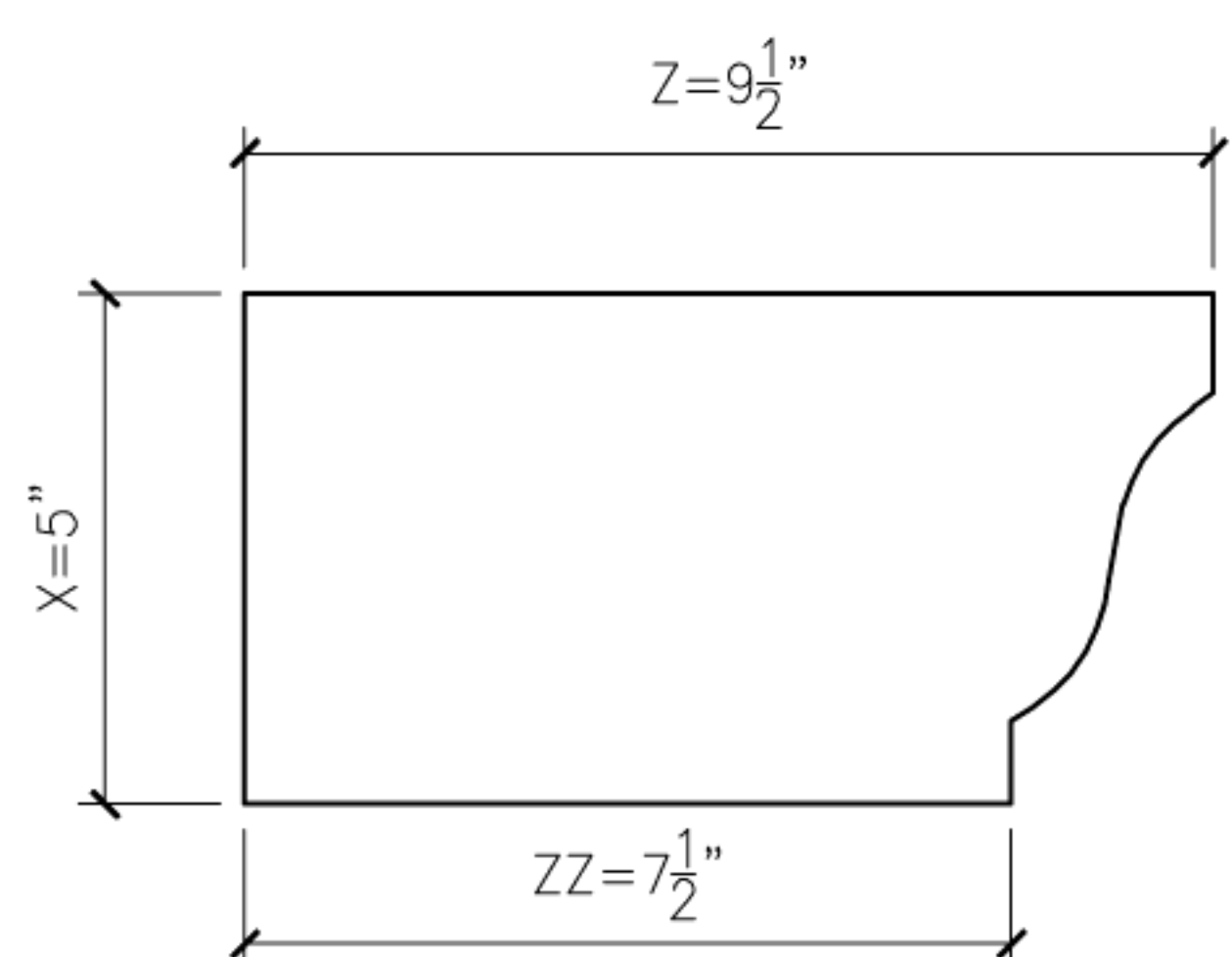
14 OGEE14 PROFILE SECTION
