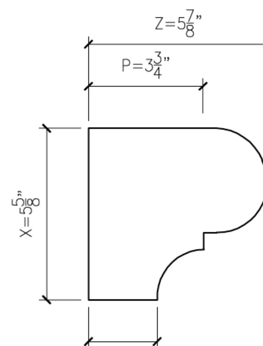
8 BOLSON8 PROFILE SECTION
