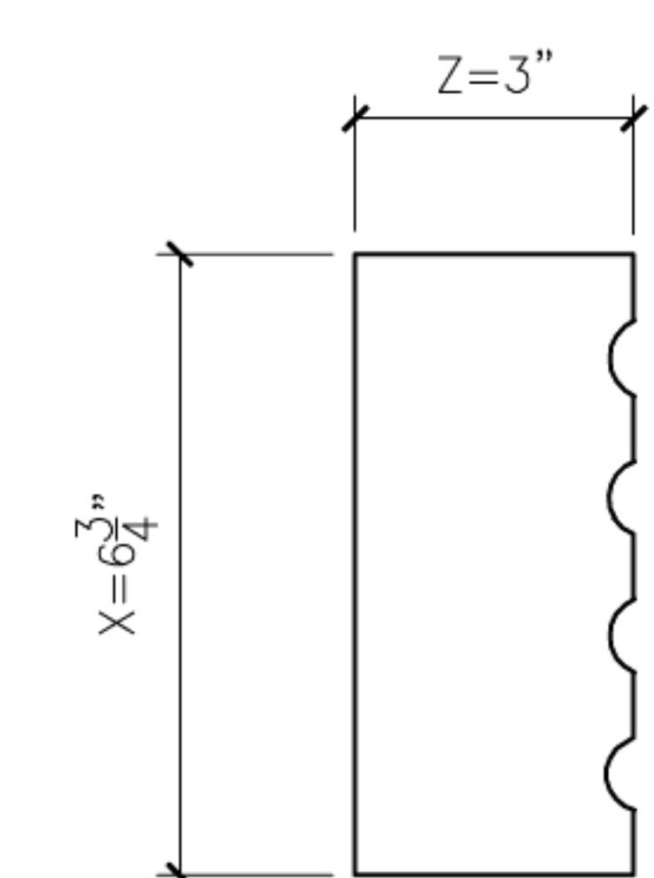
19 GEORGIAN19 PROFILE SECTION
