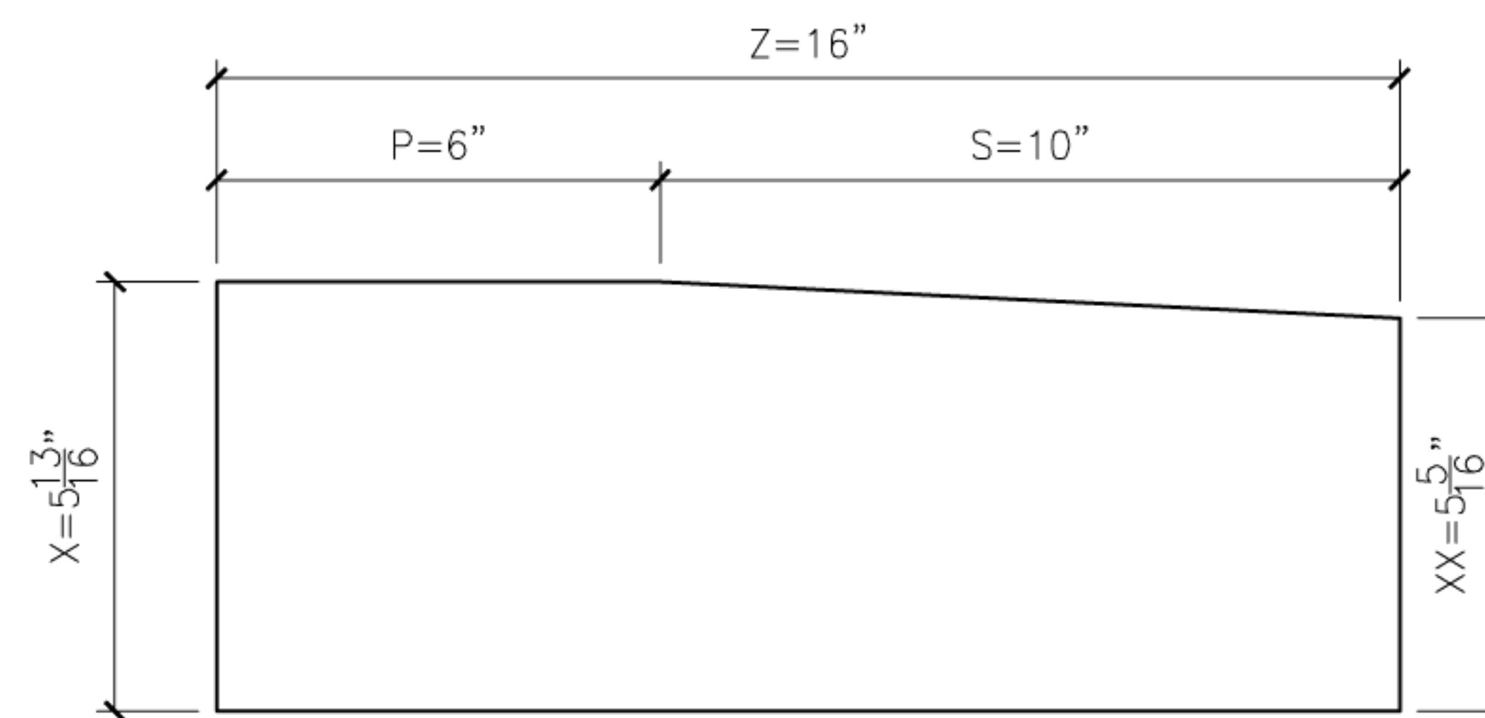
19 WEDGE19 PROFILE SECTION
