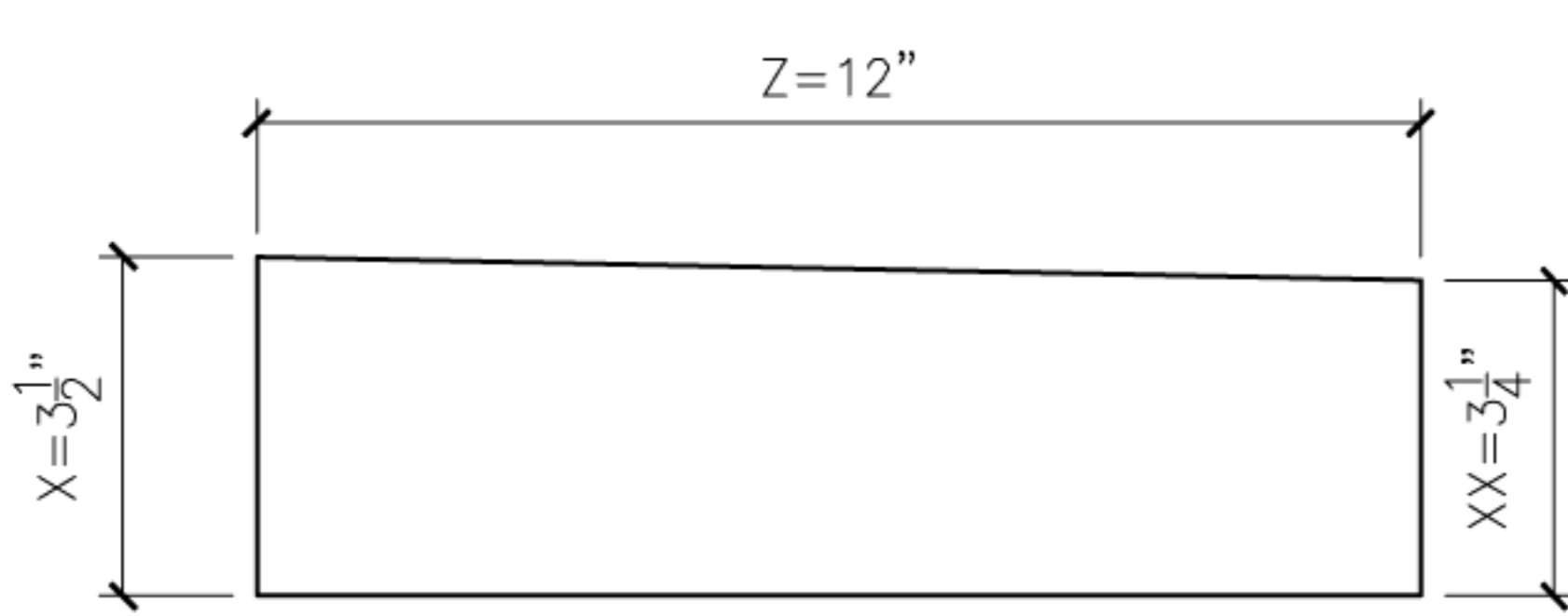
14 FLATFACE SLOPE15 PROFILE SECTION
