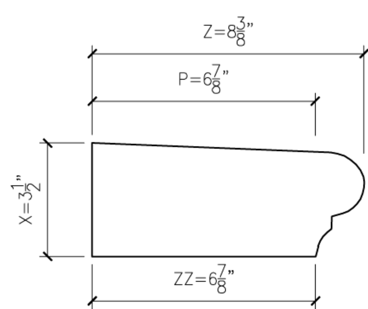
4 BOLSON4 PROFILE SECTION
