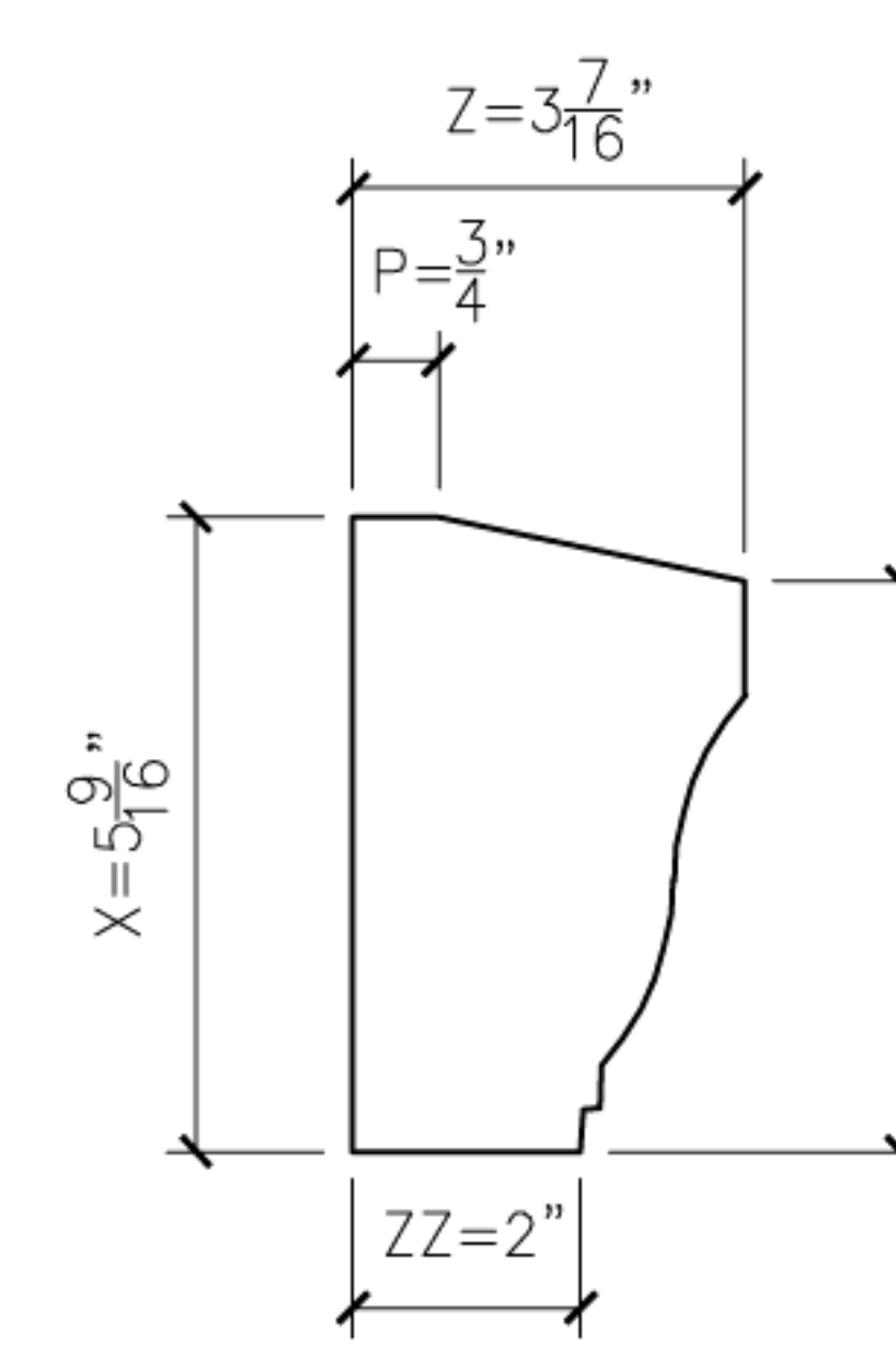
15 ORIEL15 PROFILE SECTION
