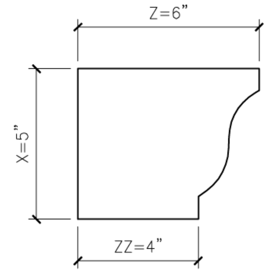
3A OGEE3A PROFILE SECTION
