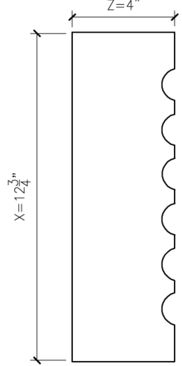
4 GEORGIAN4 PROFILE SECTION
