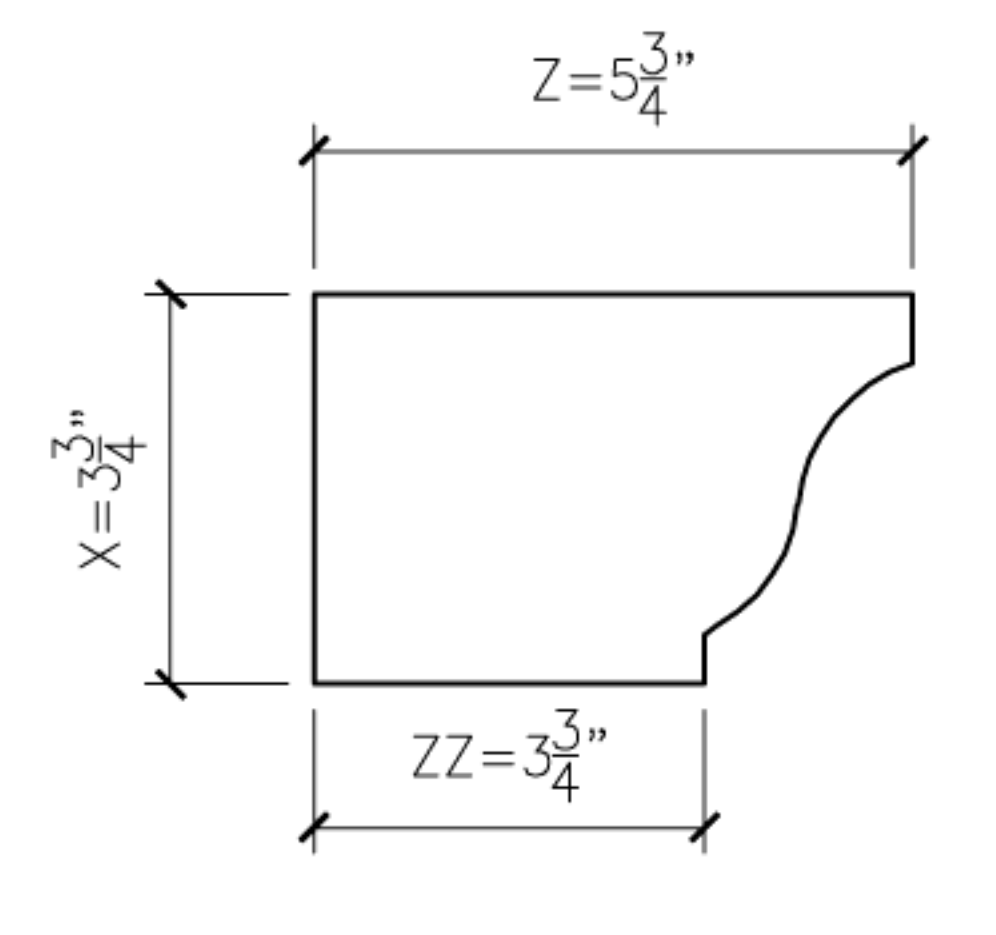
6 OGEE6 PROFILE SECTION
