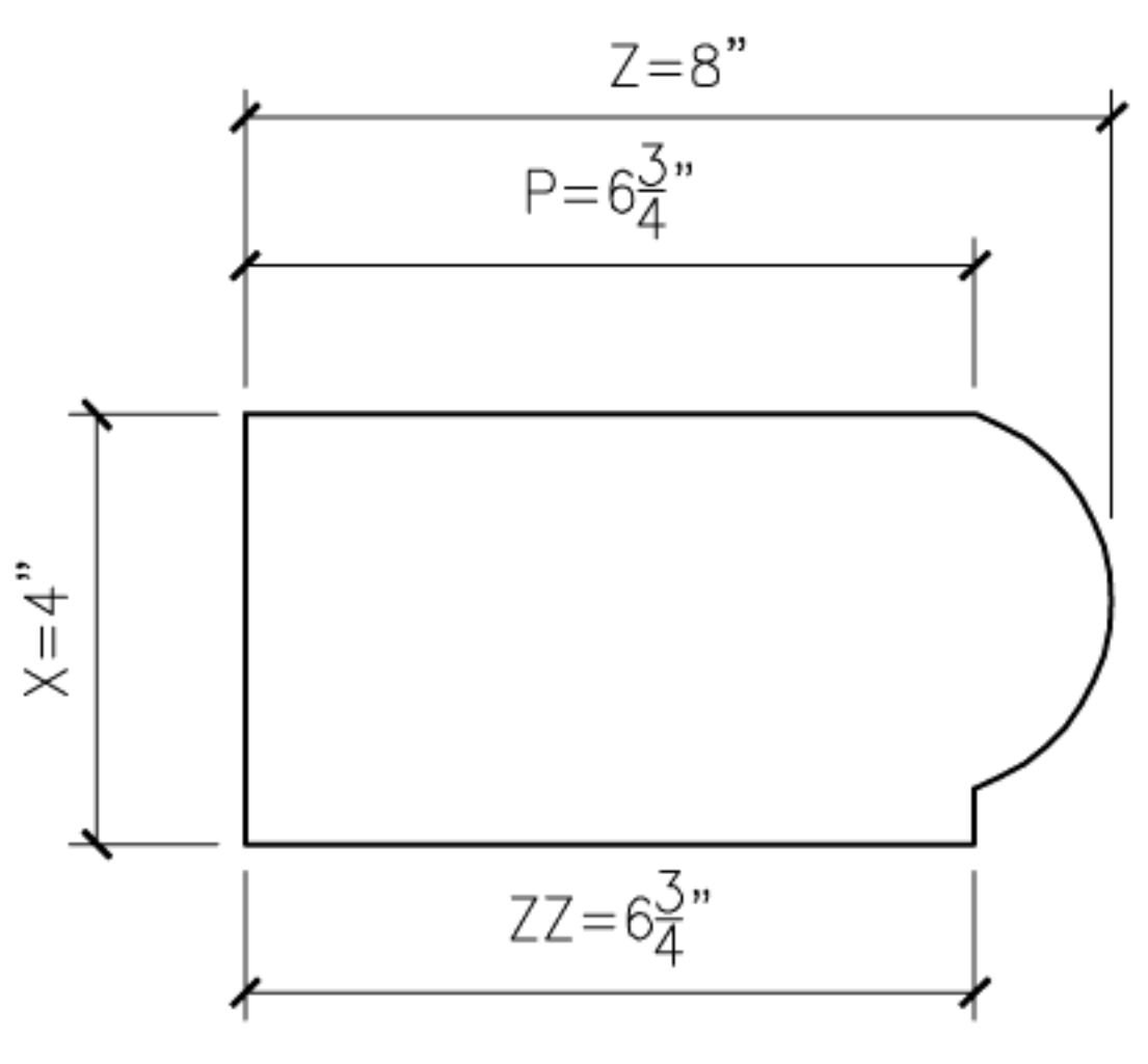
1 BULLNOSE1 PROFILE SECTION
