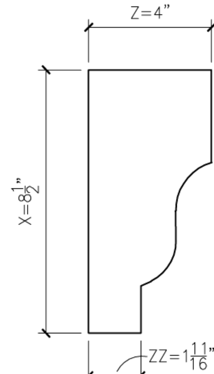
27 OGEE27 PROFILE SECTION
