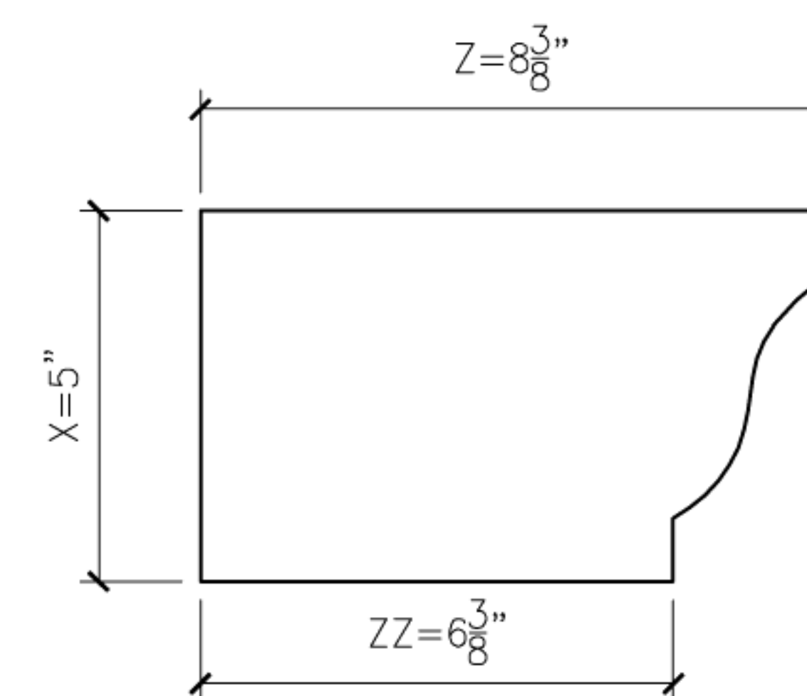
14B OGEE14B PROFILE SECTION
