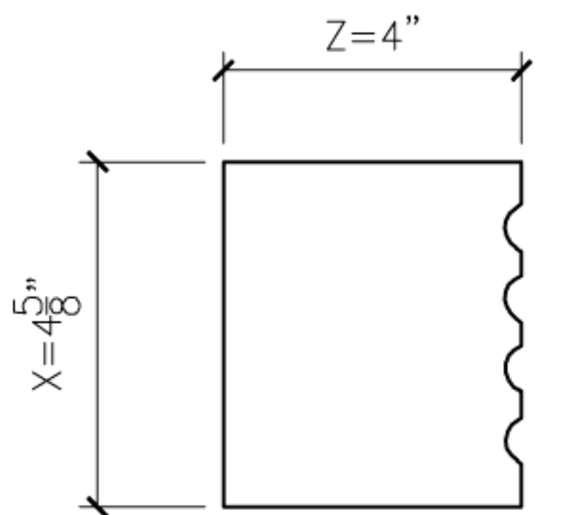
11 GEORGIAN11 PROFILE SECTION
