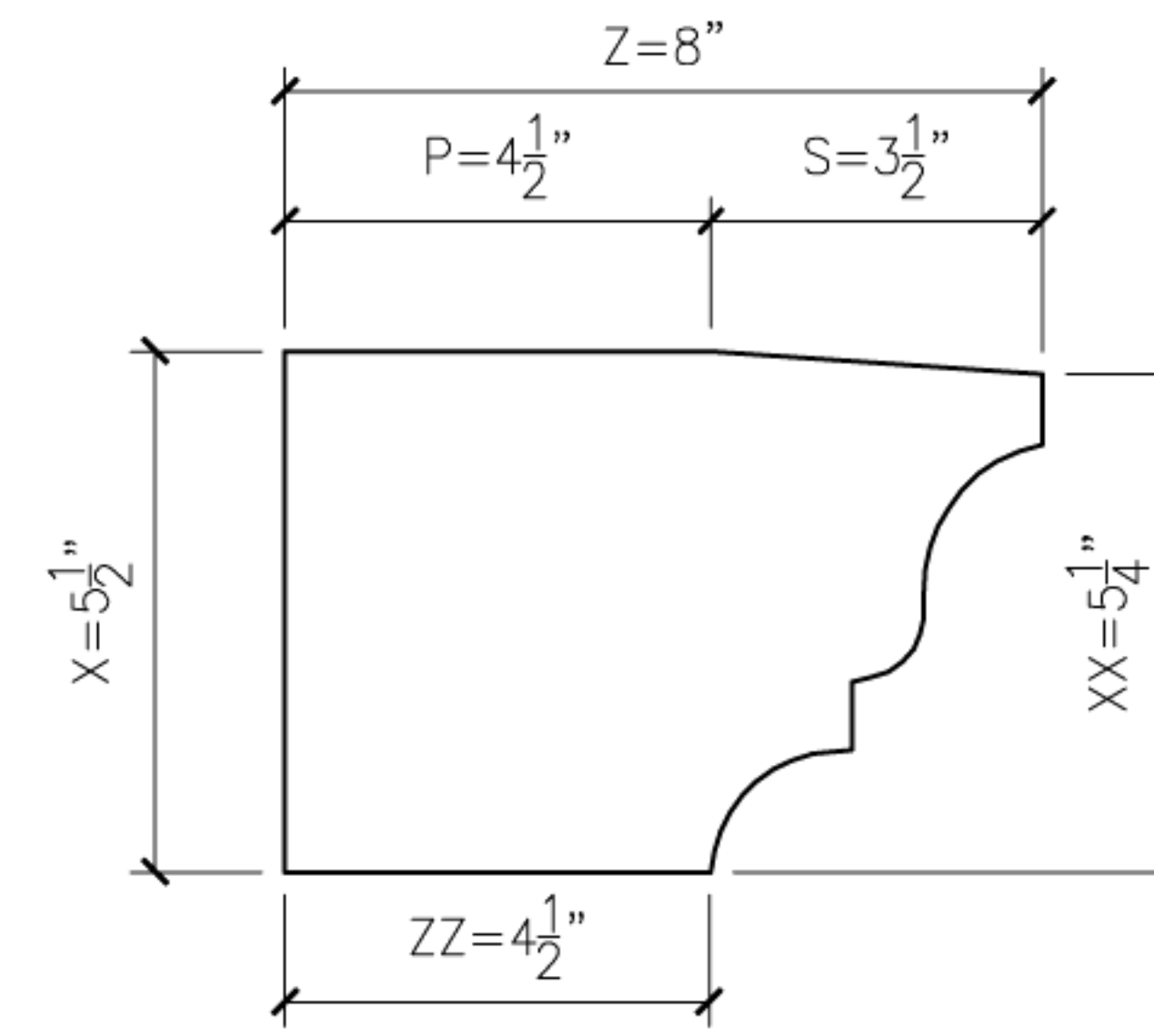
2 ORIEL2 PROFILE SECTION
