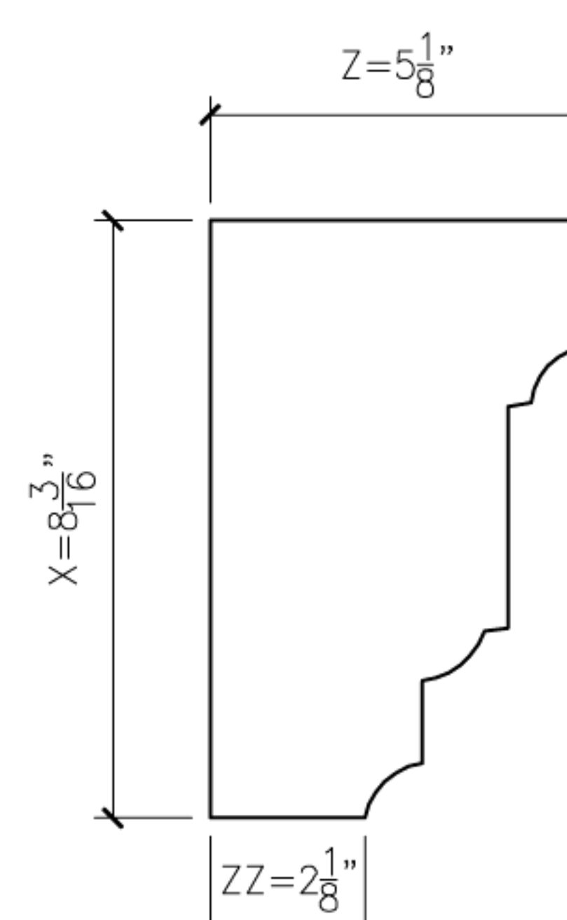
13 JAMISON13 PROFILE SECTION
