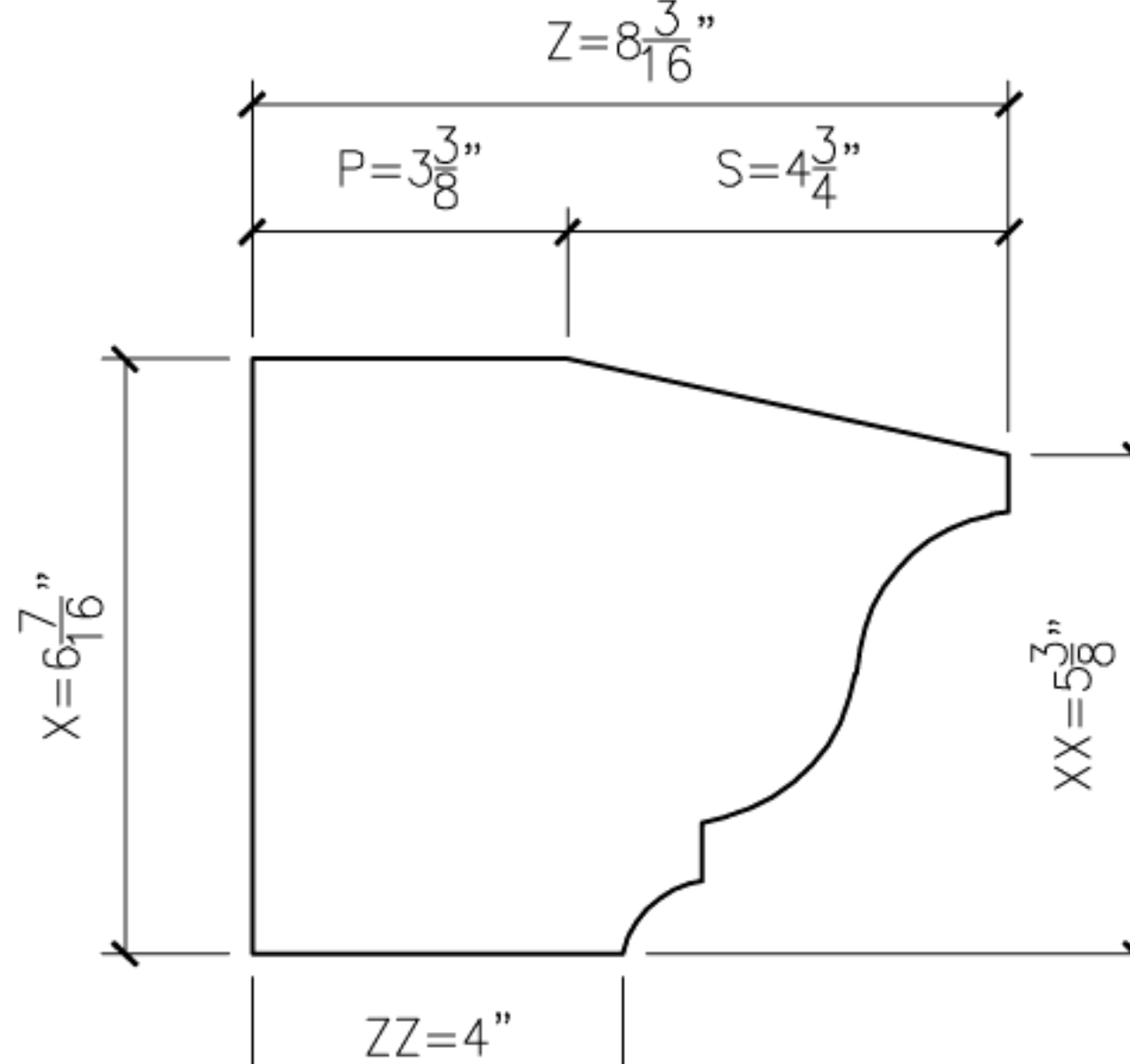
5 ORIEL5 PROFILE SECTION
