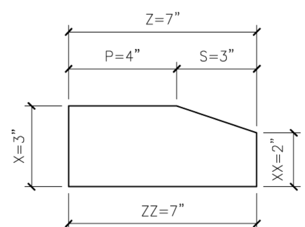
13 WEDGE13 PROFILE SECTION
