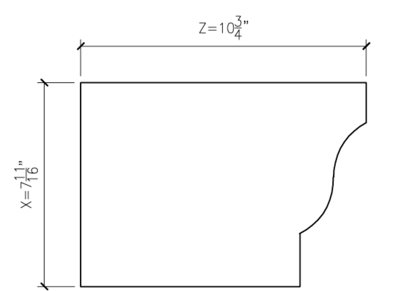
21 OGEE21 PROFILE SECTION
