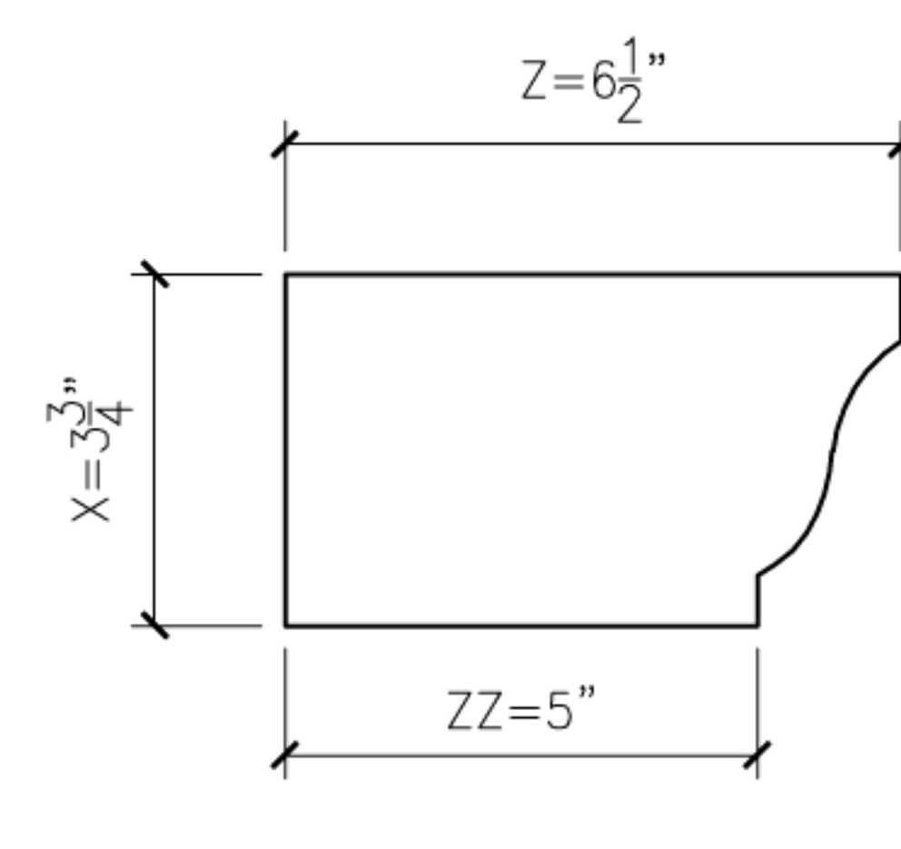
4 OGEE4 PROFILE SECTION
