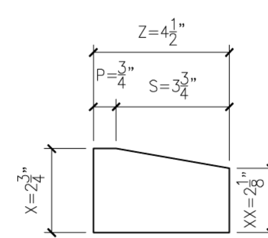
26 WEDGE26 PROFILE SECTION
