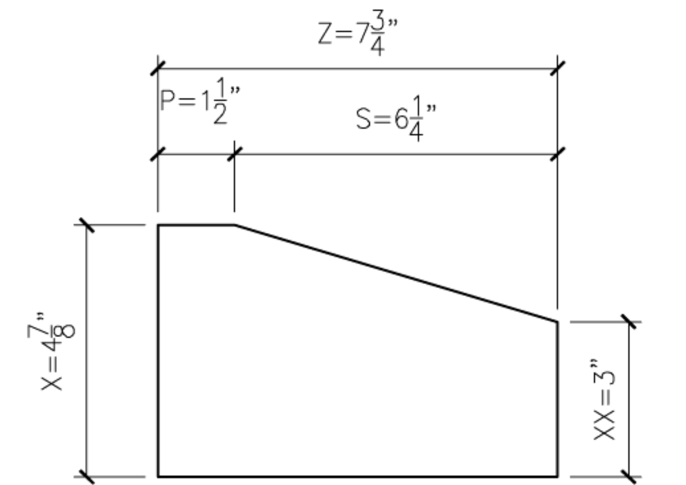
16 WEDGE16 PROFILE SECTION
