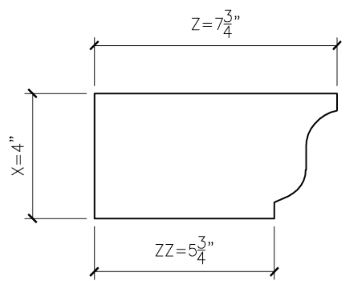
11 OGEE11 PROFILE SECTION
