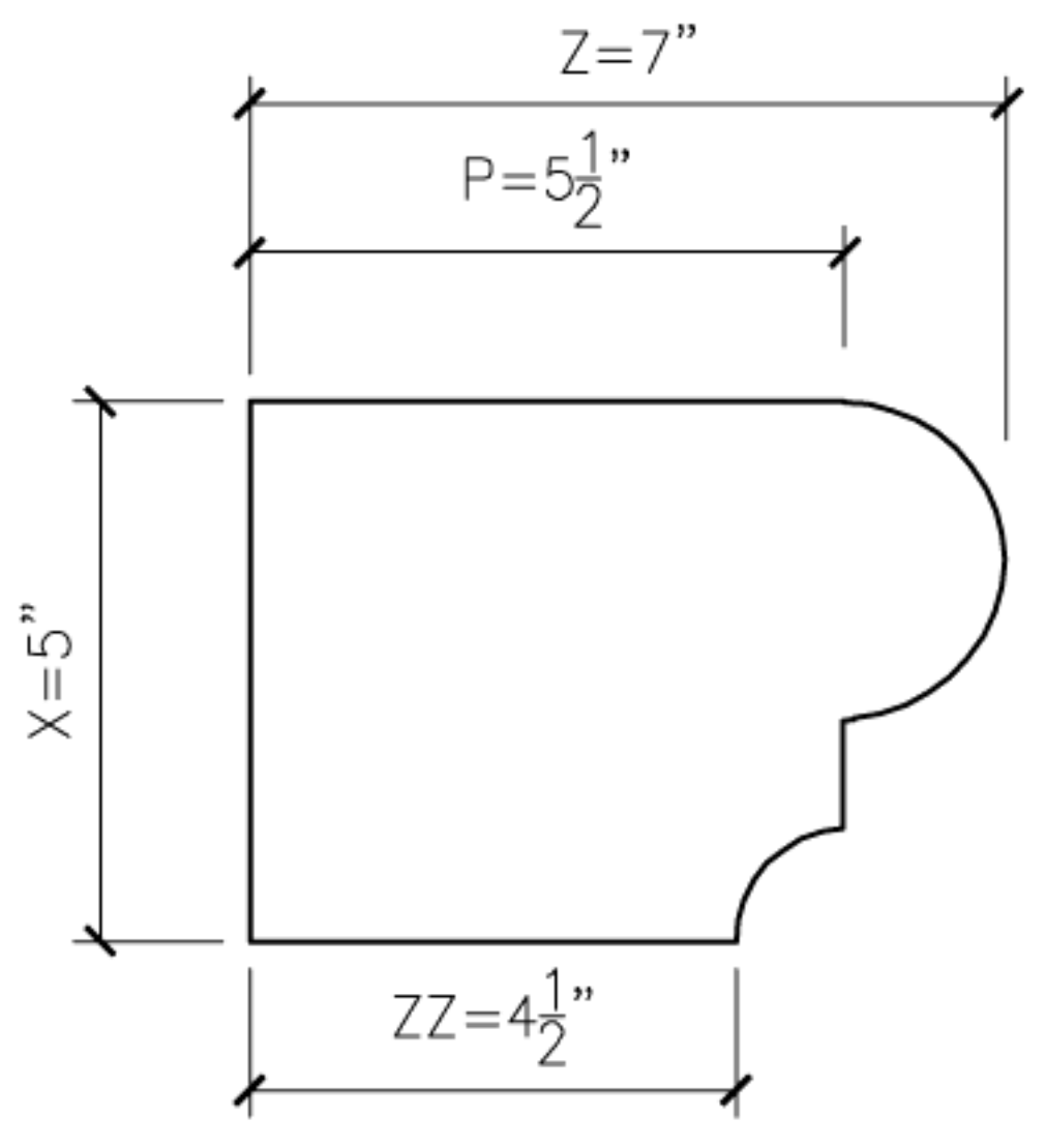
1 BOLSON1 PROFILE SECTION
