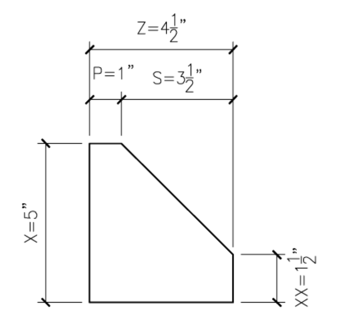
20 WEDGE20 PROFILE SECTION
