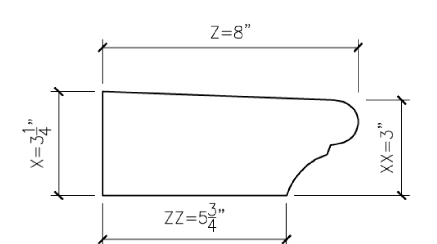
16 BOLSON16 PROFILE SECTION
