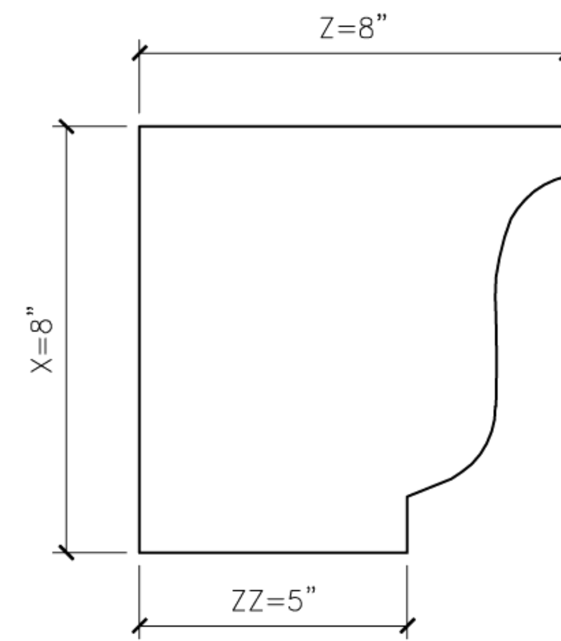
24 OGEE24 PROFILE SECTION
