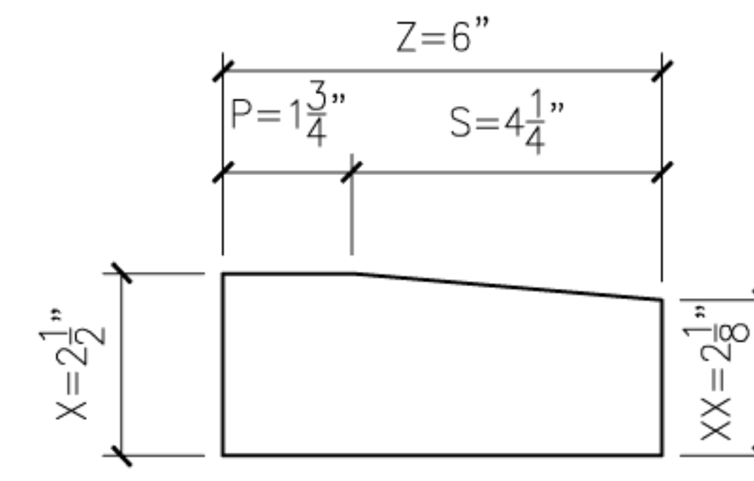
7 WEDGE7 PROFILE SECTION
