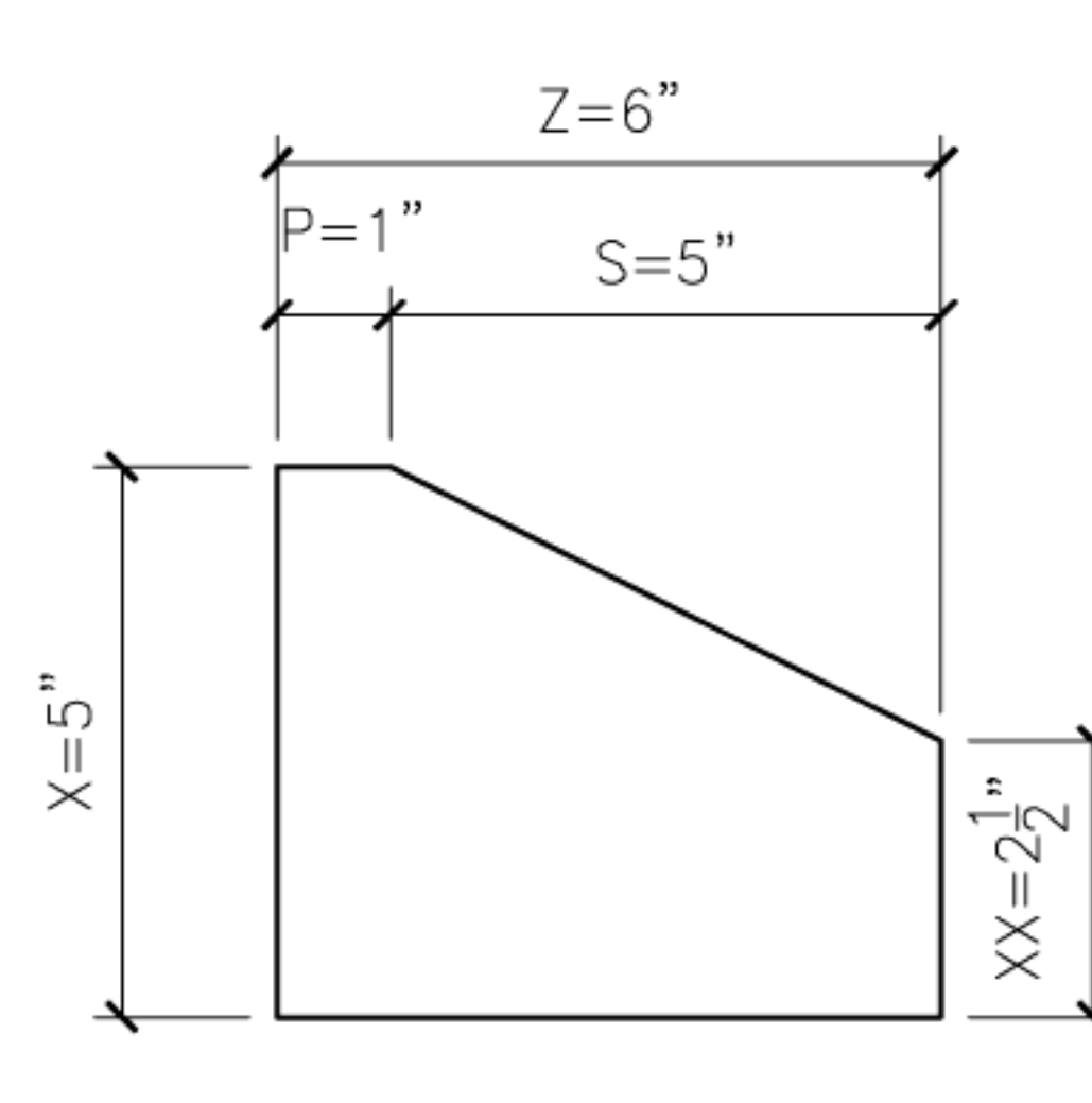
23 WEDGE23 PROFILE SECTION
