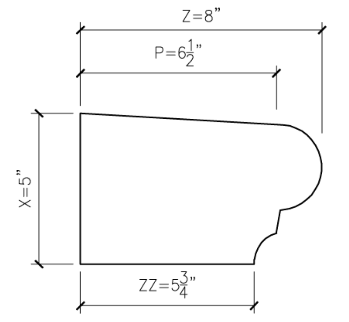
2A BOLSON2A PROFILE SECTION
