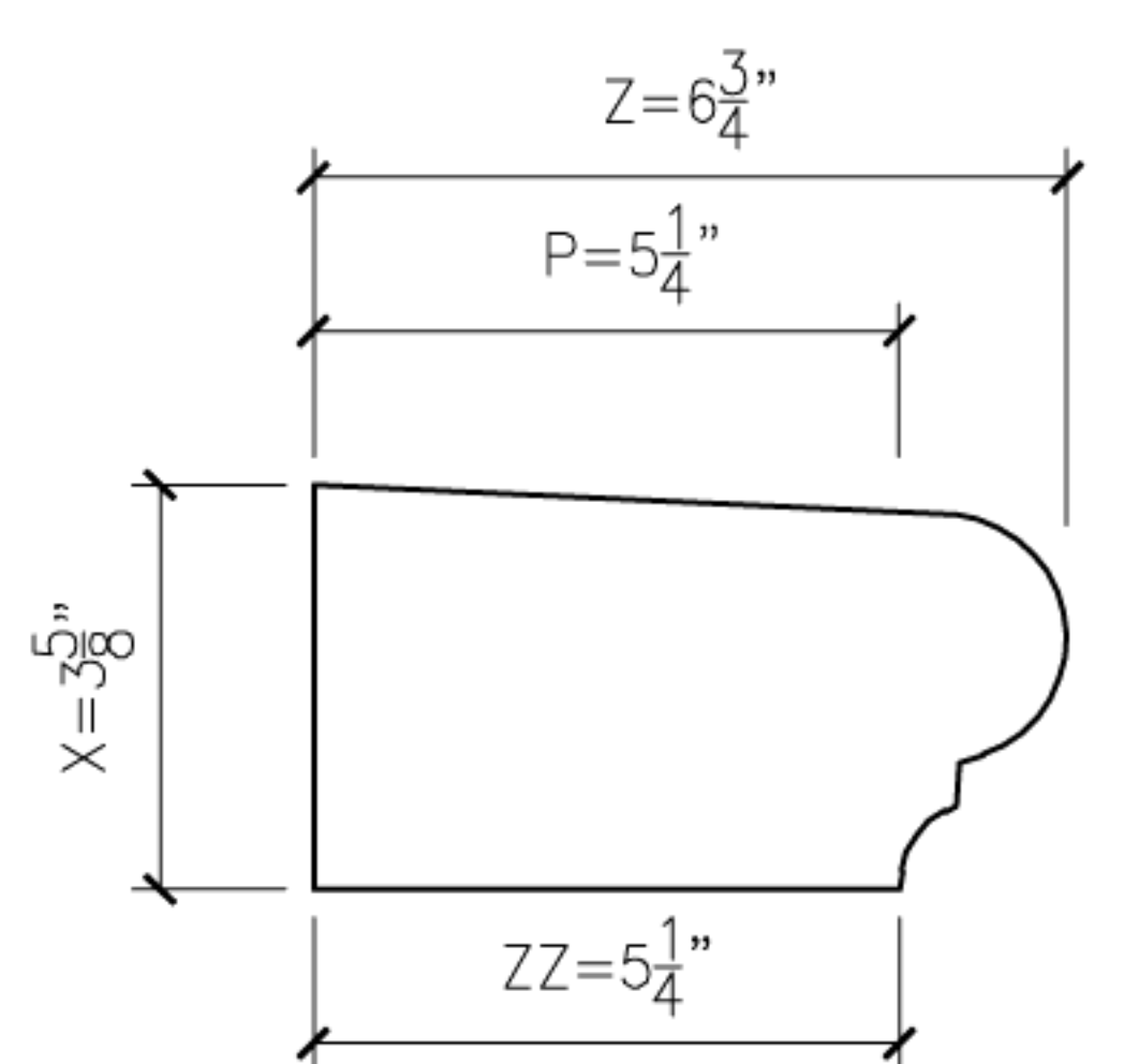
6A BOLSON6A PROFILE SECTION
