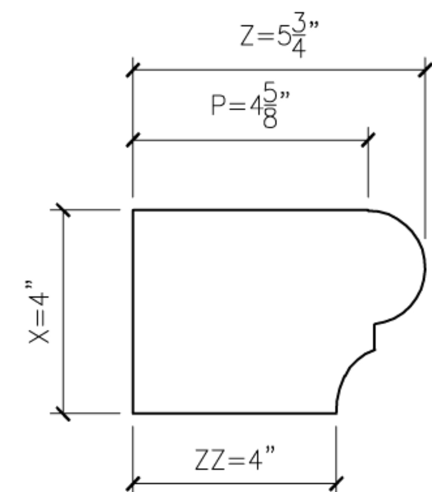
11 BOLSON11 PROFILE SECTION
