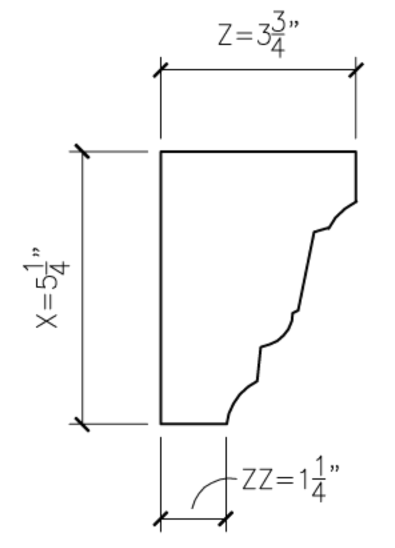
2A JAMISON2A PROFILE SECTION
