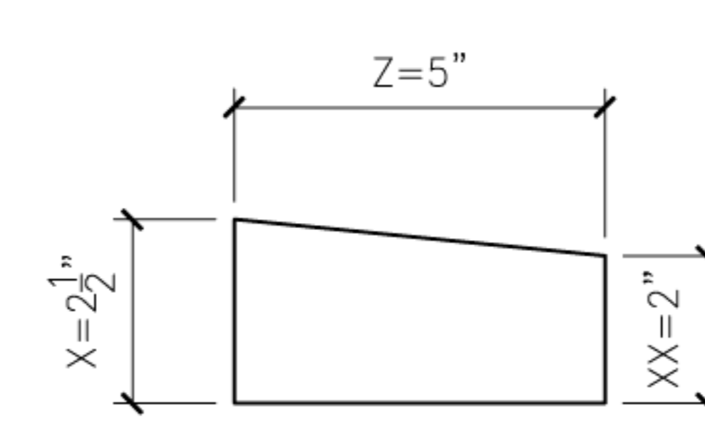
7 FLATFACE SLOPE8 PROFILE SECTION
