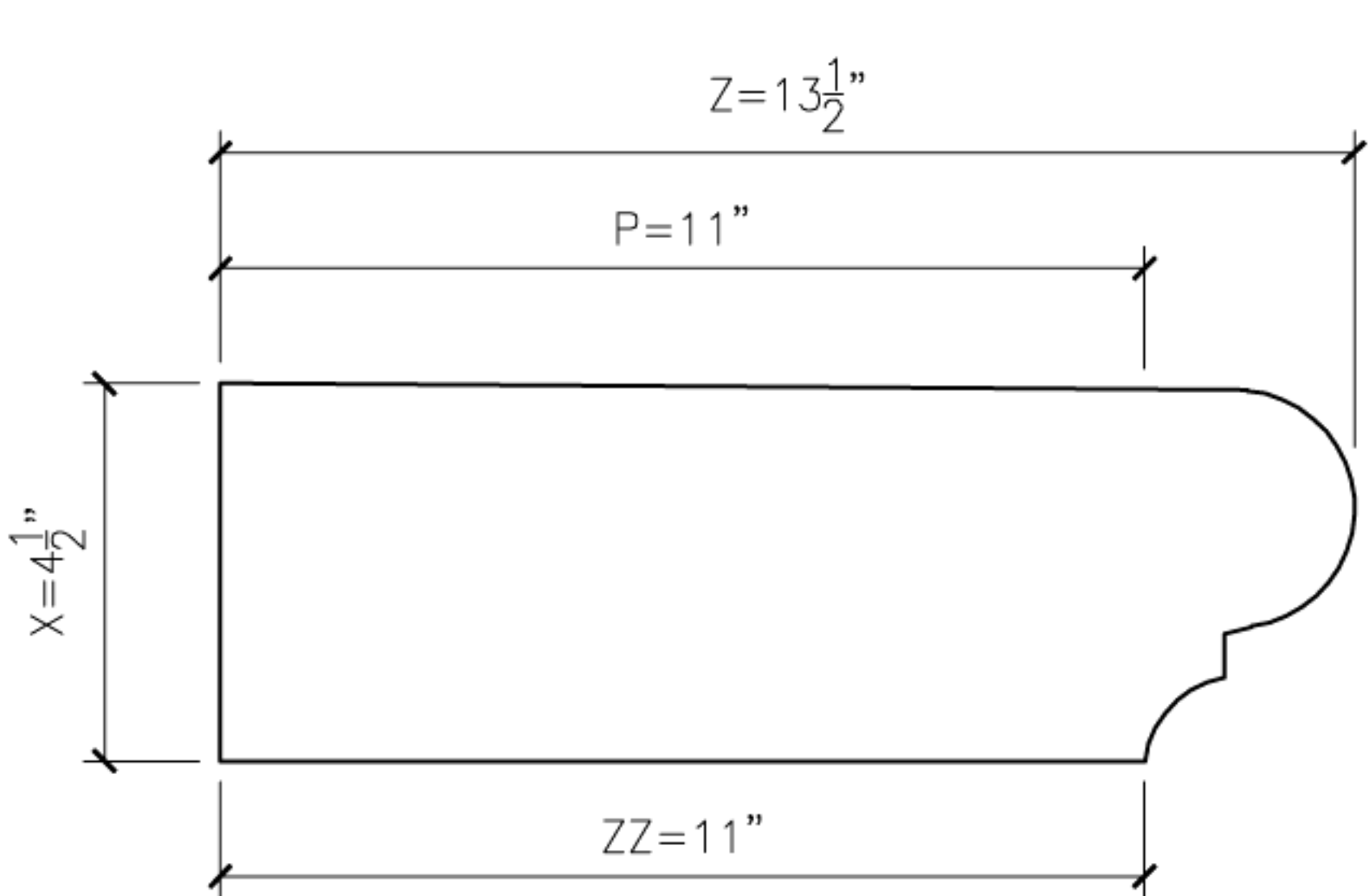
17 BOLSON17 PROFILE SECTION
