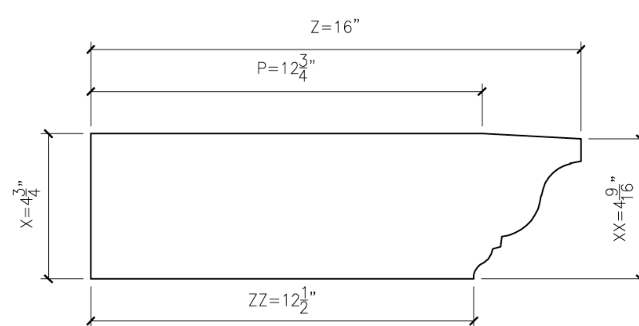
12 ORIEL12 PROFILE SECTION
