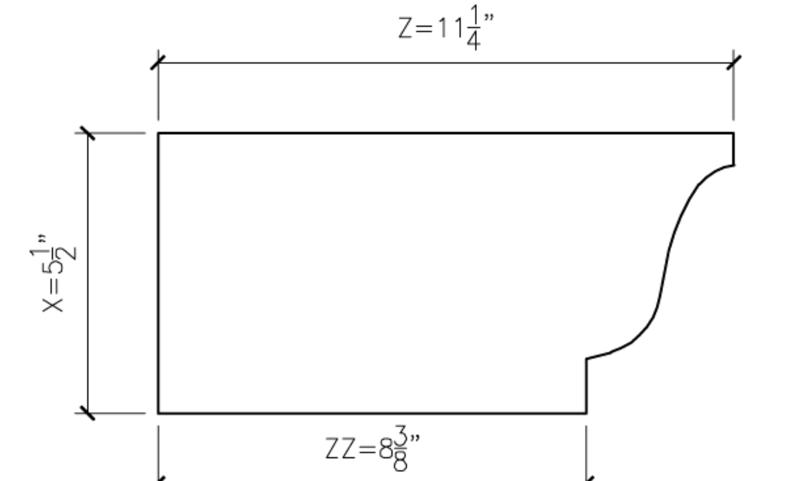
15 OGEE15 PROFILE SECTION
