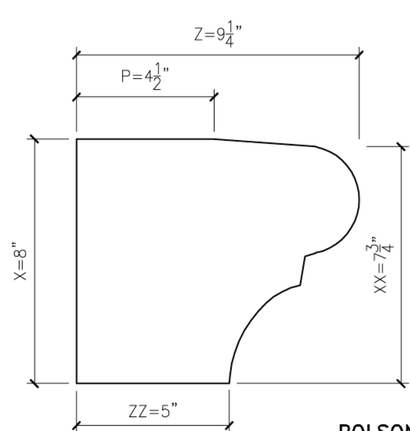
14A BOLSON14A PROFILE SECTION
