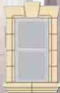
SurroundWindow
