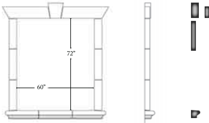
Cross Sections
