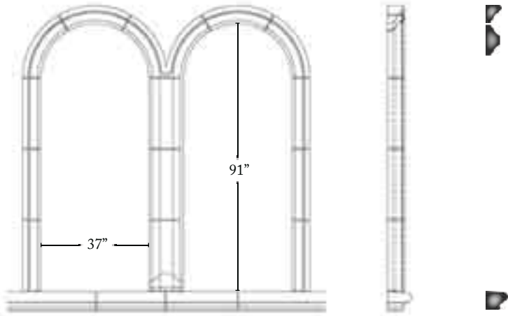
Cross Sections
