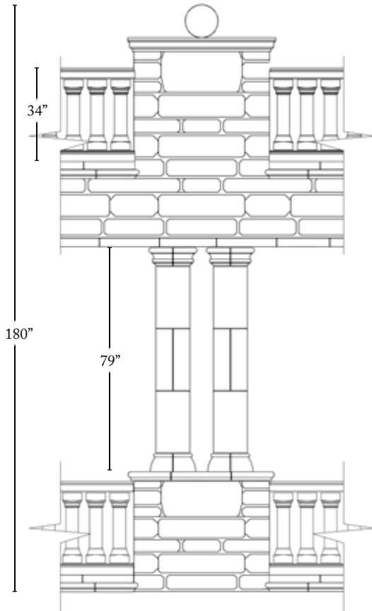
Front View
