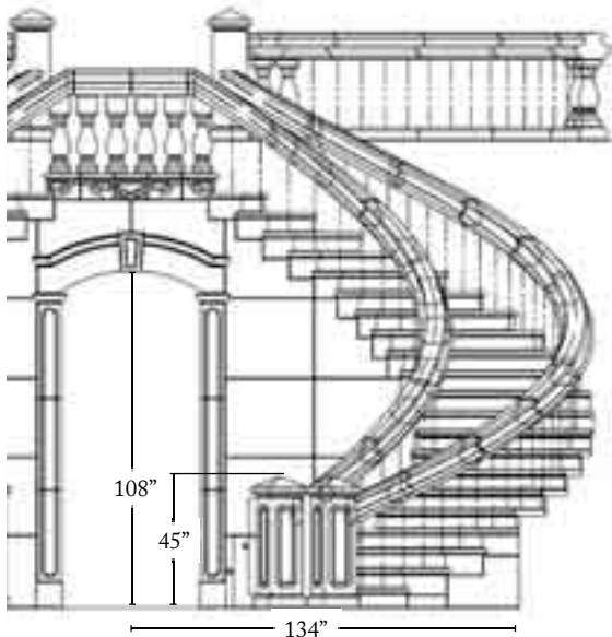
Complete Staircase
