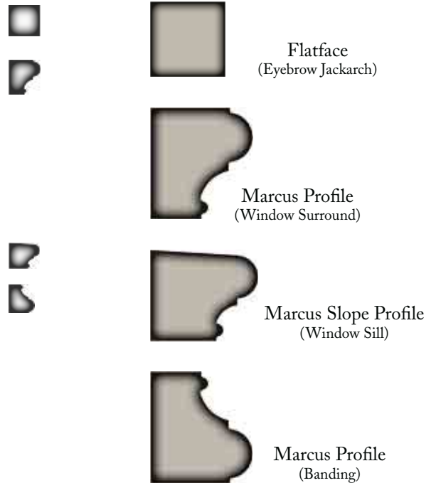
Cross Section
