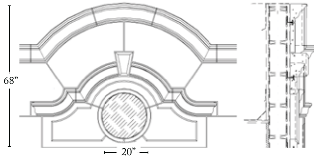
Cross Section
