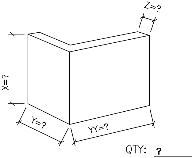
① ISOMETRIC VIEW QUOIN ONE PIECE
